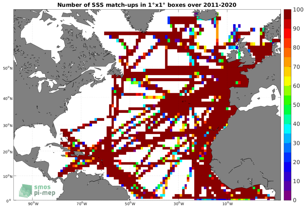
Figure 4: Number of SSS match-ups between TSG (GOSUD-Research-vessel) SSS and the SMOS SSS L4 v2 - Daily (BEC) SSS product for the North Atlantic Ocean Pi-MEP region over 1^\circ \times 1^\circ boxes and for the full satellite product period.
