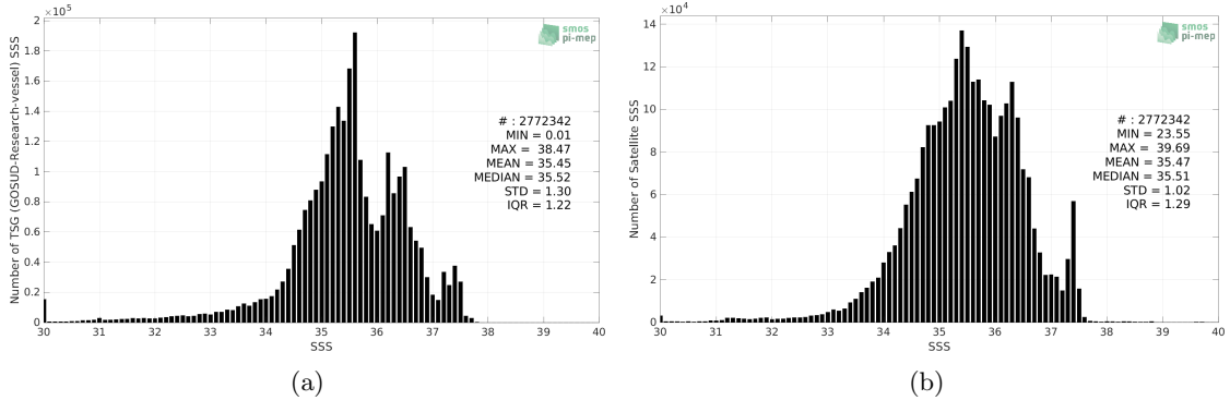
Figure 2: Histograms of SSS from TSG (GOSUD-Research-vessel) (a) and SMOS SSS L4 v2 - Daily (BEC) (b) considering all match-up pairs per bins of 0.1 over the North Atlantic Ocean Pi-MEP region and for the full satellite product period.
