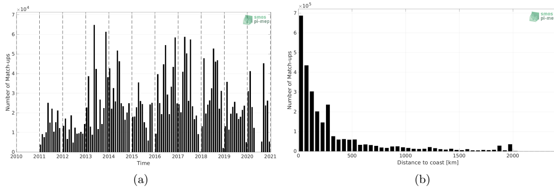
Figure 1: Number of match-ups between TSG (GOSUD-Research-vessel) and SMOS SSS L4 v2 - Daily (BEC) SSS as a function of time (a) and as function of the distance to coast (b) over the North Atlantic Ocean Pi-MEP region and for the full satellite product period.
