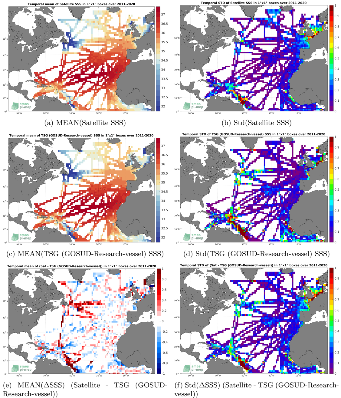
Figure 6: Temporal mean (left) and Std (right) of SSS from SMOS SSS L4 v2 - Daily (BEC) (top), TSG (GOSUD-Research-vessel) (middle), and of \Delta SSS (Satellite - TSG (GOSUD-Research-vessel)). Only match-up pairs are used to generate these maps.
