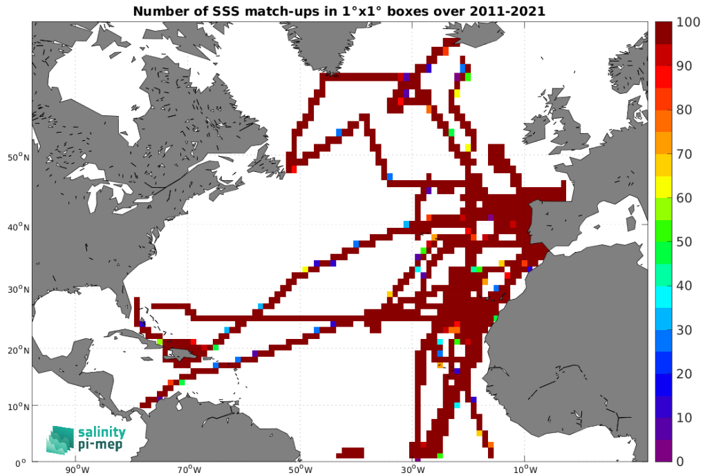
Figure 5: Number of SSS match-ups between TSG (CSIC-UTM) SSS and the SMOS SSS L4 v2 - Daily (BEC) SSS product for the North Atlantic Ocean Pi-MEP region over 1^\circ \times 1^\circ boxes and for the full satellite product period.
