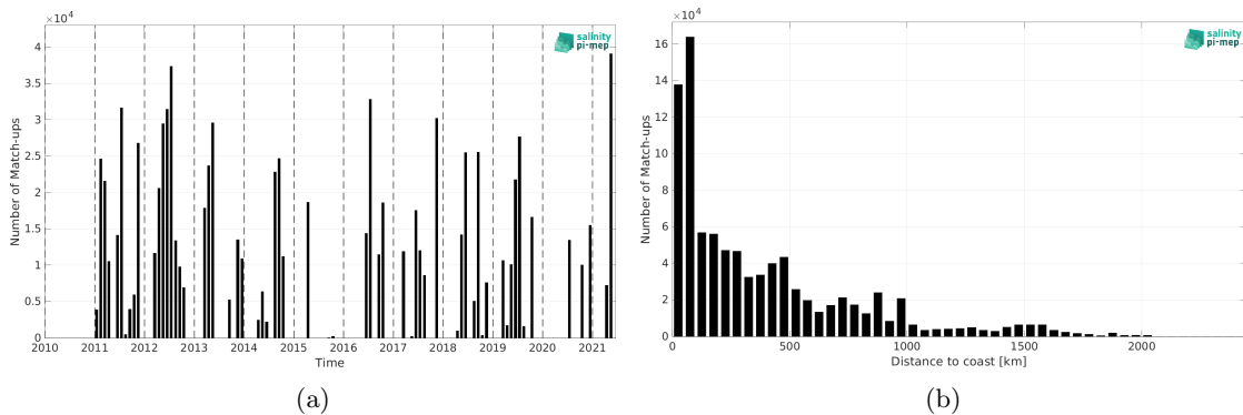
Figure 2: Number of match-ups between TSG (CSIC-UTM) and SMOS SSS L4 v2 - Daily (BEC) SSS as a function of time (a) and as function of the distance to coast (b) over the North Atlantic Ocean Pi-MEP region and for the full satellite product period.
