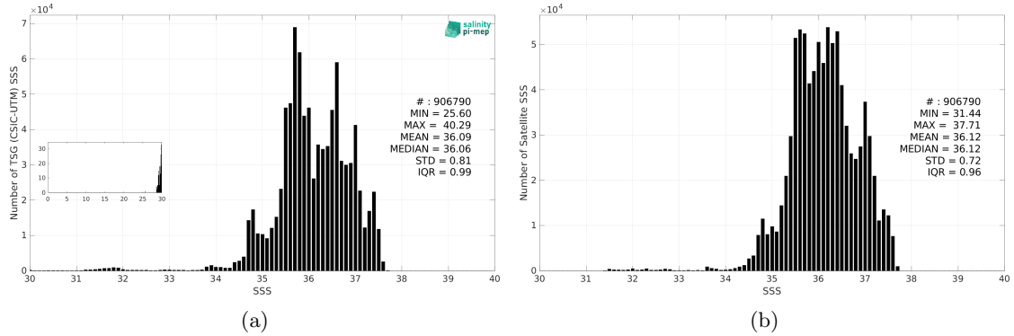
Figure 3: Histograms of SSS from TSG (CSIC-UTM) (a) and SMOS SSS L4 v2 - Daily (BEC) (b) considering all match-up pairs per bins of 0.1 over the North Atlantic Ocean Pi-MEP region and for the full satellite product period.
