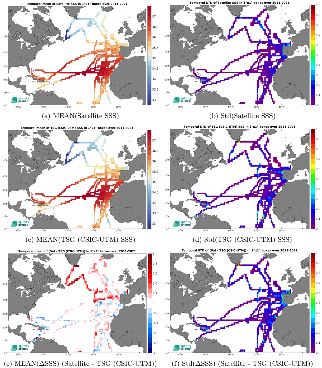
Figure 7: Temporal mean (left) and Std (right) of SSS from SMOS SSS L4 v2 - Daily (BEC) (top), TSG (CSIC-UTM) (middle), and of \Delta SSS (Satellite - TSG (CSIC-UTM)). Only match-up pairs are used to generate these maps.
