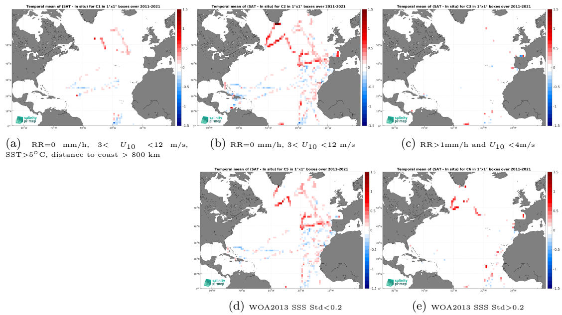
Figure 14: Temporal mean gridded over spatial boxes of size 1^\circ \times 1^\circ of \Delta\text{SSS} (SMOS SSS L4 v2 - Daily (BEC) - TSG (CSIC-UTM)) for 5 different subdatasets corresponding to: RR=0 mm/h, 3 < U_{10} < 12 m/s, SST > 5^\circ\text{C} , distance to coast > 800 km (a), RR=0 mm/h, 3 < U_{10} < 12 m/s (b), RR > 1 mm/h and U_{10} < 4 m/s (c), WOA2013 SSS Std < 0.2 (d), WOA2013 SSS Std > 0.2 (e).
