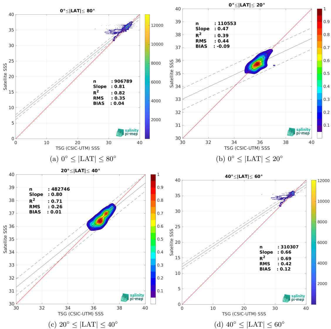
Figure 10: Contour maps of the concentration of SMOS SSS L4 v2 - Daily (BEC) SSS (y-axis) versus TSG (CSIC-UTM) SSS (x-axis) at match-up pairs for different latitude bands. For each plot, the red line shows x=y . The black thin and dashed lines indicate a linear fit through the data cloud and the \pm 95\% confidence levels, respectively. The number match-up pairs n , the slope and R^2 coefficient of the linear fit, the root mean square (RMS) and the mean bias between satellite and in situ data are indicated for each latitude band in each plots.
