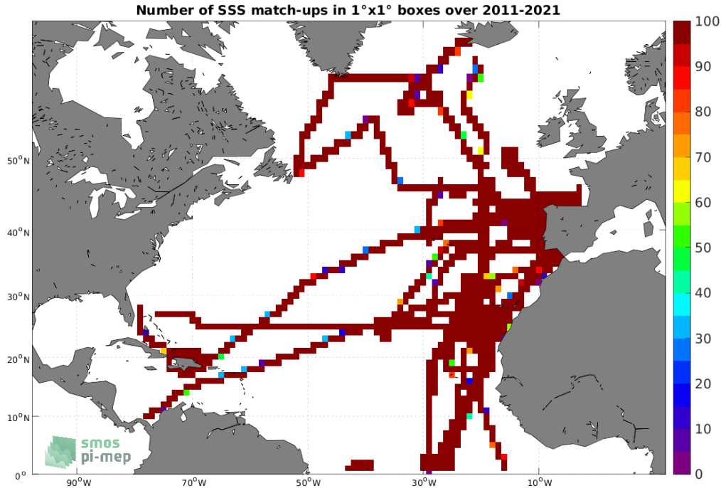
Figure 4: Number of SSS match-ups between TSG (CSIC-UTM) SSS and the SMOS SSS L4 v2 - Daily (BEC) SSS product for the North Atlantic Ocean Pi-MEP region over 1^\circ \times 1^\circ boxes and for the full satellite product period.
