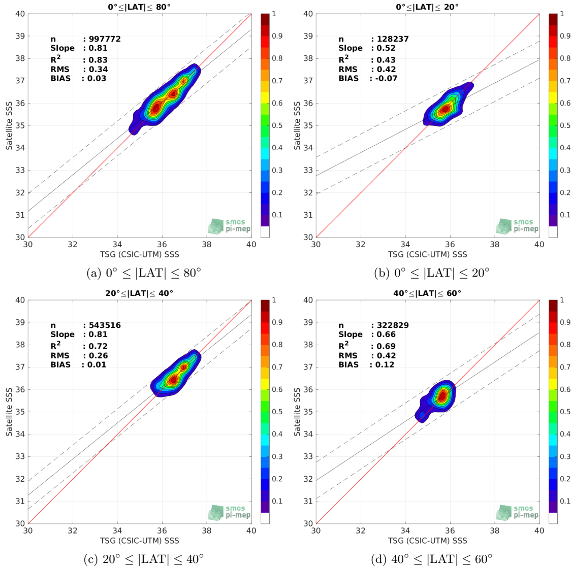
Figure 9: Contour maps of the concentration of SMOS SSS L4 v2 - Daily (BEC) SSS (y-axis) versus TSG (CSIC-UTM) SSS (x-axis) at match-up pairs for different latitude bands. For each plot, the red line shows x=y . The black thin and dashed lines indicate a linear fit through the data cloud and the \pm 95\% confidence levels, respectively. The number match-up pairs n , the slope and R^2 coefficient of the linear fit, the root mean square (RMS) and the mean bias between satellite and in situ data are indicated for each latitude band in each plots.
