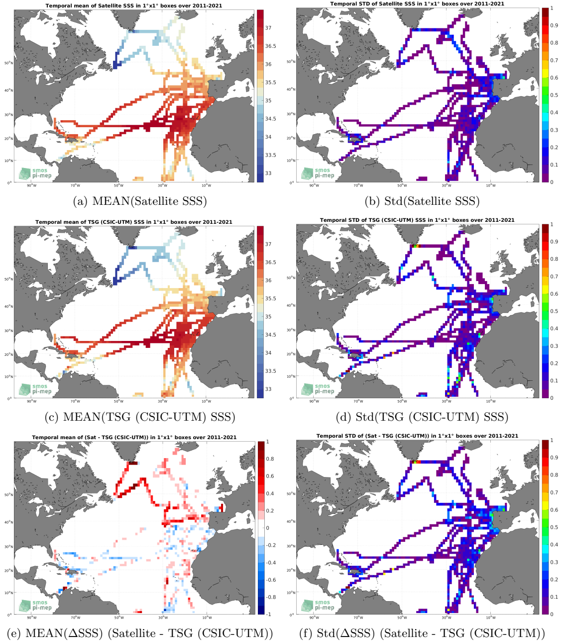
Figure 6: Temporal mean (left) and Std (right) of SSS from SMOS SSS L4 v2 - Daily (BEC) (top), TSG (CSIC-UTM) (middle), and of \Delta SSS (Satellite - TSG (CSIC-UTM)). Only match-up pairs are used to generate these maps.
