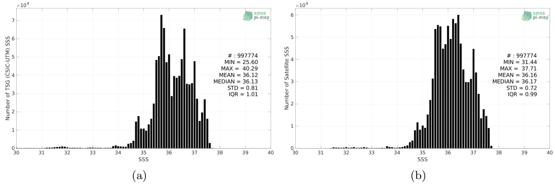
Figure 2: Histograms of SSS from TSG (CSIC-UTM) (a) and SMOS SSS L4 v2 - Daily (BEC) (b) considering all match-up pairs per bins of 0.1 over the North Atlantic Ocean Pi-MEP region and for the full satellite product period.
