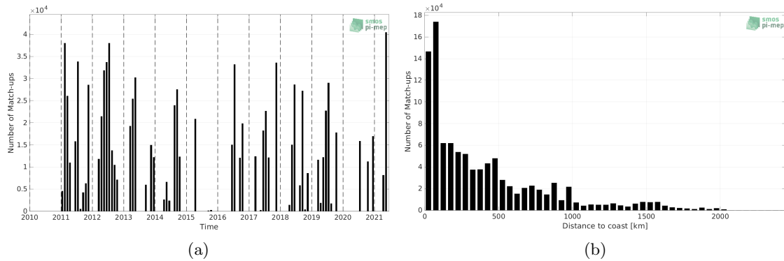
Figure 1: Number of match-ups between TSG (CSIC-UTM) and SMOS SSS L4 v2 - Daily (BEC) SSS as a function of time (a) and as function of the distance to coast (b) over the North Atlantic Ocean Pi-MEP region and for the full satellite product period.
