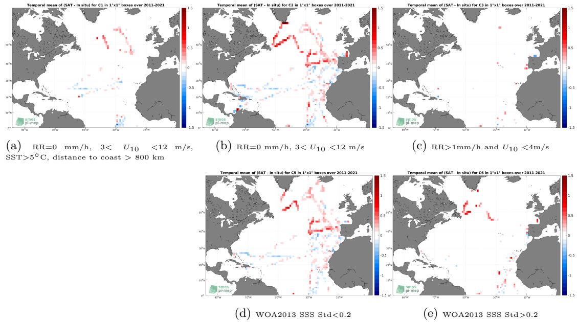
Figure 12: Temporal mean gridded over spatial boxes of size 1^\circ \times 1^\circ of \Delta SSS (SMOS SSS L4 v2 - Daily (BEC) - TSG (CSIC-UTM)) for 5 different subdatasets corresponding to:RR=0 mm/h, 3 < U_{10} < 12 m/s, SST >5^\circ\text{C} , distance to coast > 800 km (a), RR=0 mm/h, 3 < U_{10} < 12 m/s (b), RR >1 mm/h and U_{10} < 4 m/s (c), WOA2013 SSS Std <0.2 (d), WOA2013 SSS Std >0.2 (e).
