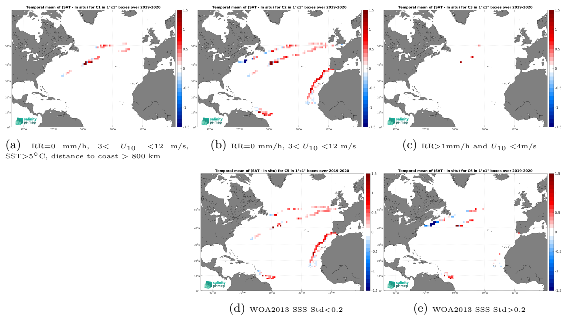
Figure 14: Temporal mean gridded over spatial boxes of size 1^\circ \times 1^\circ of \Delta\text{SSS} (SMOS SSS L4 v2 - Daily (BEC) - Saifdrone) for 5 different subdatasets corresponding to:RR=0 mm/h, 3 < U_{10} < 12 m/s, SST >5^\circ\text{C} , distance to coast > 800 km (a), RR=0 mm/h, 3 < U_{10} < 12 m/s (b), RR >1 mm/h and U_{10} < 4 m/s (c), WOA2013 SSS Std <0.2 (d), WOA2013 SSS Std >0.2 (e).
