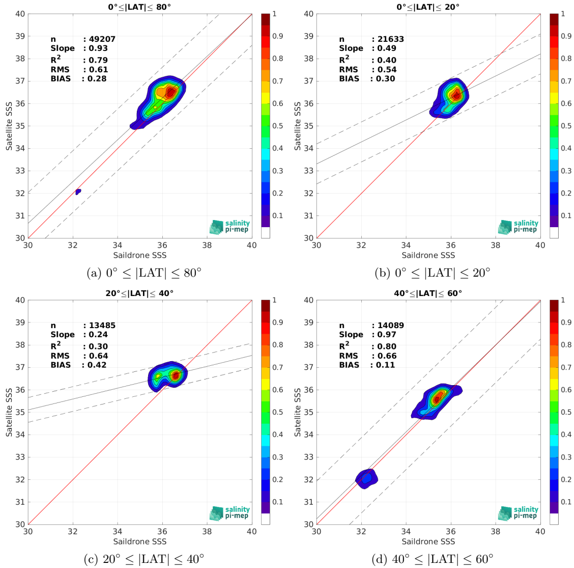
Figure 10: Contour maps of the concentration of SMOS SSS L4 v2 - Daily (BEC) SSS (y-axis) versus Saildrone SSS (x-axis) at match-up pairs for different latitude bands. For each plot, the red line shows x=y . The black thin and dashed lines indicate a linear fit through the data cloud and the \pm 95\% confidence levels, respectively. The number match-up pairs n , the slope and R^2 coefficient of the linear fit, the root mean square (RMS) and the mean bias between satellite and in situ data are indicated for each latitude band in each plots.
