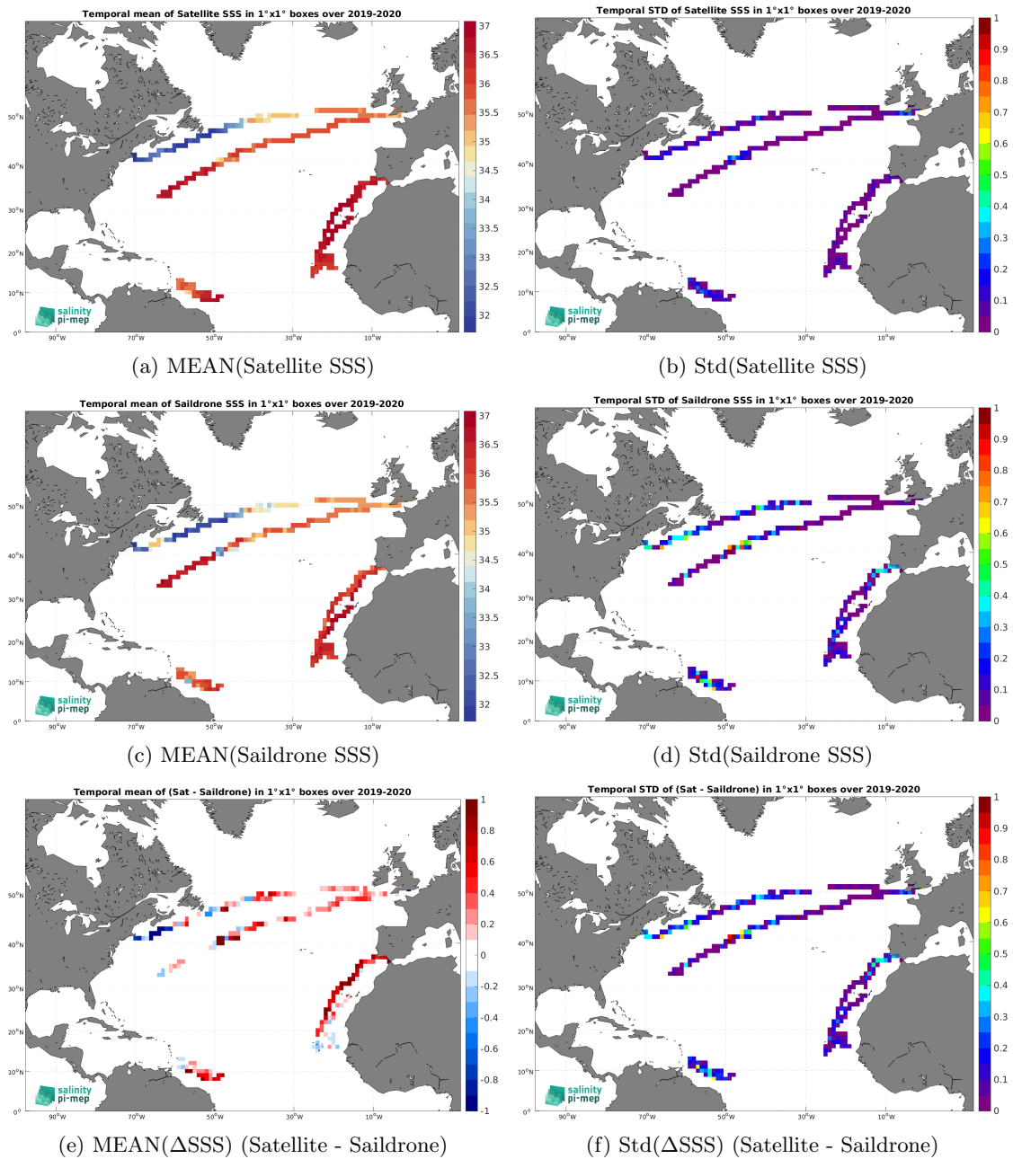
Figure 7: Temporal mean (left) and Std (right) of SSS from SMOS SSS L4 v2 - Daily (BEC) (top), Saildrone (middle), and of \Delta SSS (Satellite - Saildrone). Only match-up pairs are used to generate these maps.
