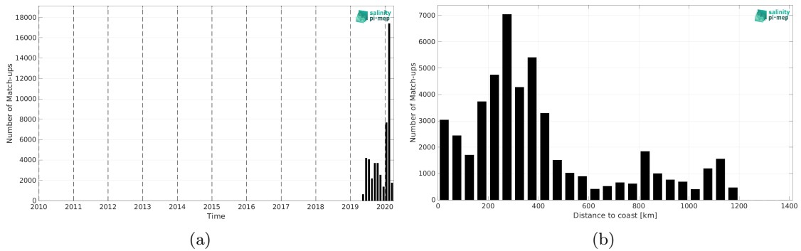
Figure 2: Number of match-ups between Saildrone and SMOS SSS L4 v2 - Daily (BEC) SSS as a function of time (a) and as function of the distance to coast (b) over the North Atlantic Ocean Pi-MEP region and for the full satellite product period.
