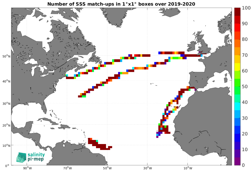
Figure 5: Number of SSS match-ups between Saildrone SSS and the SMOS SSS L4 v2 - Daily (BEC) SSS product for the North Atlantic Ocean Pi-MEP region over 1^\circ \times 1^\circ boxes and for the full satellite product period.
