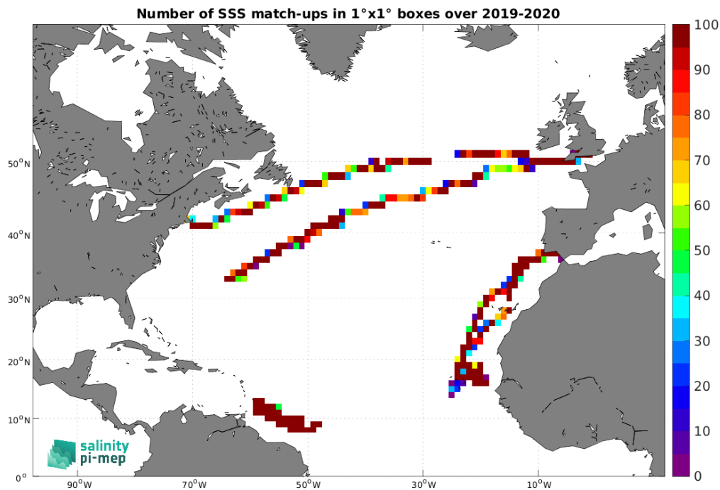
Figure 4: Number of SSS match-ups between Saildrone SSS and the SMOS SSS L4 v2 - Daily (BEC) SSS product for the North Atlantic Ocean Pi-MEP region over 1^\circ \times 1^\circ boxes and for the full satellite product period.
