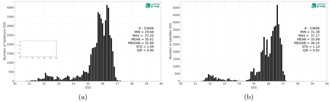
Figure 2: Histograms of SSS from Saildrone (a) and SMOS SSS L4 v2 - Daily (BEC) (b) considering all match-up pairs per bins of 0.1 over the North Atlantic Ocean Pi-MEP region and for the full satellite product period.
