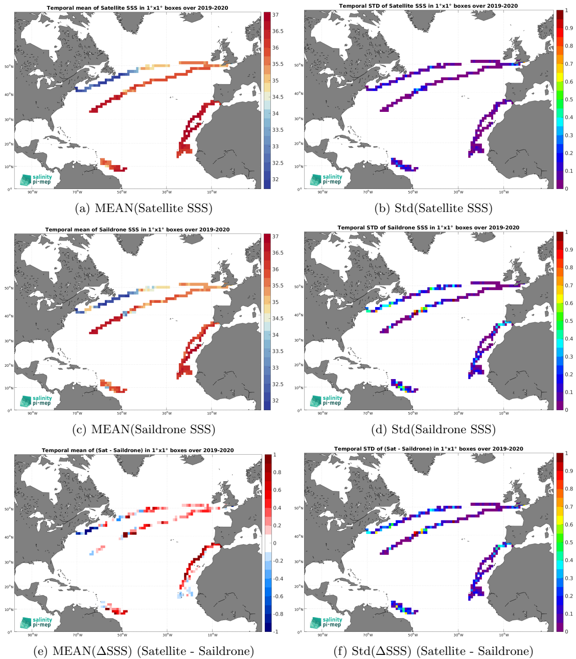
Figure 6: Temporal mean (left) and Std (right) of SSS from SMOS SSS L4 v2 - Daily (BEC) (top), Saildrone (middle), and of \Delta SSS (Satellite - Saildrone). Only match-up pairs are used to generate these maps.
