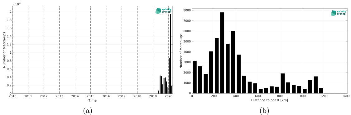
Figure 1: Number of match-ups between Saildrone and SMOS SSS L4 v2 - Daily (BEC) SSS as a function of time (a) and as function of the distance to coast (b) over the North Atlantic Ocean Pi-MEP region and for the full satellite product period.
