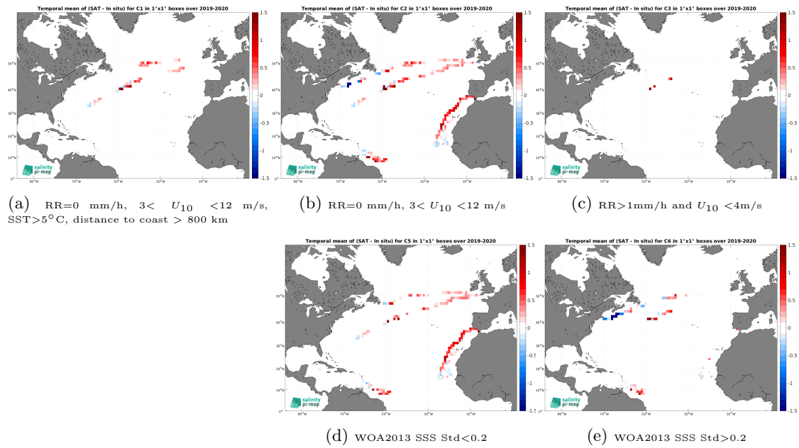
Figure 12: Temporal mean gridded over spatial boxes of size 1^\circ \times 1^\circ of \Delta\text{SSS} (SMOS SSS L4 v2 - Daily (BEC) - Saifdrone) for 5 different subdatasets corresponding to:RR=0 mm/h, 3 < U_{10} < 12 m/s, SST >5^\circ\text{C} , distance to coast > 800 km (a), RR=0 mm/h, 3 < U_{10} < 12 m/s (b), RR >1 mm/h and U_{10} < 4 m/s (c), WOA2013 SSS Std <0.2 (d), WOA2013 SSS Std >0.2 (e).
