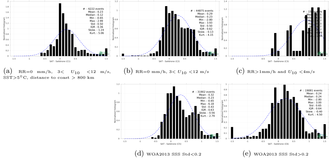
Figure 13: Normalized histogram of \Delta\text{SSS} (SMOS SSS L4 v2 - Daily (BEC) - Saildrone) for 5 different subdatasets corresponding to: RR=0 mm/h, 3 < U_{10} < 12 m/s, SST>5°C, distance to coast > 800 km (a), RR=0 mm/h, 3 < U_{10} < 12 m/s (b), RR>1mm/h and U_{10} < 4 m/s (c), WOA2013 SSS Std<0.2 (d), WOA2013 SSS Std>0.2 (e).
