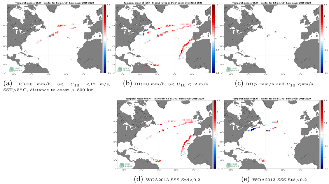
Figure 12: Temporal mean gridded over spatial boxes of size 1^\circ \times 1^\circ of \Delta\text{SSS} (SMOS SSS L4 v2 - Daily (BEC) - Sairdrone) for 5 different subdatasets corresponding to:RR=0 mm/h, 3 < U_{10} < 12 m/s, SST >5^\circ\text{C} , distance to coast > 800 km (a), RR=0 mm/h, 3 < U_{10} < 12 m/s (b), RR >1 mm/h and U_{10} < 4 m/s (c), WOA2013 SSS Std <0.2 (d), WOA2013 SSS Std >0.2 (e).
