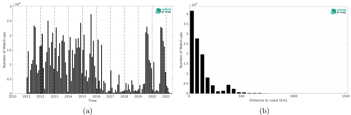
Figure 2: Number of match-ups between ICES and SMOS SSS L4 v2 - Daily (BEC) SSS as a function of time (a) and as function of the distance to coast (b) over the North Atlantic Ocean Pi-MEP region and for the full satellite product period.
