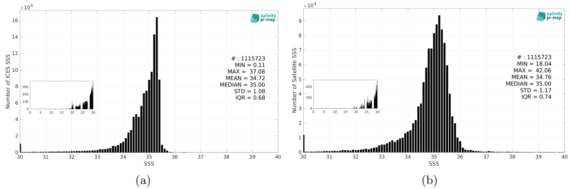
Figure 3: Histograms of SSS from ICES (a) and SMOS SSS L4 v2 - Daily (BEC) (b) considering all match-up pairs per bins of 0.1 over the North Atlantic Ocean Pi-MEP region and for the full satellite product period.
