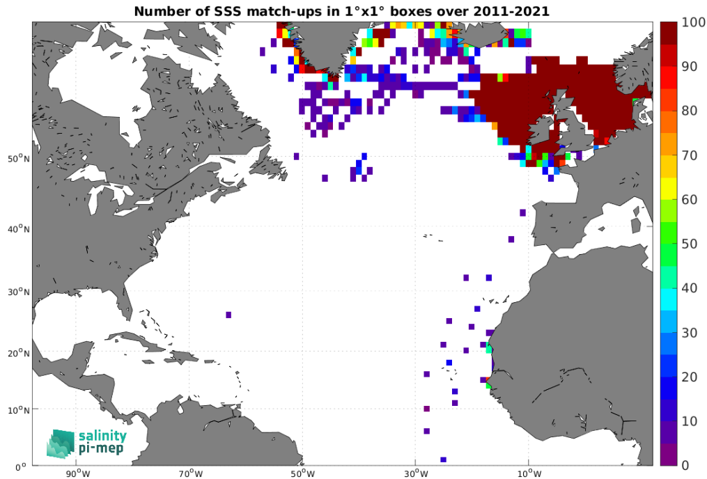
Figure 5: Number of SSS match-ups between ICES SSS and the SMOS SSS L4 v2 - Daily (BEC) SSS product for the North Atlantic Ocean Pi-MEP region over 1^\circ \times 1^\circ boxes and for the full satellite product period.
