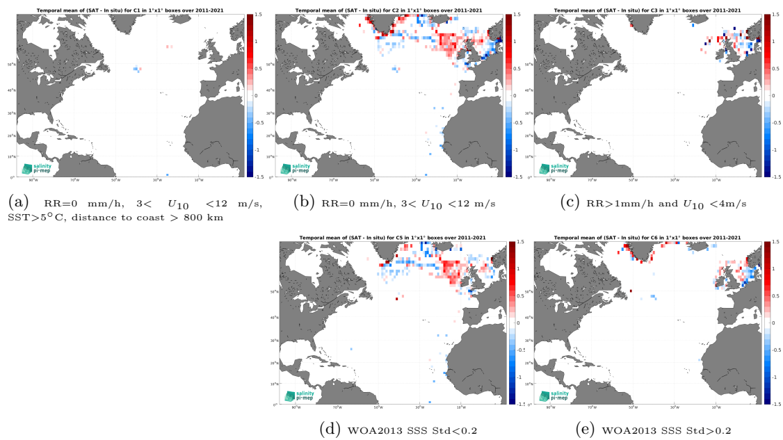
Figure 14: Temporal mean gridded over spatial boxes of size 1^\circ \times 1^\circ of \Delta\text{SSS} (SMOS SSS L4 v2 - Daily (BEC) - ICES) for 5 different subdatasets corresponding to:RR=0 mm/h, 3 < U_{10} < 12 m/s, SST >5^\circ\text{C} , distance to coast > 800 km (a), RR=0 mm/h, 3 < U_{10} < 12 m/s (b), RR >1 mm/h and U_{10} < 4 m/s (c), WOA2013 SSS Std <0.2 (d), WOA2013 SSS Std >0.2 (e).
