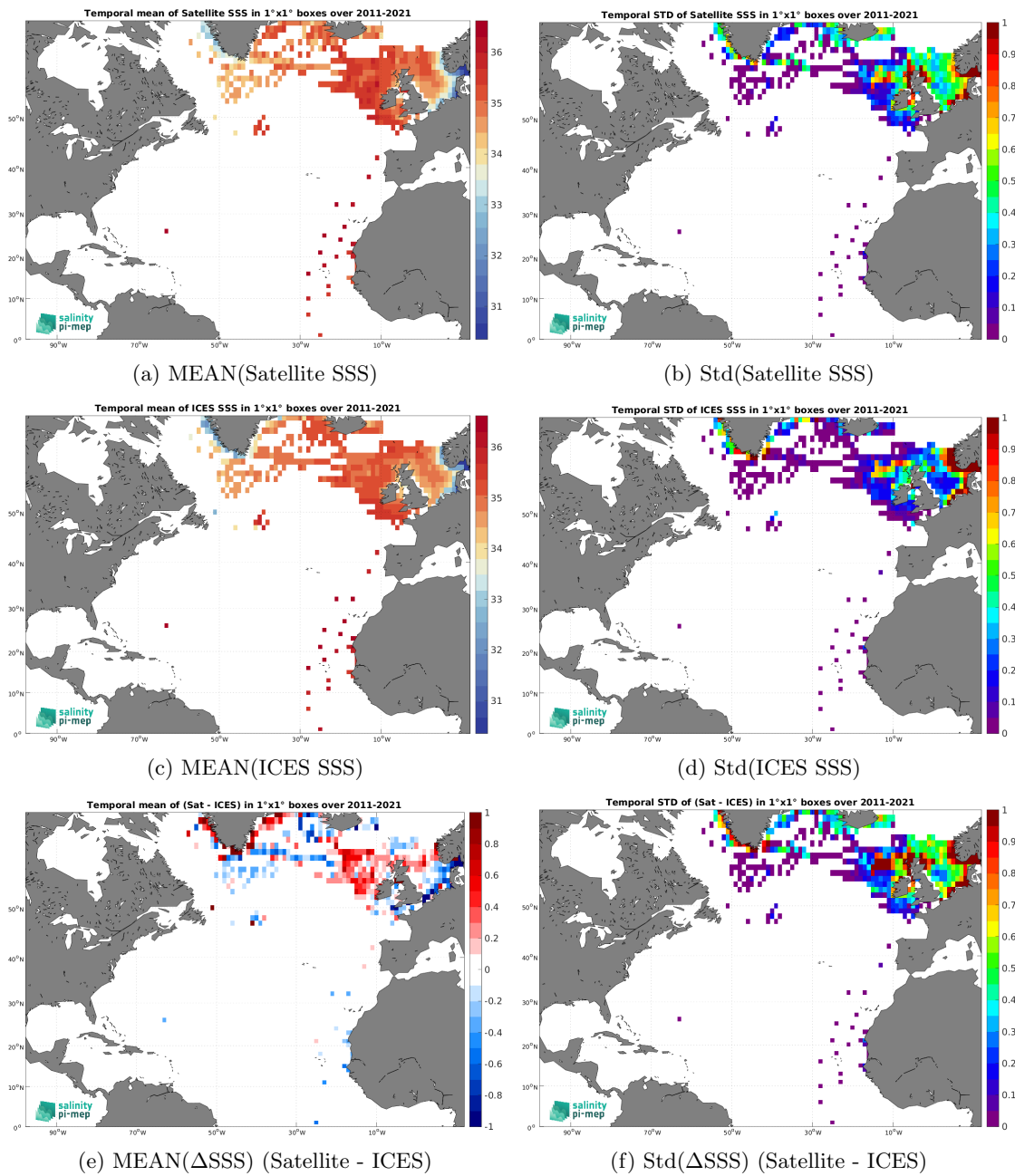
Figure 7: Temporal mean (left) and Std (right) of SSS from SMOS SSS L4 v2 - Daily (BEC) (top), ICES (middle), and of \Delta SSS (Satellite - ICES). Only match-up pairs are used to generate these maps.
