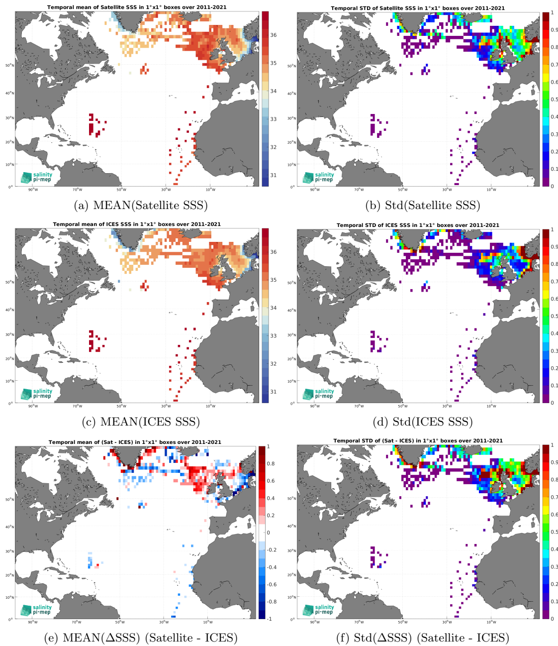
Figure 6: Temporal mean (left) and Std (right) of SSS from SMOS SSS L4 v2 - Daily (BEC) (top), ICES (middle), and of \Delta SSS (Satellite - ICES). Only match-up pairs are used to generate these maps.
