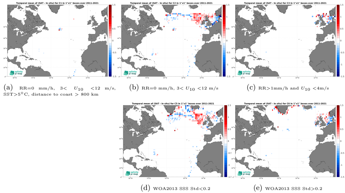
Figure 12: Temporal mean gridded over spatial boxes of size 1^\circ \times 1^\circ of \Delta SSS (SMOS SSS L4 v2 - Daily (BEC) - ICES) for 5 different subdatasets corresponding to:RR=0 mm/h, 3 < U_{10} < 12 m/s, SST >5^\circ\text{C} , distance to coast > 800 km (a), RR=0 mm/h, 3 < U_{10} < 12 m/s (b), RR >1 mm/h and U_{10} < 4 m/s (c), WOA2013 SSS Std <0.2 (d), WOA2013 SSS Std >0.2 (e).
