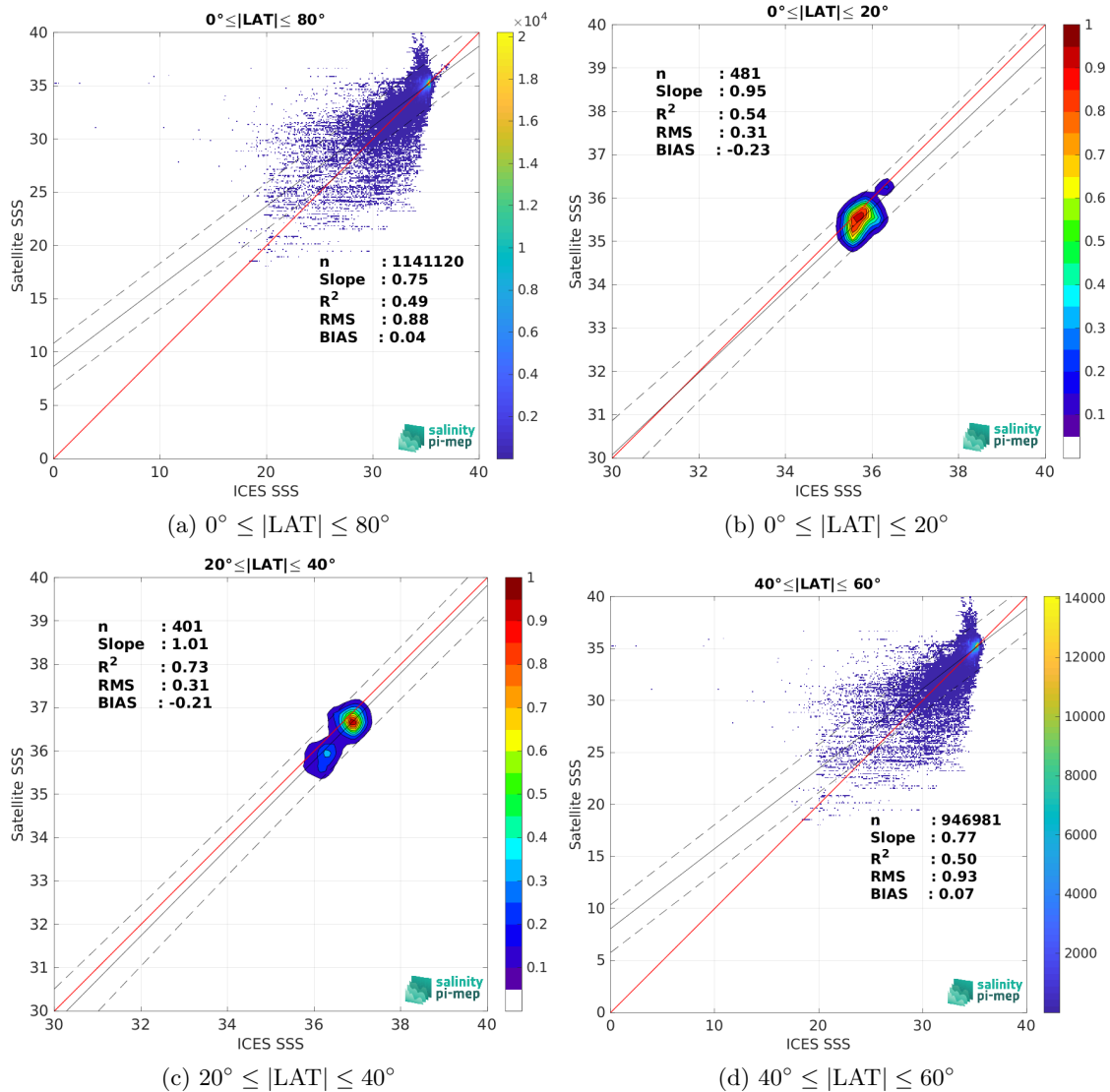
Figure 9: Contour maps of the concentration of SMOS SSS L4 v2 - Daily (BEC) SSS (y-axis) versus ICES SSS (x-axis) at match-up pairs for different latitude bands. For each plot, the red line shows x=y . The black thin and dashed lines indicate a linear fit through the data cloud and the \pm 95\% confidence levels, respectively. The number match-up pairs n , the slope and R^2 coefficient of the linear fit, the root mean square (RMS) and the mean bias between satellite and in situ data are indicated for each latitude band in each plots.
