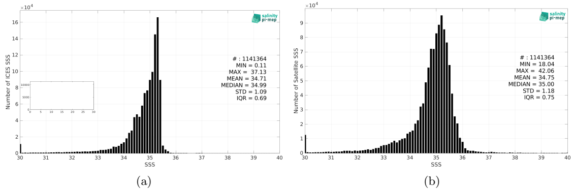
Figure 2: Histograms of SSS from ICES (a) and SMOS SSS L4 v2 - Daily (BEC) (b) considering all match-up pairs per bins of 0.1 over the North Atlantic Ocean Pi-MEP region and for the full satellite product period.
