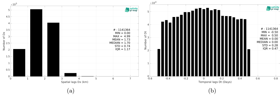
Figure 5: Histograms of the spatial (a) and temporal (b) lags between the location/time of the ICES measurement and the date of the corresponding SMOS SSS L4 v2 - Daily (BEC) SSS pixel.
