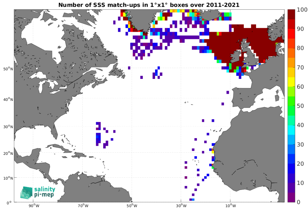
Figure 4: Number of SSS match-ups between ICES SSS and the SMOS SSS L4 v2 - Daily (BEC) SSS product for the North Atlantic Ocean Pi-MEP region over 1^\circ \times 1^\circ boxes and for the full satellite product period.
