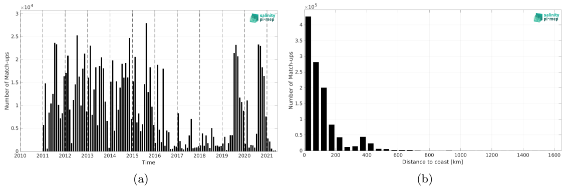
Figure 1: Number of match-ups between ICES and SMOS SSS L4 v2 - Daily (BEC) SSS as a function of time (a) and as function of the distance to coast (b) over the North Atlantic Ocean Pi-MEP region and for the full satellite product period.
