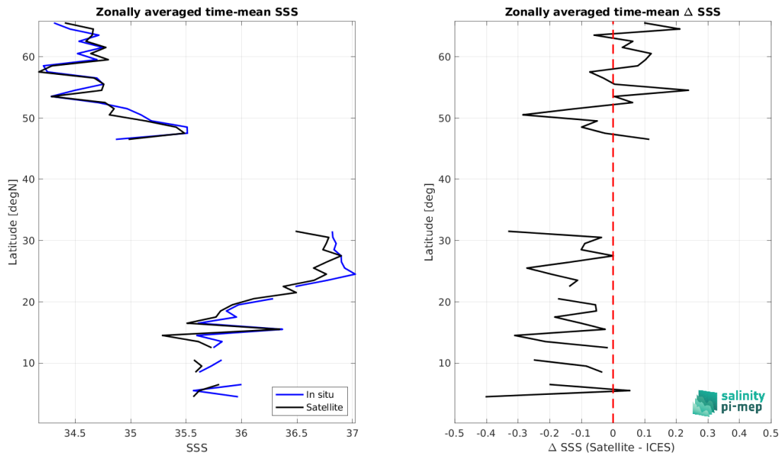
Figure 8: Left panel: Zonal mean SSS from SMOS SSS L4 v2 - Daily (BEC) satellite product (black) and from ICES (blue). Right panel: Zonal mean of \Delta SSS (Satellite - ICES) for all the collected Pi-MEP match-up pairs estimated over the full satellite product period.
