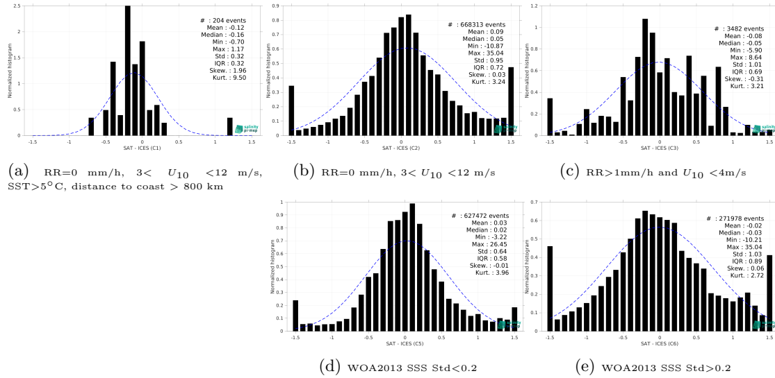
Figure 13: Normalized histogram of \Delta SSS (SMOS SSS L4 v2 - Daily (BEC) - ICES) for 5 different subdatasets corresponding to: RR=0 mm/h, 3 < U_{10} < 12 m/s, SST > 5°C, distance to coast > 800 km (a), RR=0 mm/h, 3 < U_{10} < 12 m/s (b), RR > 1mm/h and U_{10} < 4 m/s (c), WOA2013 SSS Std < 0.2 (d), WOA2013 SSS Std > 0.2 (e).
