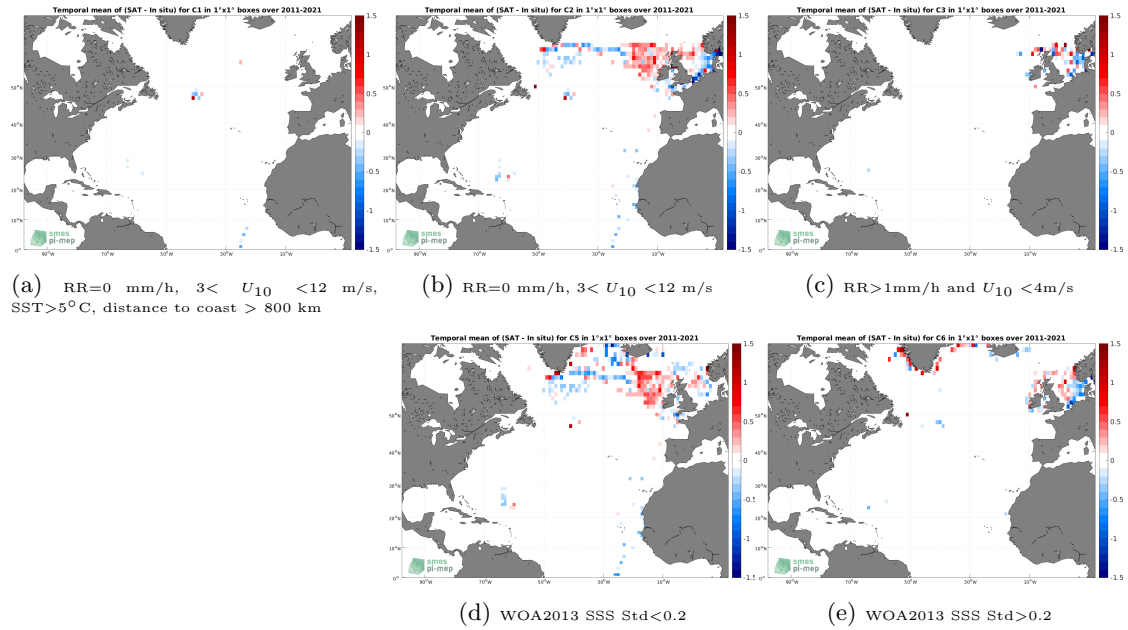
Figure 12: Temporal mean gridded over spatial boxes of size 1^\circ \times 1^\circ of \Delta\text{SSS} (SMOS SSS L4 v2 - Daily (BEC) - ICES) for 5 different subdatasets corresponding to:RR=0 mm/h, 3 < U_{10} < 12 m/s, SST >5^\circ\text{C} , distance to coast > 800 km (a), RR=0 mm/h, 3 < U_{10} < 12 m/s (b), RR >1 mm/h and U_{10} < 4 m/s (c), WOA2013 SSS Std <0.2 (d), WOA2013 SSS Std >0.2 (e).
