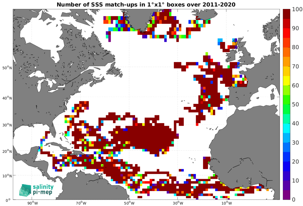
Figure 4: Number of SSS match-ups between Surface drifters SSS and the SMOS SSS L4 v2 - Daily (BEC) SSS product for the North Atlantic Ocean Pi-MEP region over 1^\circ \times 1^\circ boxes and for the full satellite product period.
