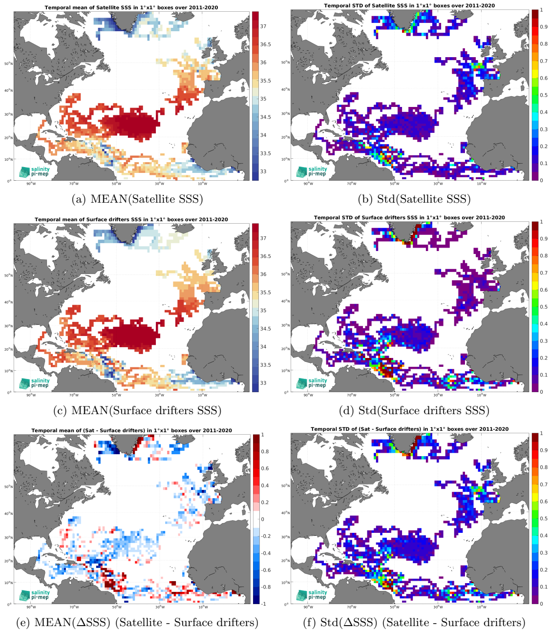
Figure 6: Temporal mean (left) and Std (right) of SSS from SMOS SSS L4 v2 - Daily (BEC) (top), Surface drifters (middle), and of \Delta SSS (Satellite - Surface drifters). Only match-up pairs are used to generate these maps.
