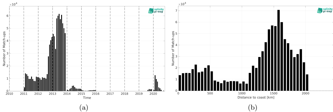
Figure 2: Number of match-ups between Surface drifters and SMOS SSS L4 v2 - Daily (BEC) SSS as a function of time (a) and as function of the distance to coast (b) over the North Atlantic Ocean Pi-MEP region and for the full satellite product period.
