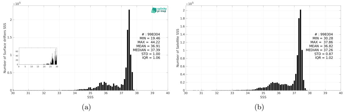
Figure 3: Histograms of SSS from Surface drifters (a) and SMOS SSS L4 v2 - Daily (BEC) (b) considering all match-up pairs per bins of 0.1 over the North Atlantic Ocean Pi-MEP region and for the full satellite product period.
