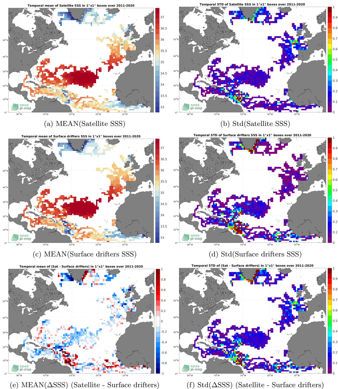
Figure 5: Temporal mean (left) and Std (right) of SSS from SMOS SSS L4 v2 - Daily (BEC) (top), Surface drifters (middle), and of \Delta SSS (Satellite - Surface drifters). Only match-up pairs are used to generate these maps.
