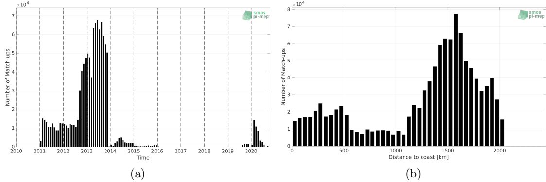
Figure 1: Number of match-ups between Surface drifters and SMOS SSS L4 v2 - Daily (BEC) SSS as a function of time (a) and as function of the distance to coast (b) over the North Atlantic Ocean Pi-MEP region and for the full satellite product period.
