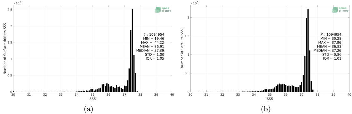
Figure 2: Histograms of SSS from Surface drifters (a) and SMOS SSS L4 v2 - Daily (BEC) (b) considering all match-up pairs per bins of 0.1 over the North Atlantic Ocean Pi-MEP region and for the full satellite product period.
