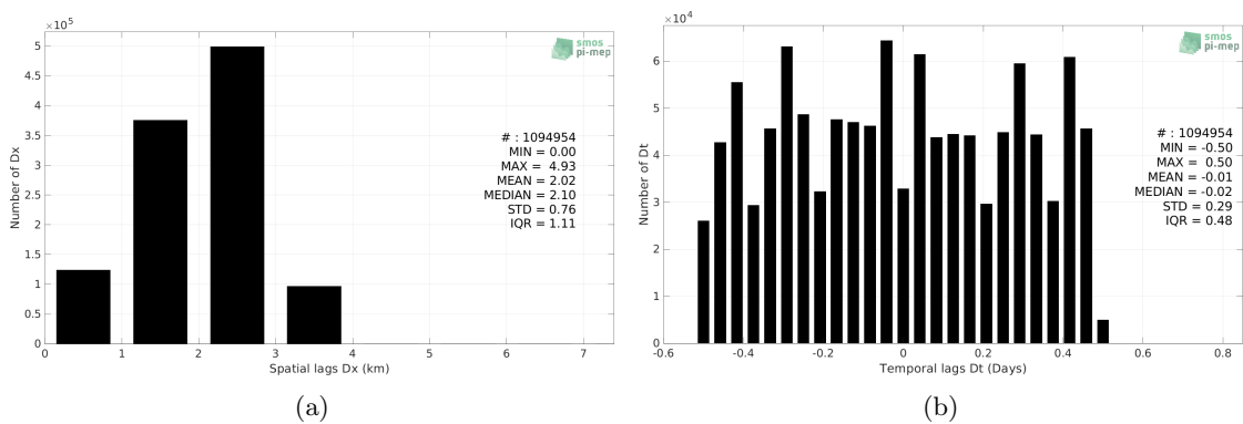
Figure 4: Histograms of the spatial (a) and temporal (b) lags between the location/time of the Surface drifters measurement and the date of the corresponding SMOS SSS L4 v2 - Daily (BEC) SSS pixel.
