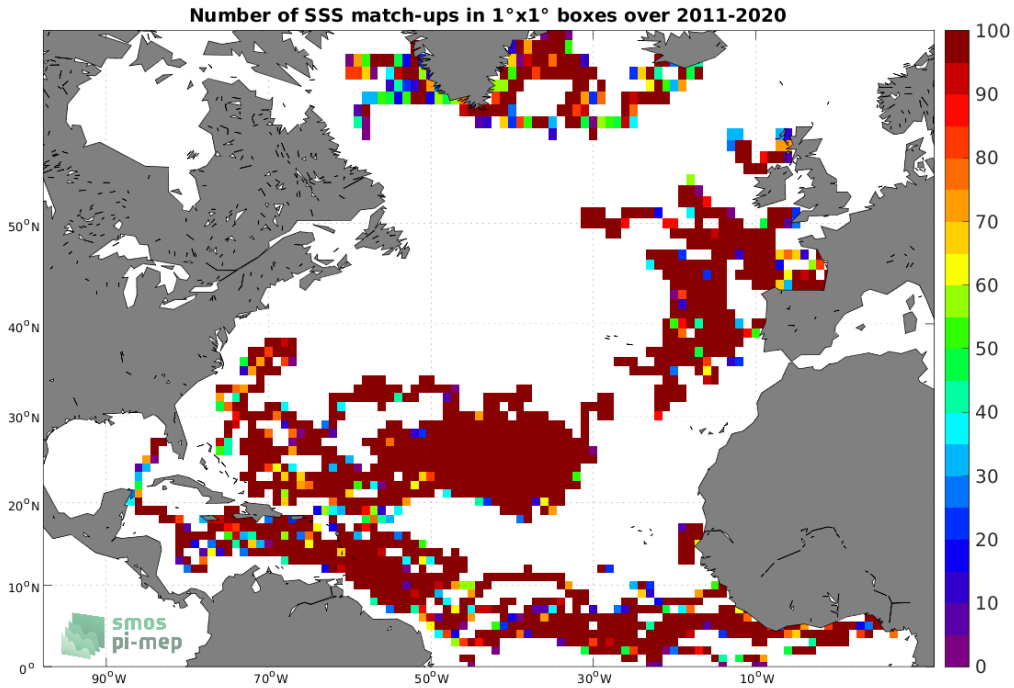
Figure 3: Number of SSS match-ups between Surface drifters SSS and the SMOS SSS L4 v2 - Daily (BEC) SSS product for the North Atlantic Ocean Pi-MEP region over 1^\circ \times 1^\circ boxes and for the full satellite product period.
