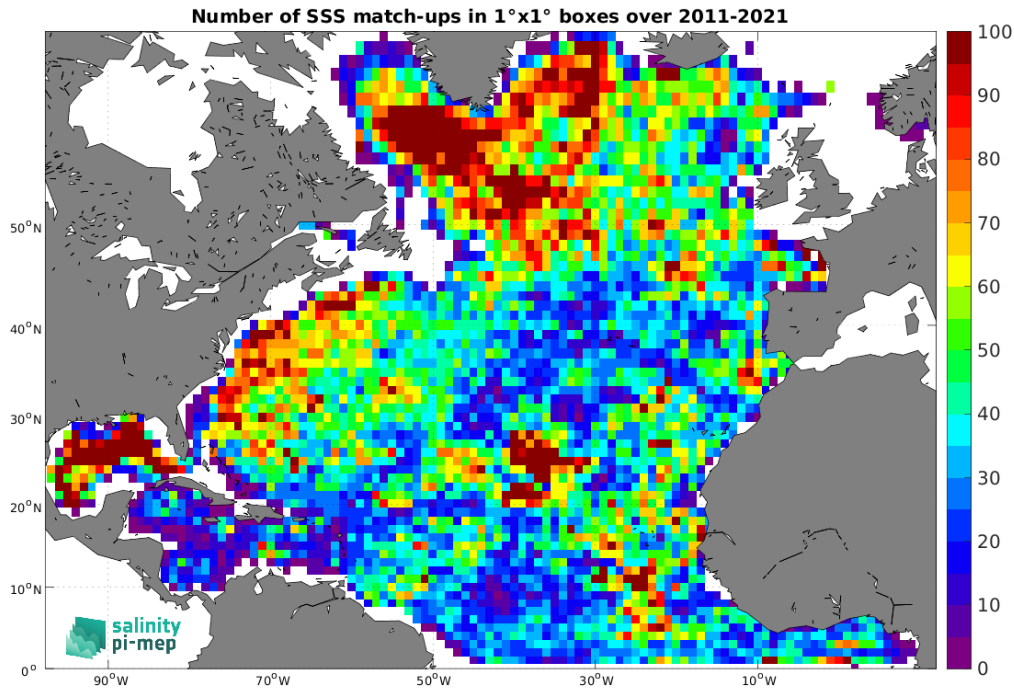
Figure 5: Number of SSS match-ups between Argo SSS and the SMOS SSS L4 v2 - Daily (BEC) SSS product for the North Atlantic Ocean Pi-MEP region over 1^{\circ} \times 1^{\circ} boxes and for the full satellite product period.
