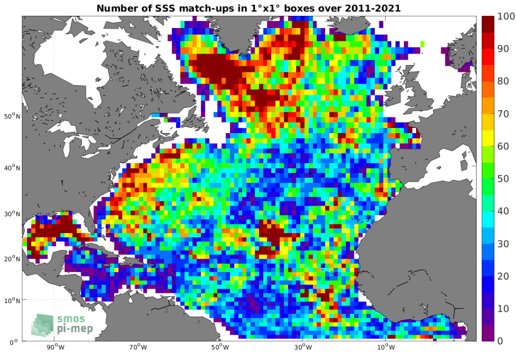
Figure 4: Number of SSS match-ups between Argo SSS and the SMOS SSS L4 v2 - Daily (BEC) SSS product for the North Atlantic Ocean Pi-MEP region over 1^\circ \times 1^\circ boxes and for the full satellite product period.
