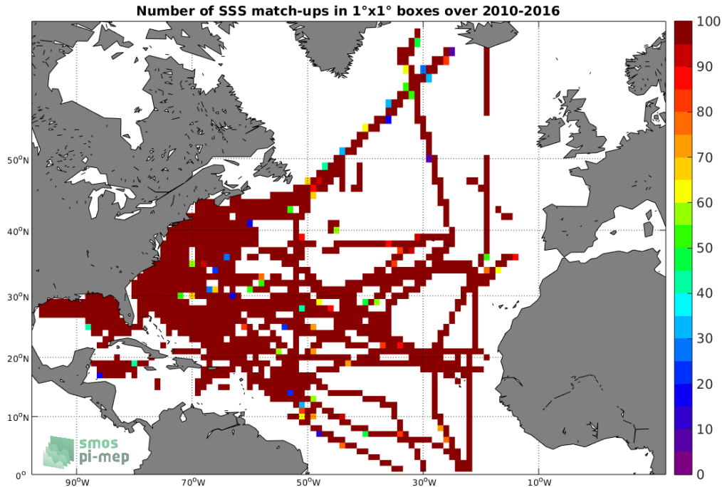
Figure 4: Number of SSS match-ups between TSG (SAMOS) SSS and the SMOS SSS L3 v3 Monthly (ICDC) SSS product for the North Atlantic Ocean Pi-MEP region over 1°x1° boxes and for the full satellite product period.
