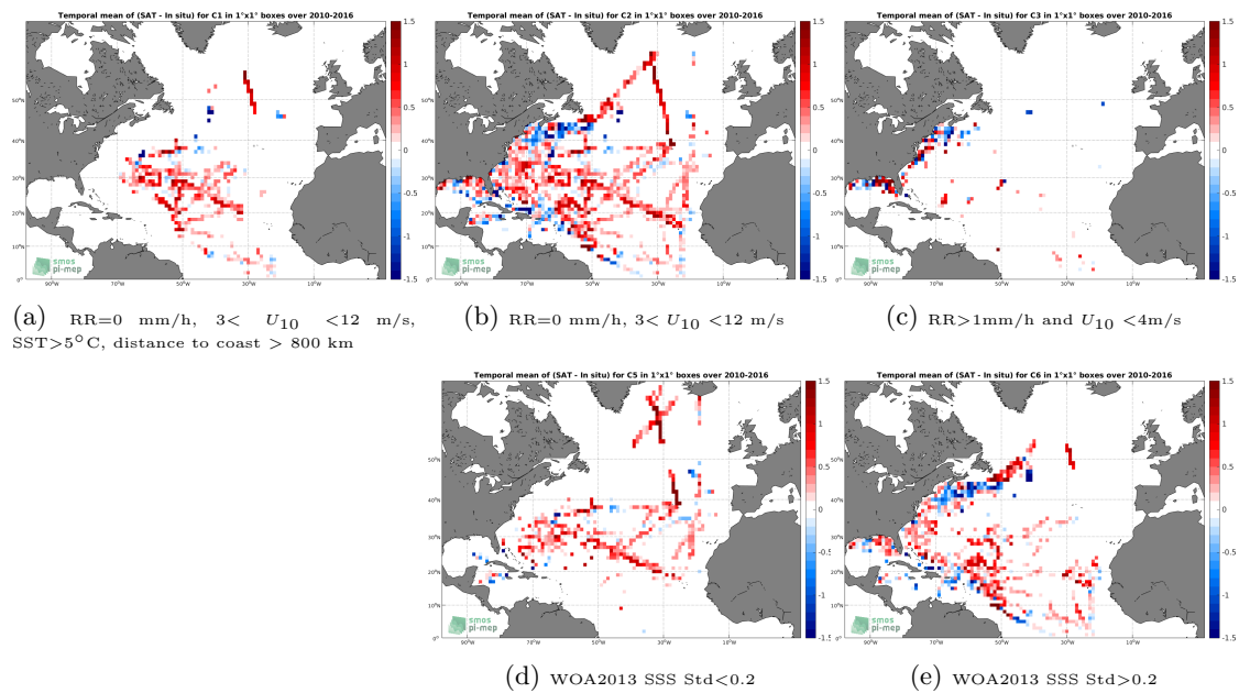
Figure 12: Temporal mean gridded over spatial boxes of size 1^\circ \times 1^\circ of \Delta SSS (SMOS SSS L3 v3 Monthly (ICDC) - TSG (SAMOS)) for 5 different subdatasets corresponding to:RR=0 mm/h, 3 < U_{10} < 12 m/s, SST >5^\circ\text{C} , distance to coast > 800 km (a), RR=0 mm/h, 3 < U_{10} < 12 m/s (b), RR >1 mm/h and U_{10} < 4 m/s (c), WOA2013 SSS Std <0.2 (d), WOA2013 SSS Std >0.2 (e).
