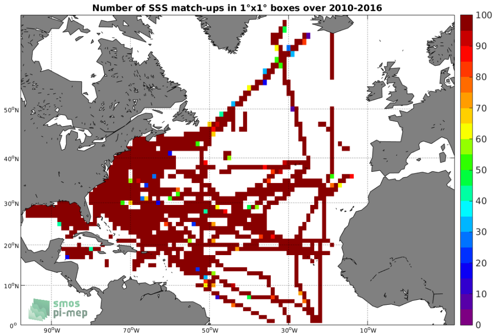
Figure 4: Number of SSS match-ups between TSG-SAMOS SSS and the SMOS-L3-ICDC-V3-MONTHLY-0.5DEG SSS product for the North Atlantic Ocean Pi-MEP region over 1°x1° boxes and for the full satellite product period.
