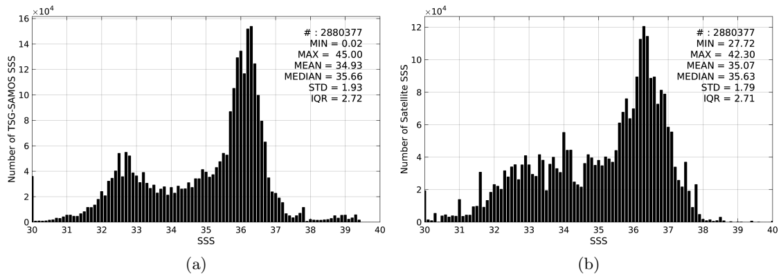
Figure 2: Histograms of SSS from TSG-SAMOS (a) and SMOS-L3-ICDC-V3-MONTHLY-0.5DEG (b) considering all match-up pairs per bins of 0.1 over the North Atlantic Ocean Pi-MEP region and for the full satellite product period.
