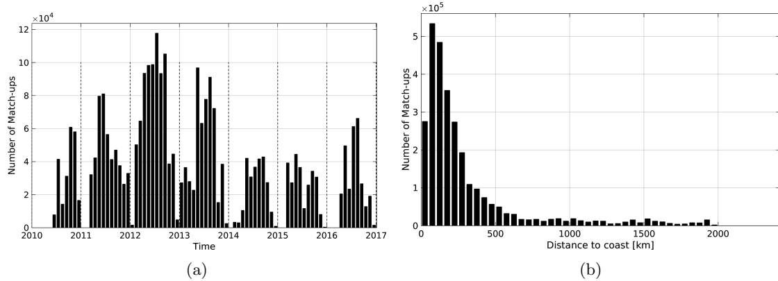
Figure 1: Number of match-ups between TSG-SAMOS and SMOS-L3-ICDC-V3-MONTHLY-0.5DEG SSS as a function of time (a) and as function of the distance to coast (b) over the North Atlantic Ocean Pi-MEP region and for the full satellite product period.
