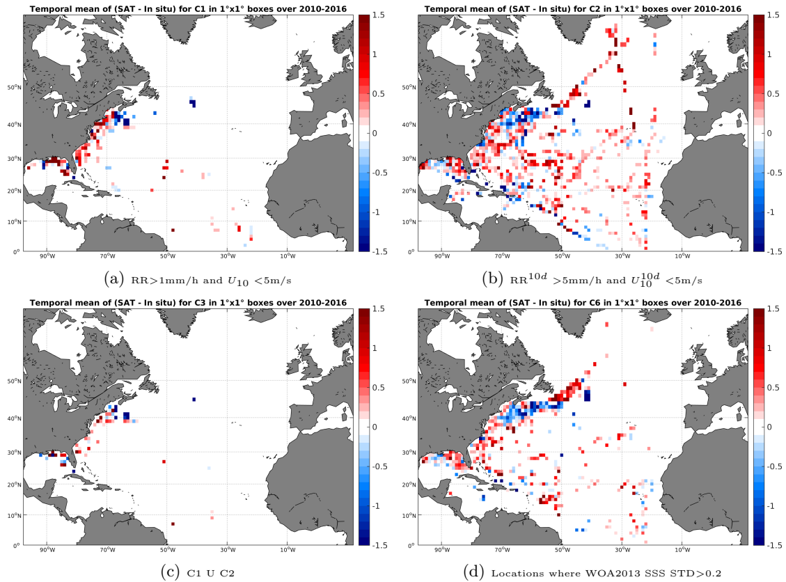
Figure 12: Temporal mean gridded over spatial boxes of size 1^\circ \times 1^\circ of \Delta SSS (SMOS-L3-ICDC-V3-MONTHLY-0.5DEG - TSG-SAMOS) for 4 different subdatasets corresponding to:RR >1 mm/h and U_{10} < 5 m/s (a), RR 10d > 5 mm/h and U_{10}^{10d} < 5 m/s (b), C1 U C2 (c),Locations where WOA2013 SSS STD >0.2 (d).
