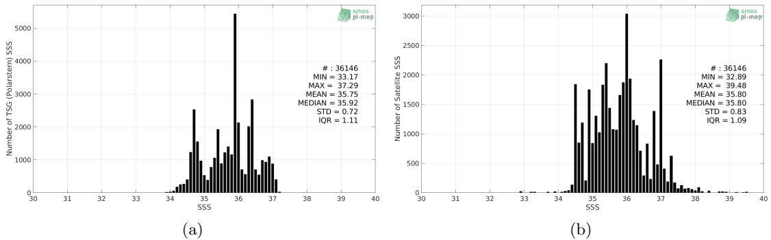
Figure 2: Histograms of SSS from TSG (Polarstern) (a) and SMOS SSS L3 v3 Monthly (ICDC) (b) considering all match-up pairs per bins of 0.1 over the North Atlantic Ocean Pi-MEP region and for the full satellite product period.
