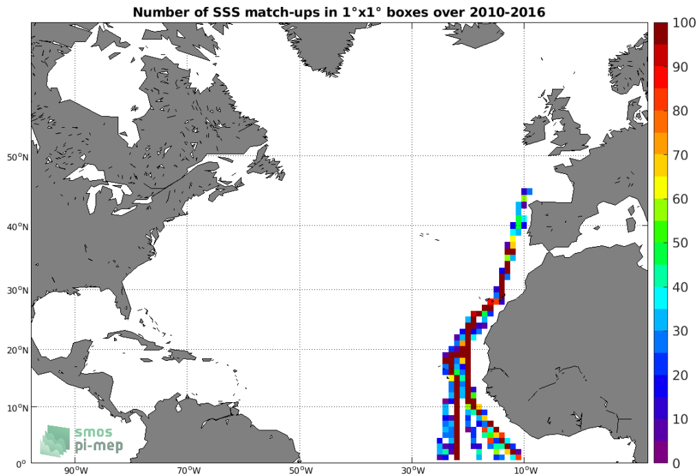
Figure 4: Number of SSS match-ups between TSG (Polarstern) SSS and the SMOS SSS L3 v3 Monthly (ICDC) SSS product for the North Atlantic Ocean Pi-MEP region over 1^\circ \times 1^\circ boxes and for the full satellite product period.
