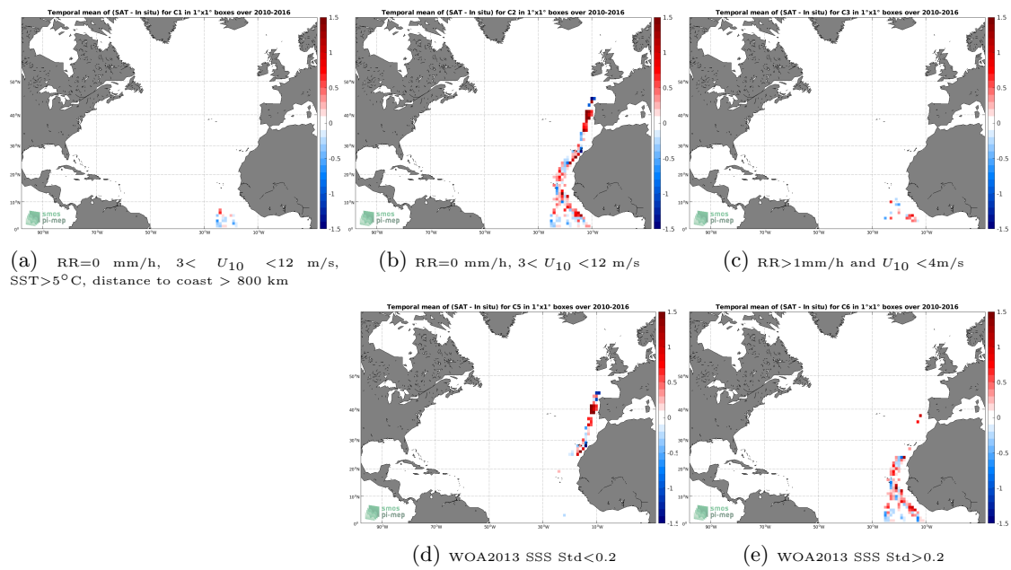
Figure 12: Temporal mean gridded over spatial boxes of size 1^\circ \times 1^\circ of \Delta SSS (SMOS SSS L3 v3 Monthly (ICDC) - TSG (Polarstern)) for 5 different subdatasets corresponding to:RR=0 mm/h, 3 < U_{10} < 12 m/s, SST >5^\circ\text{C} , distance to coast > 800 km (a), RR=0 mm/h, 3 < U_{10} < 12 m/s (b), RR >1 mm/h and U_{10} < 4 m/s (c), WOA2013 SSS Std <0.2 (d), WOA2013 SSS Std >0.2 (e).
