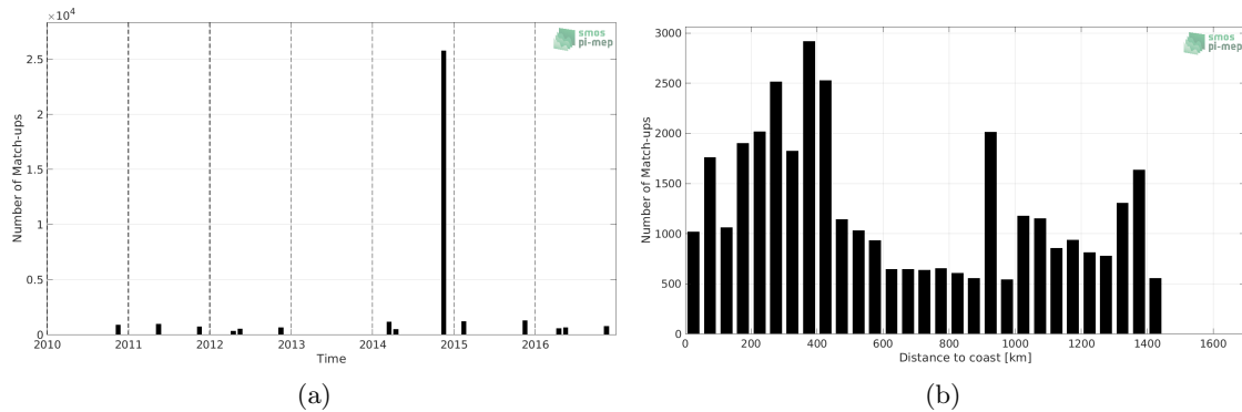
Figure 1: Number of match-ups between TSG (Polarstern) and SMOS SSS L3 v3 Monthly (ICDC) SSS as a function of time (a) and as function of the distance to coast (b) over the North Atlantic Ocean Pi-MEP region and for the full satellite product period.
