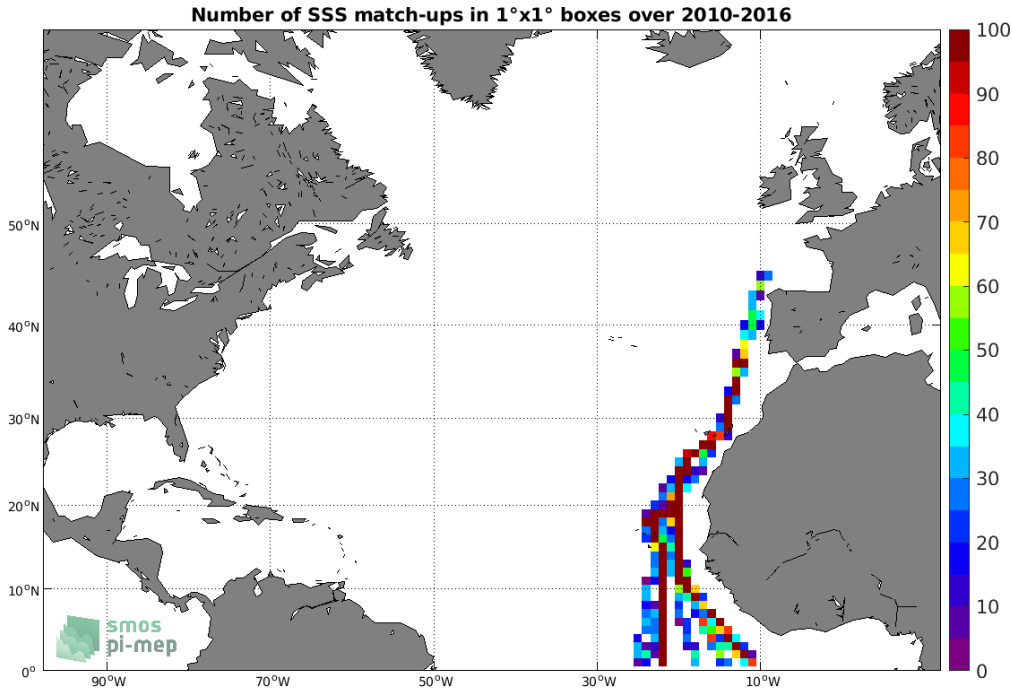
Figure 4: Number of SSS match-ups between TSG (Polarstern) SSS and the SMOS SSS L3 v3 Monthly (ICDC) SSS product for the North Atlantic Ocean Pi-MEP region over 1^{\circ} \times 1^{\circ} boxes and for the full satellite product period.
