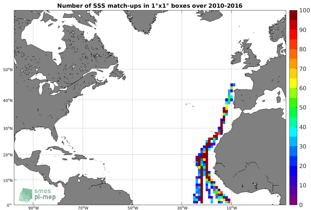
Figure 4: Number of SSS match-ups between TSG (Polarstern) SSS and the SMOS SSS L3 v3 Monthly (ICDC) SSS product for the North Atlantic Ocean Pi-MEP region over 1°x1° boxes and for the full satellite product period.
