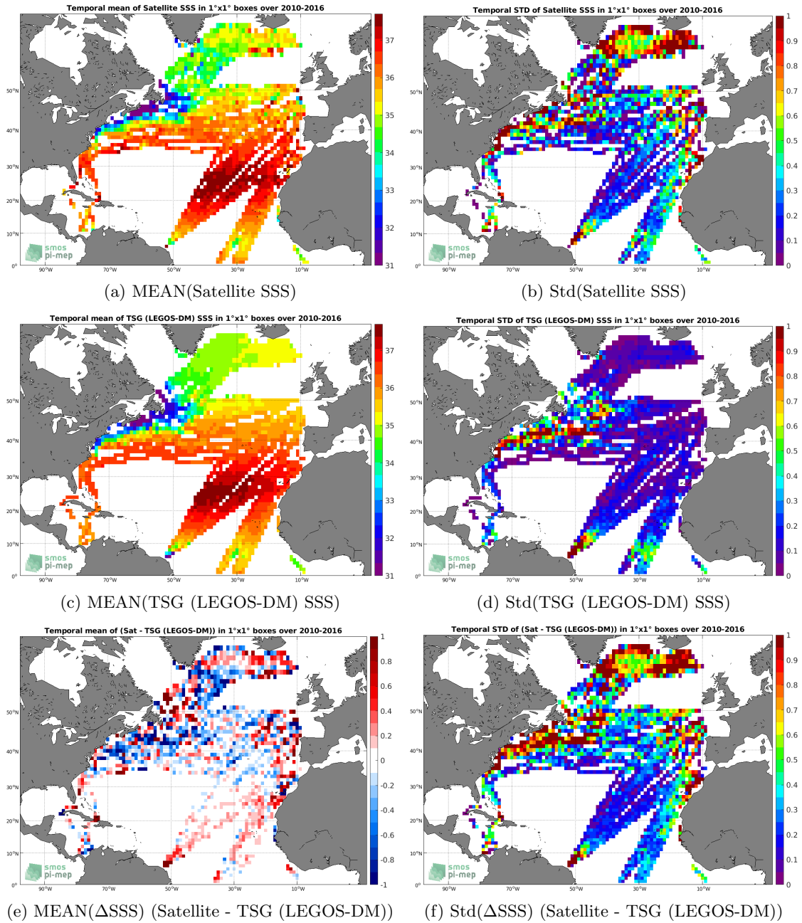
Figure 6: Temporal mean (left) and Std (right) of SSS from SMOS SSS L3 v3 Monthly (ICDC) (top), TSG (LEGOS-DM) (middle), and of \Delta SSS (Satellite - TSG (LEGOS-DM)). Only match-pairs are used to generate these maps.
