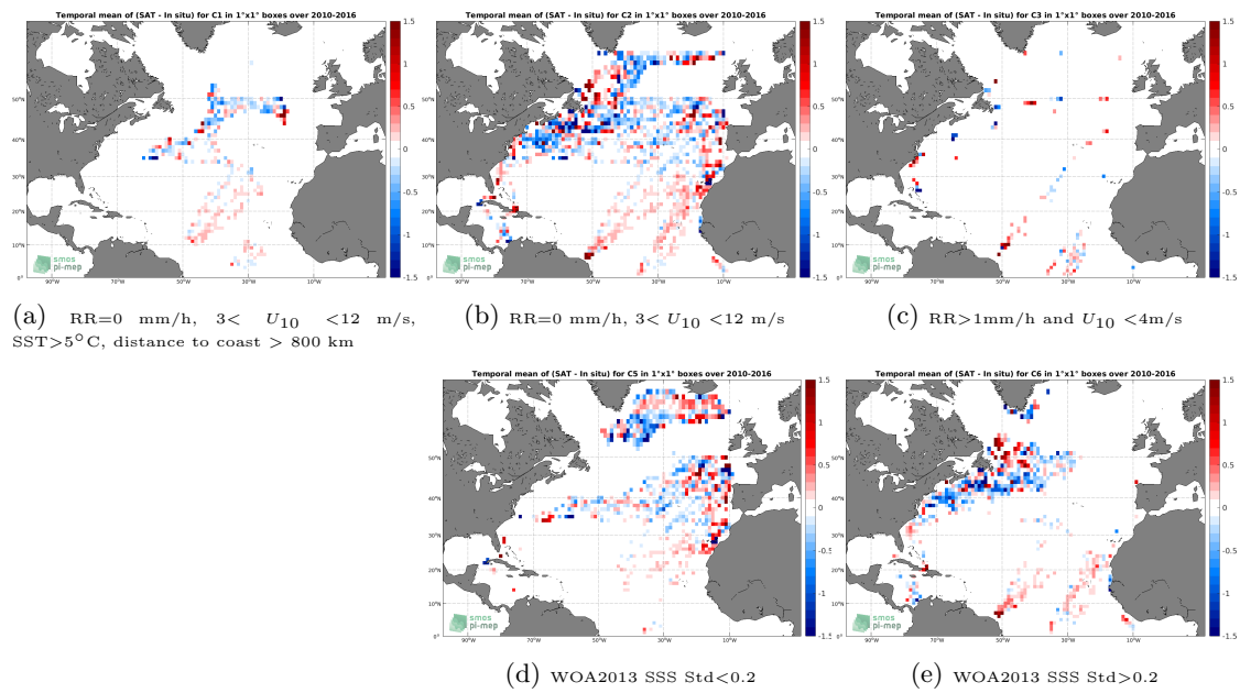
Figure 12: Temporal mean gridded over spatial boxes of size 1^\circ \times 1^\circ of \Delta\text{SSS} (SMOS SSS L3 v3 Monthly (ICDC) - TSG (LEGOS-DM)) for 5 different subdatasets corresponding to:RR=0 mm/h, 3 < U_{10} < 12 m/s, SST > 5^\circ\text{C} , distance to coast > 800 km (a), RR=0 mm/h, 3 < U_{10} < 12 m/s (b), RR > 1 mm/h and U_{10} < 4 m/s (c), WOA2013 SSS Std < 0.2 (d), WOA2013 SSS Std > 0.2 (e).
