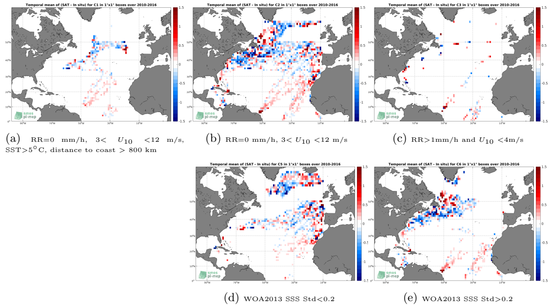
Figure 12: Temporal mean gridded over spatial boxes of size 1^\circ \times 1^\circ of \Delta\text{SSS} (SMOS-L3-ICDC-V3-MONTHLY-0.5DEG - TSG-LEGOS-DM) for 5 different subdatasets corresponding to:RR=0 mm/h, 3 < U_{10} < 12 m/s, SST > 5^\circ\text{C} , distance to coast > 800 km (a), RR=0 mm/h, 3 < U_{10} < 12 m/s (b), RR > 1 mm/h and U_{10} < 4 m/s (c), WOA2013 SSS Std < 0.2 (d), WOA2013 SSS Std > 0.2 (e).
