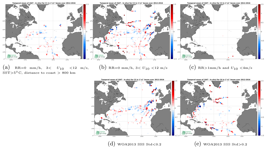
Figure 12: Temporal mean gridded over spatial boxes of size 1^\circ \times 1^\circ of \Delta\text{SSS} (SMOS SSS L3 v3 Monthly (ICDC) - TSG (GOSUD-Sailing-ship)) for 5 different subdatasets corresponding to:RR=0 mm/h, 3 < U_{10} < 12 m/s, SST>5°C, distance to coast > 800 km (a), RR=0 mm/h, 3 < U_{10} < 12 m/s (b), RR>1mm/h and U_{10} < 4 m/s (c), WOA2013 SSS Std<0.2 (d), WOA2013 SSS Std>0.2 (e).
