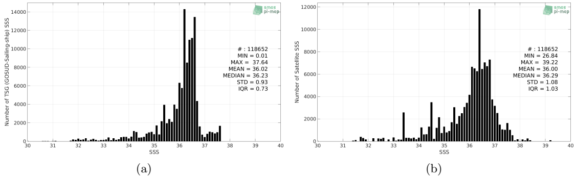
Figure 2: Histograms of SSS from TSG (GOSUD-Sailing-ship) (a) and SMOS SSS L3 v3 Monthly (ICDC) (b) considering all match-up pairs per bins of 0.1 over the North Atlantic Ocean Pi-MEP region and for the full satellite product period.
