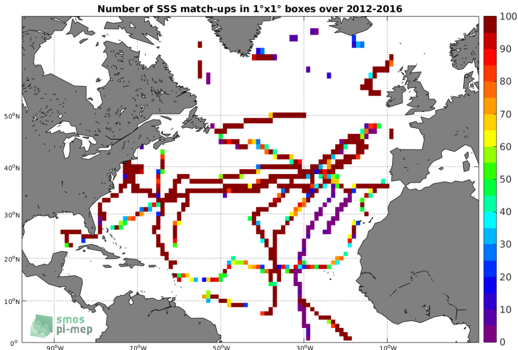
Figure 4: Number of SSS match-ups between TSG-GOSUD-Sailing-ship SSS and the SMOS-L3-ICDC-V3-MONTHLY-0.5DEG SSS product for the North Atlantic Ocean Pi-MEP region over 1^\circ \times 1^\circ boxes and for the full satellite product period.
