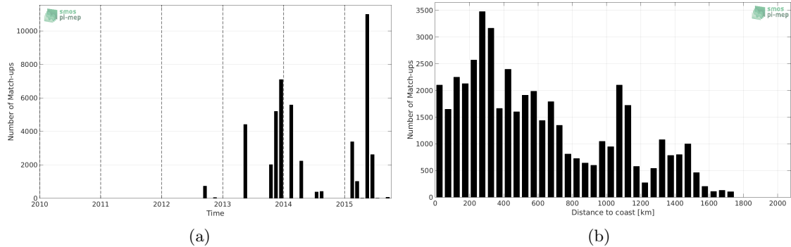
Figure 1: Number of match-ups between TSG-GOSUD-Sailing-ship and SMOS-L3-ICDC-V3-MONTHLY-0.5DEG SSS as a function of time (a) and as function of the distance to coast (b) over the North Atlantic Ocean Pi-MEP region and for the full satellite product period.
