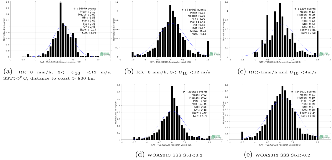
Figure 13: Normalized histogram of \Delta SSS (SMOS-L3-ICDC-V3-MONTHLY-0.5DEG - TSG-GOSUD-Research-vessel) for 5 different subdatasets corresponding to: RR=0 mm/h, 3 < U_{10} < 12 m/s, SST >5^{\circ}\text{C} , distance to coast > 800 km (a), RR=0 mm/h, 3 < U_{10} < 12 m/s (b), RR >1 mm/h and U_{10} < 4 m/s (c), WOA2013 SSS Std <0.2 (d), WOA2013 SSS Std >0.2 (e).
