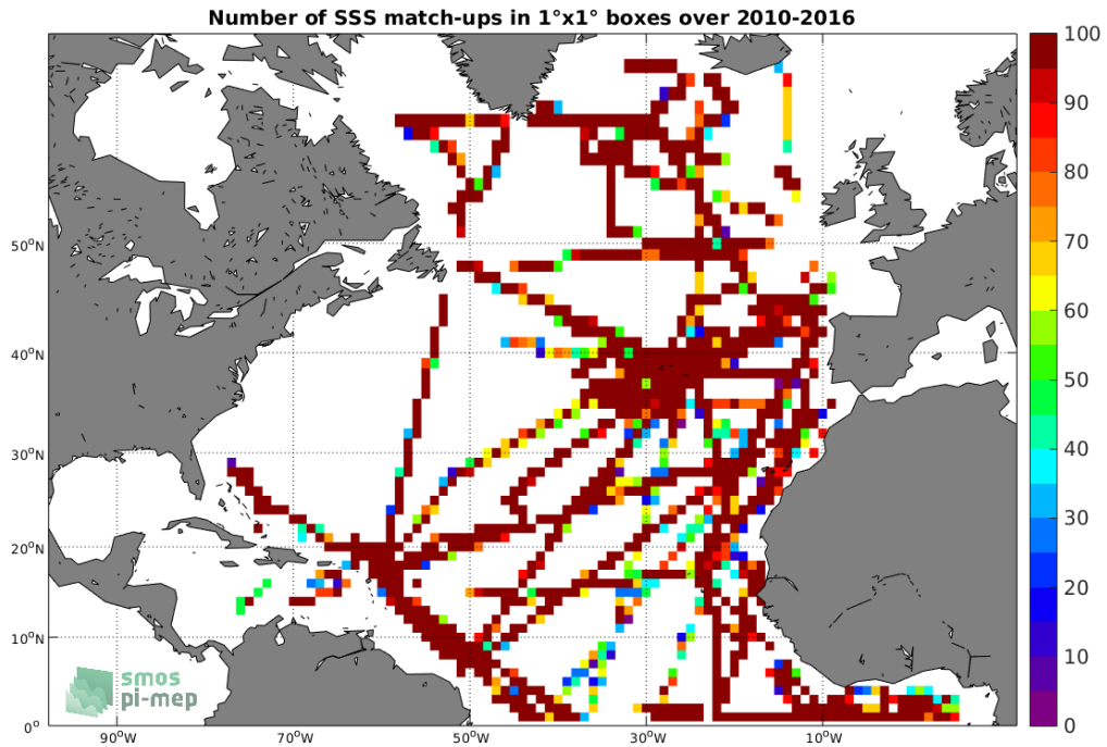
Figure 4: Number of SSS match-ups between TSG-GOSUD-Research-vessel SSS and the SMOS-L3-ICDC-V3-MONTHLY-0.5DEG SSS product for the North Atlantic Ocean Pi-MEP region over 1^\circ \times 1^\circ boxes and for the full satellite product period.
