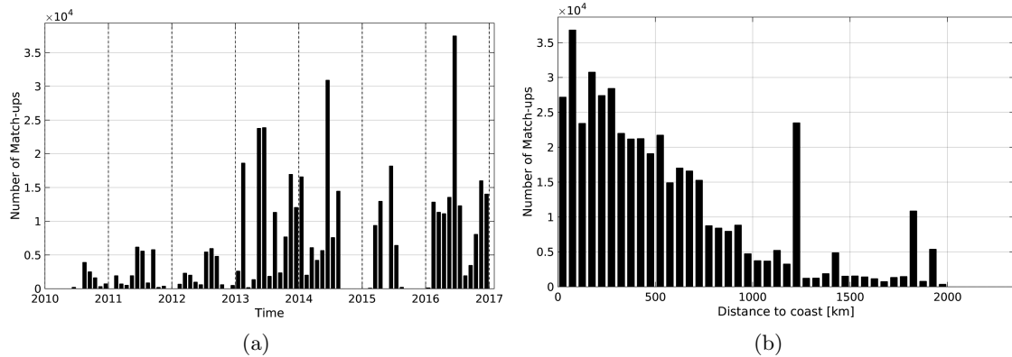
Figure 1: Number of match-ups between TSG-GOSUD-Research-vessel and SMOS-L3-ICDC-V3-MONTHLY-0.5DEG SSS as a function of time (a) and as function of the distance to coast (b) over the North Atlantic Ocean Pi-MEP region and for the full satellite product period.
