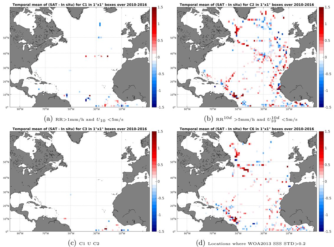
Figure 12: Temporal mean gridded over spatial boxes of size 1^\circ \times 1^\circ of \Delta SSS (SMOS-L3-ICDC-V3-MONTHLY-0.5DEG - TSG-GOSUD-Research-vessel) for 4 different subdatasets corresponding to: RR > 1 mm/h and U_{10} < 5 m/s (a), RR 10d > 5 mm/h and U_{10}^{10d} < 5 m/s (b), C1 U C2 (c), Locations where WOA2013 SSS STD > 0.2 (d).
