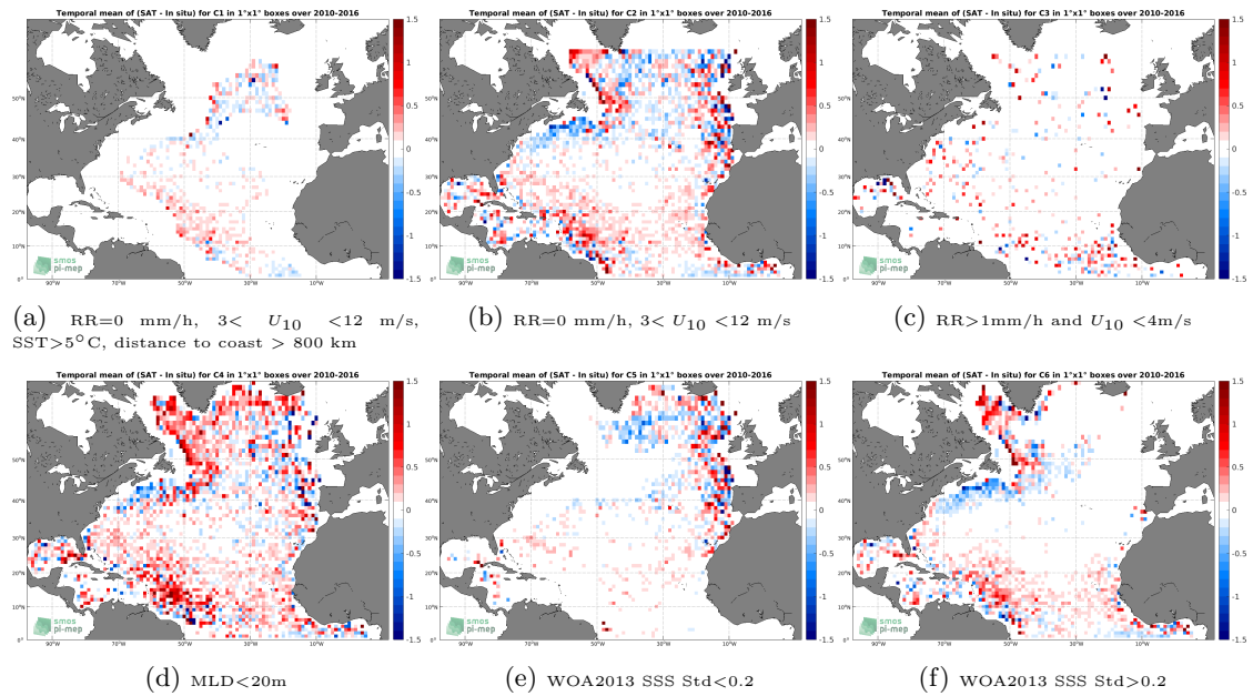
Figure 12: Temporal mean gridded over spatial boxes of size 1°x1° of \Delta SSS (SMOS SSS L3 v3 Monthly (ICDC) - Argo) for 6 different subdatasets corresponding to:RR=0 mm/h, 3 < U_{10} < 12 m/s, SST>5°C, distance to coast > 800 km (a), RR=0 mm/h, 3 < U_{10} < 12 m/s (b), RR>1mm/h and U_{10} < 4 m/s (c),MLD<20m (d),WOA2013 SSS Std<0.2 (e),WOA2013 SSS Std>0.2 (f).
