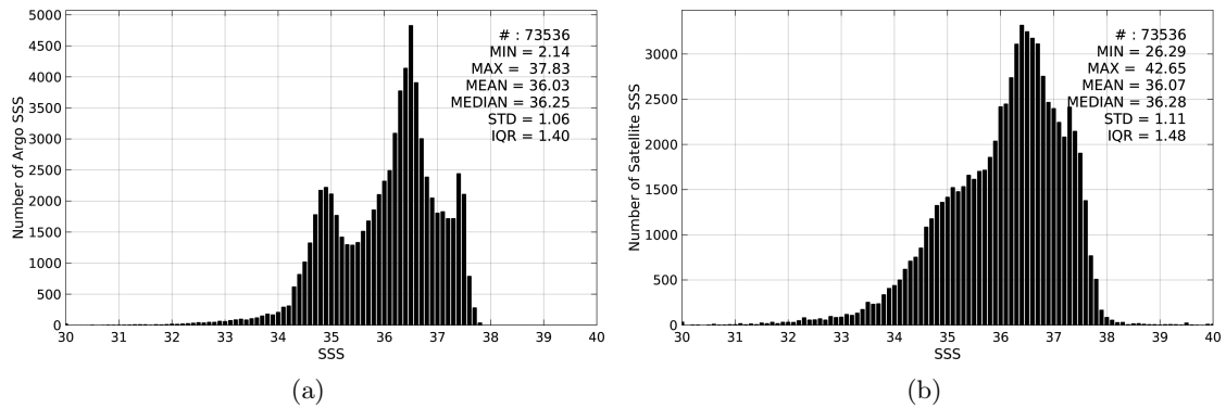
Figure 2: Histograms of SSS from Argo (a) and SMOS-L3-ICDC-V3-MONTHLY-0.5DEG (b) considering all match-up pairs per bins of 0.1 over the North Atlantic Ocean Pi-MEP region and for the full satellite product period.
