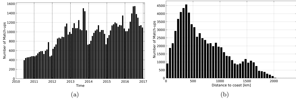
Figure 1: Number of match-ups between Argo and SMOS-L3-ICDC-V3-MONTHLY-0.5DEG SSS as a function of time (a) and as function of the distance to coast (b) over the North Atlantic Ocean Pi-MEP region and for the full satellite product period.
