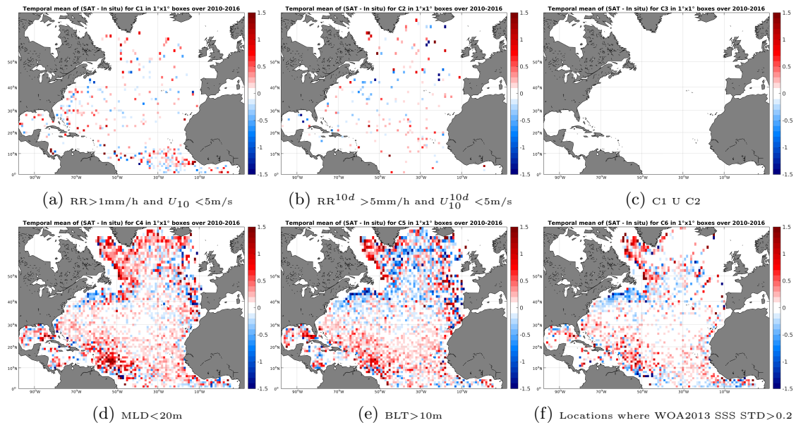
Figure 12: Temporal mean gridded over spatial boxes of size 1^\circ \times 1^\circ of \Delta SSS (SMOS-L3-ICDC-V3-MONTHLY-0.5DEG - Argo) for 6 different subdatasets corresponding to: RR > 1\text{mm/h} and U_{10} < 5\text{m/s} (a), RR^{10d} > 5\text{mm/h} and U_{10}^{10d} < 5\text{m/s} (b), C1 U C2 (c), MLD < 20\text{m} (d), BLT > 10\text{m} (e), Locations where WOA2013 SSS STD > 0.2 (f).
