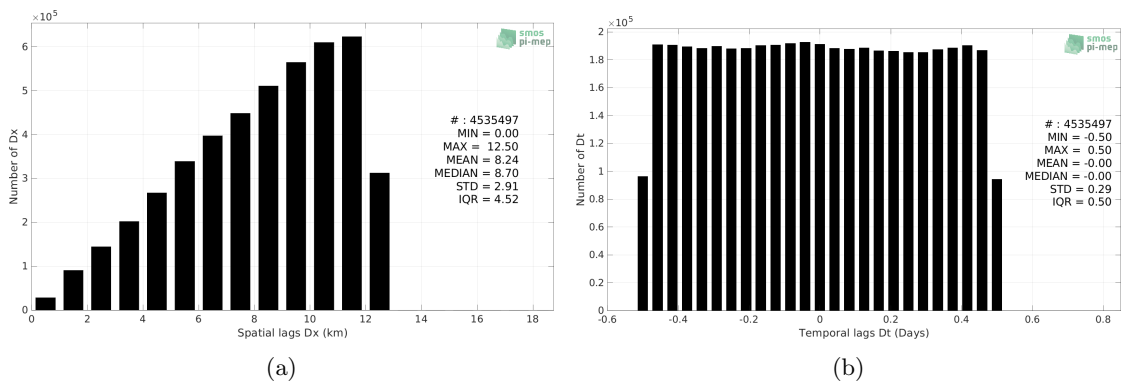
Figure 5: Histograms of the spatial (a) and temporal (b) lags between the location/time of the TSG (SAMOS) measurement and the date of the corresponding SMOS SSS L2Q v331 - With FLAG (CMEMS-CATDS-CPDC) SSS pixel.
