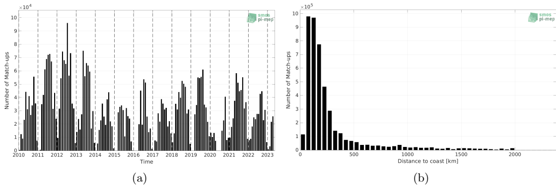
Figure 1: Number of match-ups between TSG (SAMOS) and SMOS SSS L2Q v331 - With FLAG (CMEMS-CATDS-CPDC) SSS as a function of time (a) and as function of the distance to coast (b) over the North Atlantic Ocean Pi-MEP region and for the full satellite product period.
