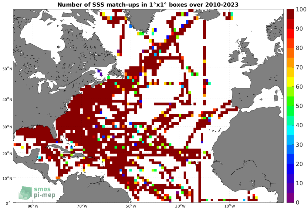
Figure 4: Number of SSS match-ups between TSG (SAMOS) SSS and the SMOS SSS L2Q v331 - With FLAG (CMEMS-CATDS-CPDC) SSS product for the North Atlantic Ocean Pi-MEP region over 1^\circ \times 1^\circ boxes and for the full satellite product period.
