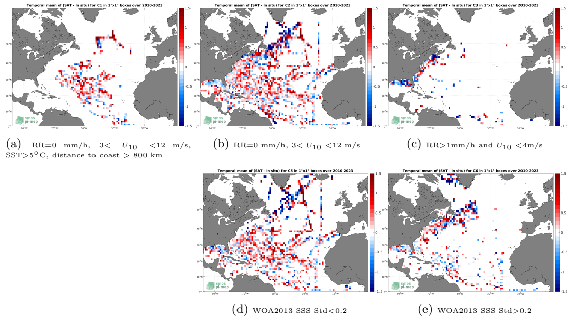
Figure 12: Temporal mean gridded over spatial boxes of size 1^\circ \times 1^\circ of \Delta\text{SSS} (SMOS SSS L2Q v331 - With FLAG (CMEMS-CATDS-CPDC) - TSG (SAMOS)) for 5 different subdatasets corresponding to:RR=0 mm/h, 3 < U_{10} < 12 m/s, SST >5^\circ\text{C} , distance to coast > 800 km (a), RR=0 mm/h, 3 < U_{10} < 12 m/s (b), RR >1 mm/h and U_{10} < 4 m/s (c), WOA2013 SSS Std <0.2 (d), WOA2013 SSS Std >0.2 (e).
