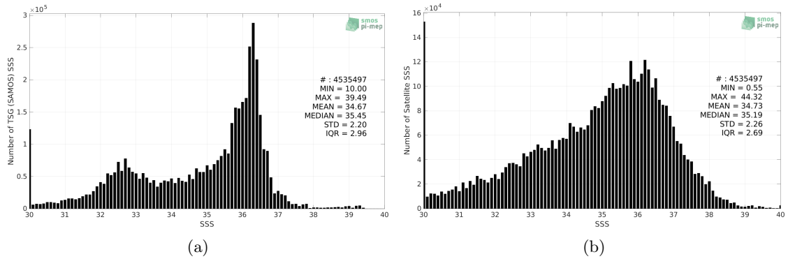
Figure 2: Histograms of SSS from TSG (SAMOS) (a) and SMOS SSS L2Q v331 - With FLAG (CMEMS-CATDS-CPDC) (b) considering all match-up pairs per bins of 0.1 over the North Atlantic Ocean Pi-MEP region and for the full satellite product period.
