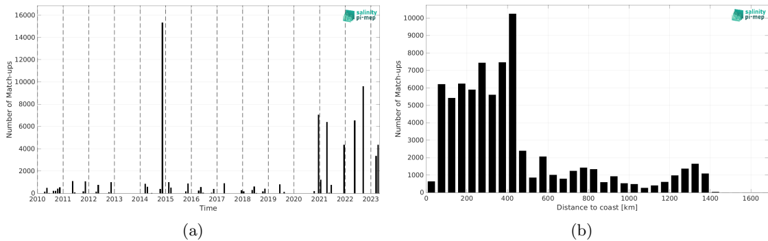
Figure 2: Number of match-ups between TSG (Polarstern) and SMOS SSS L2Q v331 - With FLAG (CMEMS-CATDS-CPDC) SSS as a function of time (a) and as function of the distance to coast (b) over the North Atlantic Ocean Pi-MEP region and for the full satellite product period.
