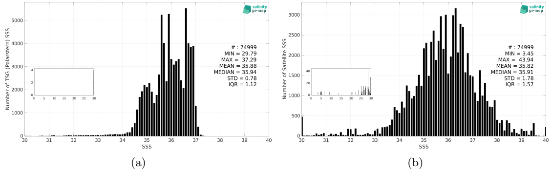
Figure 3: Histograms of SSS from TSG (Polarstern) (a) and SMOS SSS L2Q v331 - With FLAG (CMEMS-CATDS-CPDC) (b) considering all match-up pairs per bins of 0.1 over the North Atlantic Ocean Pi-MEP region and for the full satellite product period.
