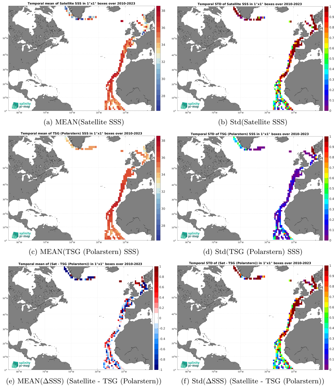
Figure 7: Temporal mean (left) and Std (right) of SSS from SMOS SSS L2Q v331 - With FLAG (CMEMS-CATDS-CPDC) (top), TSG (Polarstern) (middle), and of \Delta SSS (Satellite - TSG (Polarstern)). Only match-up pairs are used to generate these maps.
