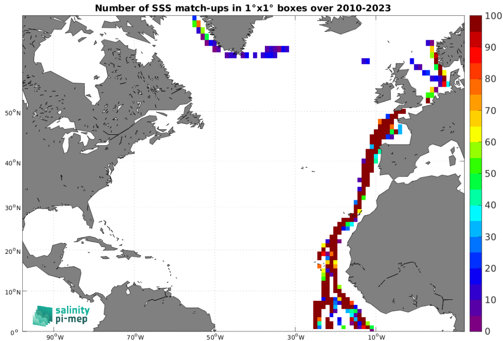
Figure 5: Number of SSS match-ups between TSG (Polarstern) SSS and the SMOS SSS L2Q v331 - With FLAG (CMEMS-CATDS-CPDC) SSS product for the North Atlantic Ocean Pi-MEP region over 1^\circ \times 1^\circ boxes and for the full satellite product period.
