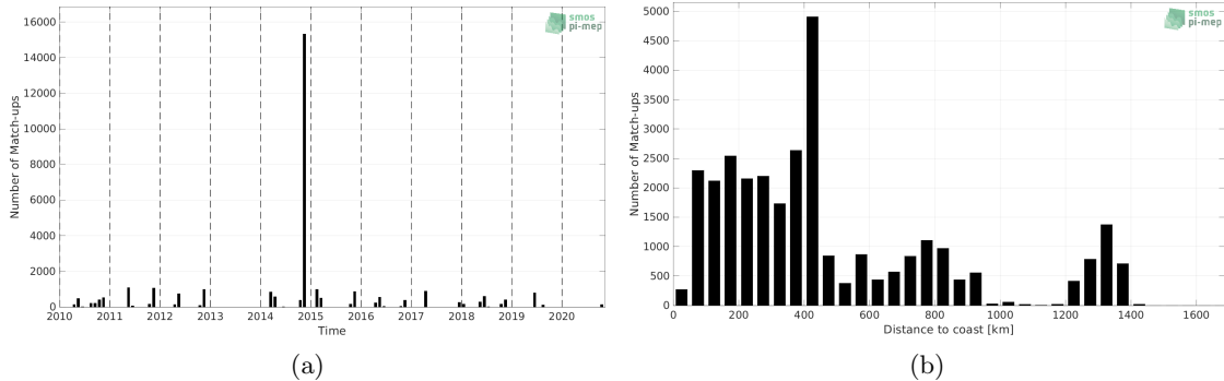
Figure 1: Number of match-ups between TSG (Polarstern) and SMOS SSS L2Q v331 - With FLAG (CMEMS-CATDS-CPDC) SSS as a function of time (a) and as function of the distance to coast (b) over the North Atlantic Ocean Pi-MEP region and for the full satellite product period.
