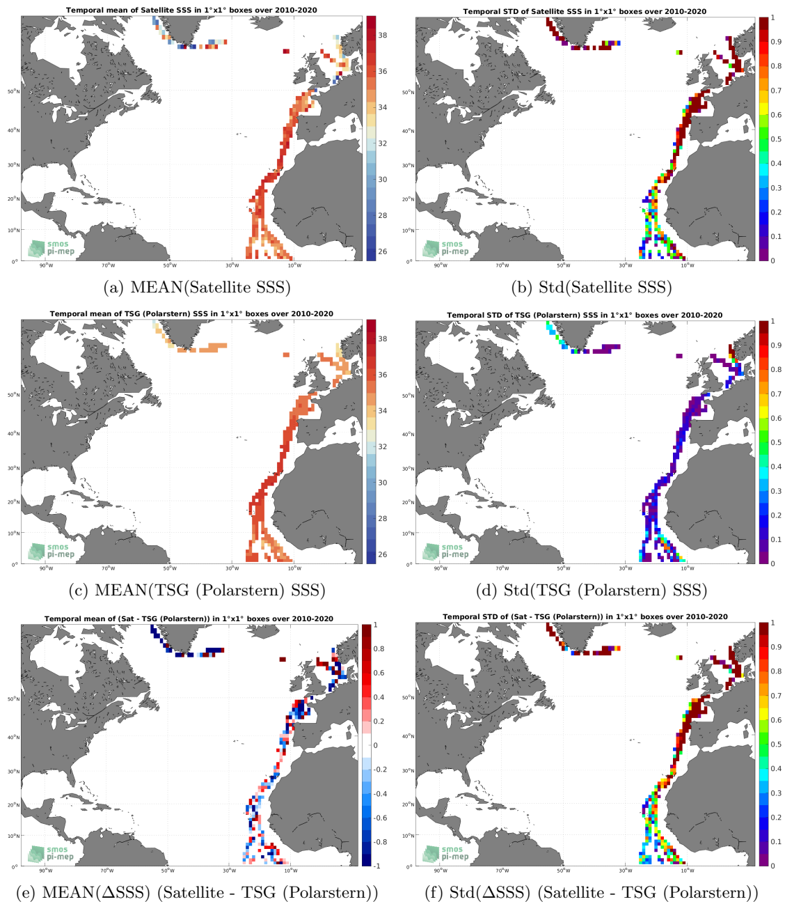
Figure 6: Temporal mean (left) and Std (right) of SSS from SMOS SSS L2Q v331 - With FLAG (CMEMS-CATDS-CPDC) (top), TSG (Polarstern) (middle), and of \Delta SSS (Satellite - TSG (Polarstern)). Only match-up pairs are used to generate these maps.
