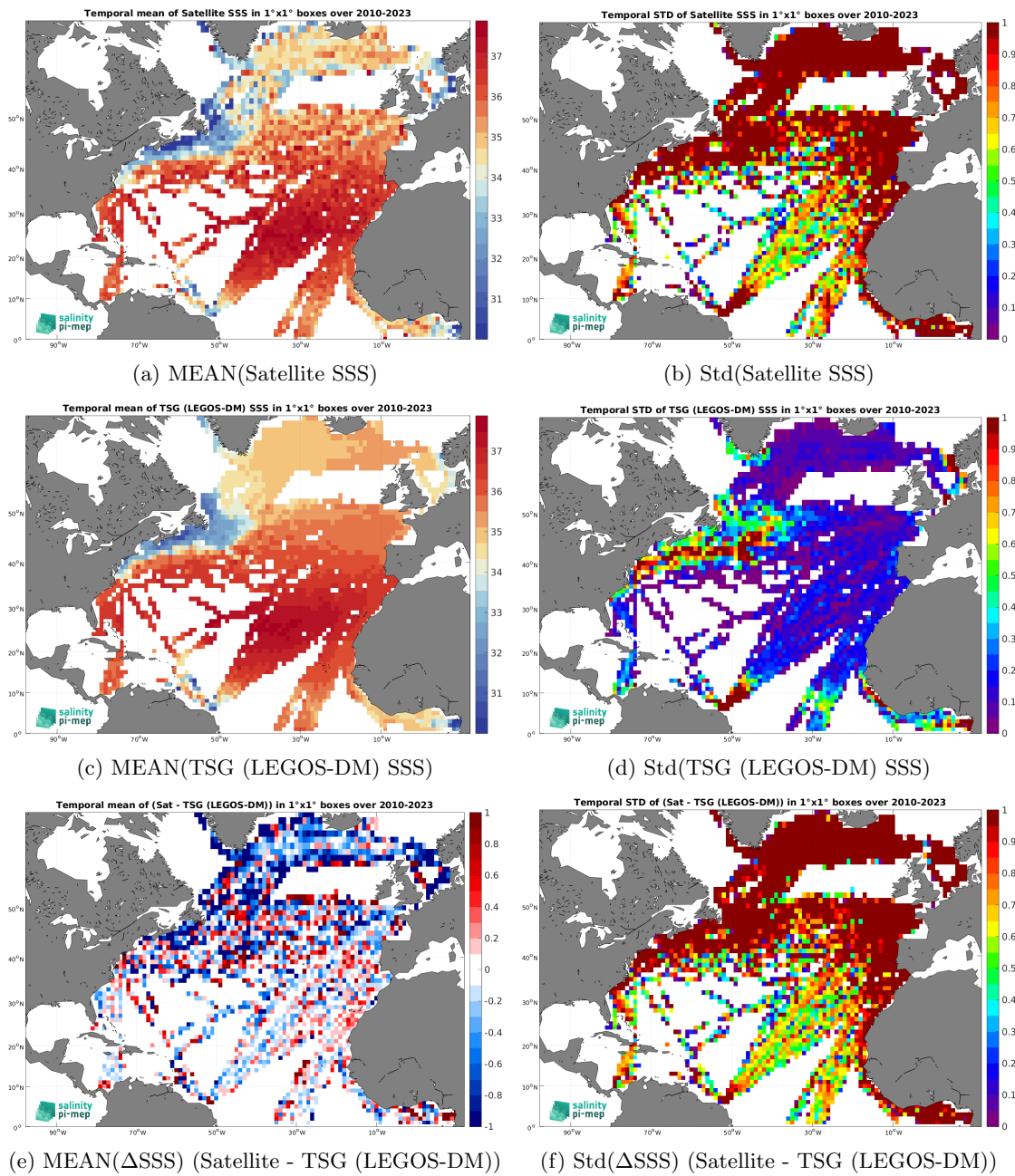
Figure 7: Temporal mean (left) and Std (right) of SSS from SMOS SSS L2Q v331 - With FLAG (CMEMS-CATDS-CPDC) (top), TSG (LEGOS-DM) (middle), and of \Delta SSS (Satellite - TSG (LEGOS-DM)). Only match-up pairs are used to generate these maps.
