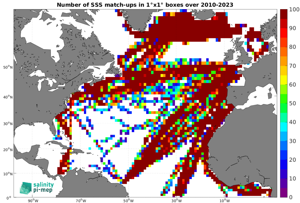
Figure 5: Number of SSS match-ups between TSG (LEGOS-DM) SSS and the SMOS SSS L2Q v331 - With FLAG (CMEMS-CATDS-CPDC) SSS product for the North Atlantic Ocean Pi-MEP region over 1^\circ \times 1^\circ boxes and for the full satellite product period.
