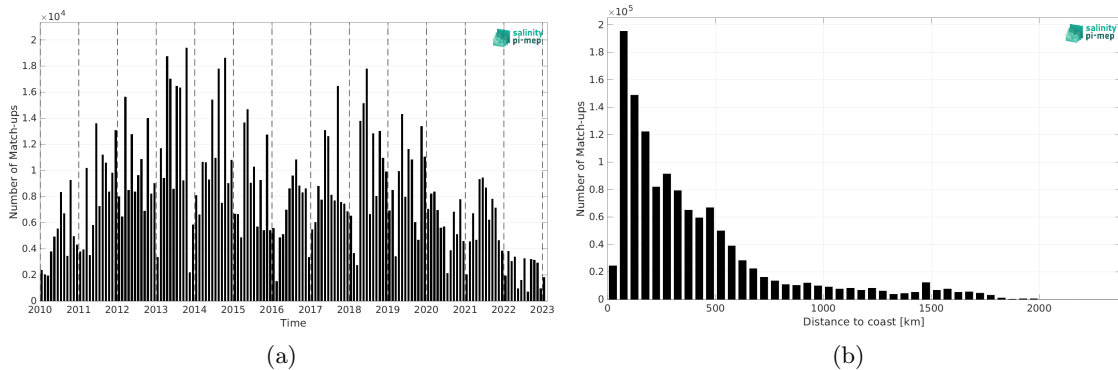
Figure 2: Number of match-ups between TSG (LEGOS-DM) and SMOS SSS L2Q v331 - With FLAG (CMEMS-CATDS-CPDC) SSS as a function of time (a) and as function of the distance to coast (b) over the North Atlantic Ocean Pi-MEP region and for the full satellite product period.
