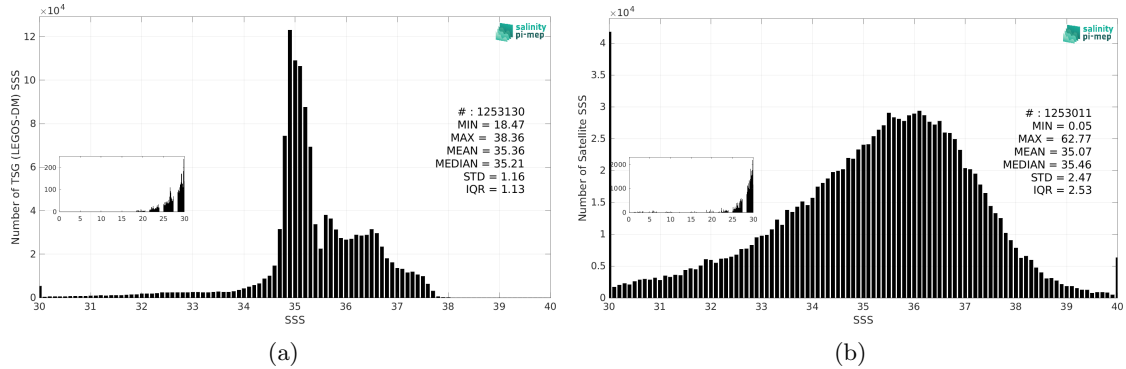
Figure 3: Histograms of SSS from TSG (LEGOS-DM) (a) and SMOS SSS L2Q v331 - With FLAG (CMEMS-CATDS-CPDC) (b) considering all match-up pairs per bins of 0.1 over the North Atlantic Ocean Pi-MEP region and for the full satellite product period.
