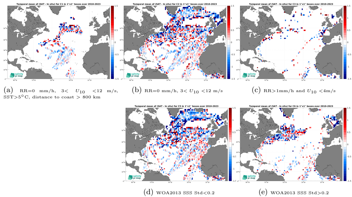
Figure 14: Temporal mean gridded over spatial boxes of size 1^\circ \times 1^\circ of \Delta\text{SSS} (SMOS SSS L2Q v331 - With FLAG (CMEMS-CATDS-CPDC) - TSG (LEGOS-DM)) for 5 different subdatasets corresponding to:RR=0 mm/h, 3 < U_{10} < 12 m/s, SST >5^\circ\text{C} , distance to coast > 800 km (a), RR=0 mm/h, 3 < U_{10} < 12 m/s (b), RR >1 mm/h and U_{10} < 4 m/s (c), WOA2013 SSS Std <0.2 (d), WOA2013 SSS Std >0.2 (e).
