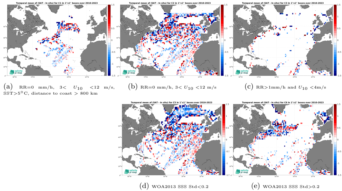
Figure 12: Temporal mean gridded over spatial boxes of size 1^\circ \times 1^\circ of \Delta\text{SSS} (SMOS SSS L2Q v331 - With FLAG (CMEMS-CATDS-CPDC) - TSG (LEGOS-DM)) for 5 different subdatasets corresponding to:RR=0 mm/h, 3 < U_{10} < 12 m/s, SST >5^\circ\text{C} , distance to coast > 800 km (a), RR=0 mm/h, 3 < U_{10} < 12 m/s (b), RR >1 mm/h and U_{10} < 4 m/s (c), WOA2013 SSS Std <0.2 (d), WOA2013 SSS Std >0.2 (e).
