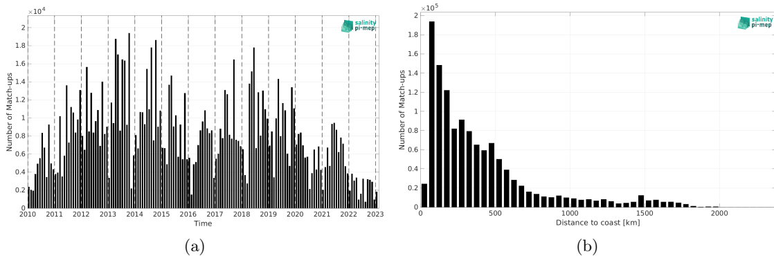
Figure 1: Number of match-ups between TSG (LEGOS-DM) and SMOS SSS L2Q v331 - With FLAG (CMEMS-CATDS-CPDC) SSS as a function of time (a) and as function of the distance to coast (b) over the North Atlantic Ocean Pi-MEP region and for the full satellite product period.
