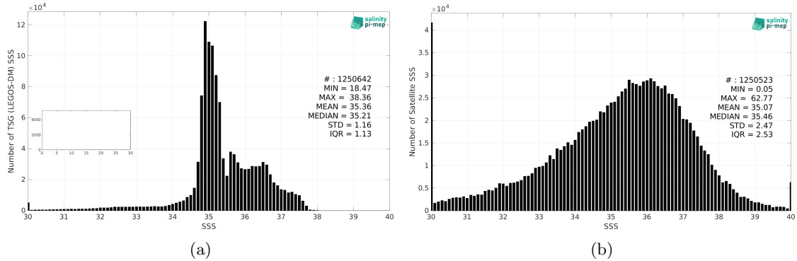
Figure 2: Histograms of SSS from TSG (LEGOS-DM) (a) and SMOS SSS L2Q v331 - With FLAG (CMEMS-CATDS-CPDC) (b) considering all match-up pairs per bins of 0.1 over the North Atlantic Ocean Pi-MEP region and for the full satellite product period.
