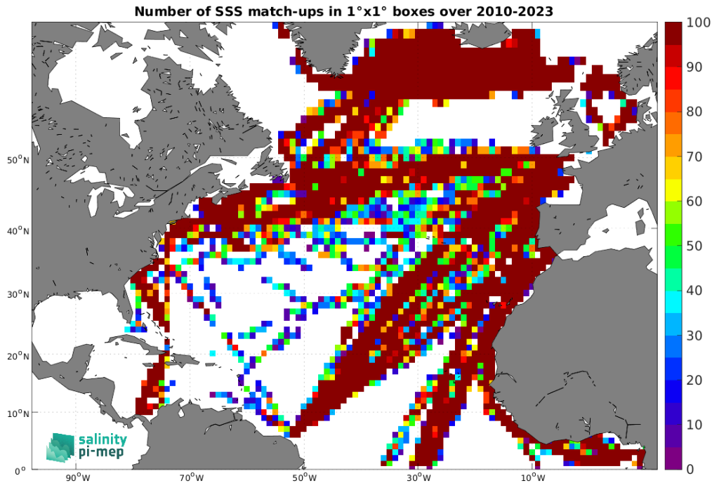
Figure 4: Number of SSS match-ups between TSG (LEGOS-DM) SSS and the SMOS SSS L2Q v331 - With FLAG (CMEMS-CATDS-CPDC) SSS product for the North Atlantic Ocean Pi-MEP region over 1^\circ \times 1^\circ boxes and for the full satellite product period.
