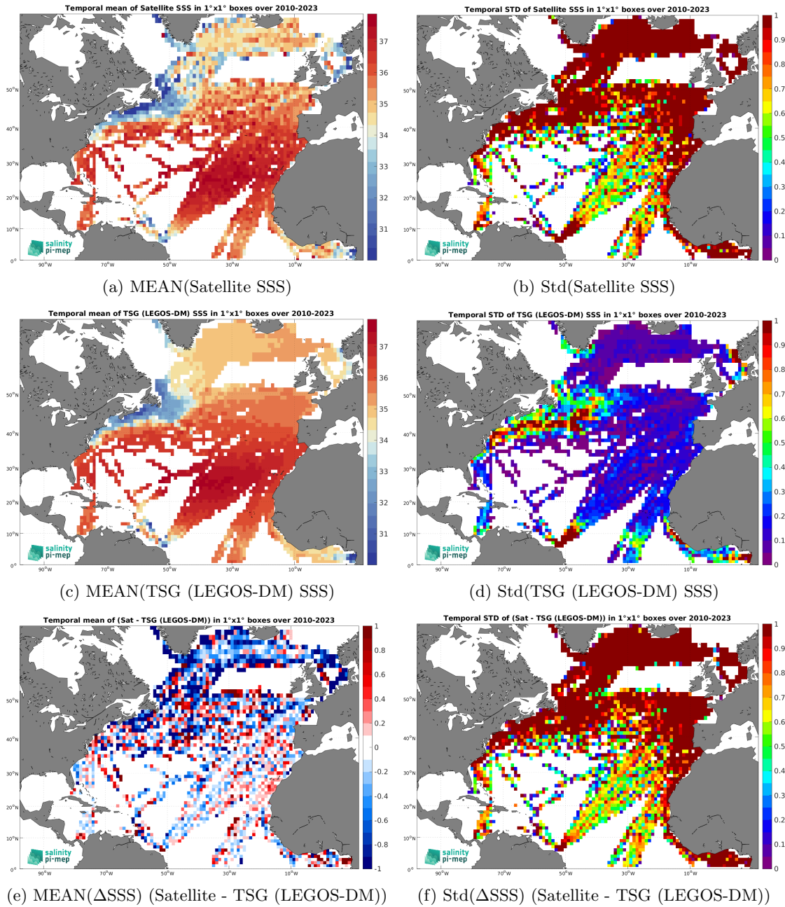
Figure 6: Temporal mean (left) and Std (right) of SSS from SMOS SSS L2Q v331 - With FLAG (CMEMS-CATDS-CPDC) (top), TSG (LEGOS-DM) (middle), and of \Delta SSS (Satellite - TSG (LEGOS-DM)). Only match-up pairs are used to generate these maps.
