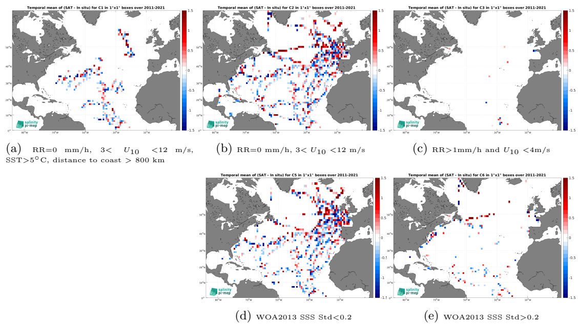
Figure 14: Temporal mean gridded over spatial boxes of size 1^\circ \times 1^\circ of \Delta\text{SSS} (SMOS SSS L2Q v331 - With FLAG (CMEMS-CATDS-CPDC) - TSG (GOSUD-Sailing-ship)) for 5 different subdatasets corresponding to:RR=0 mm/h, 3 < U_{10} < 12 m/s, SST>5°C, distance to coast > 800 km (a), RR=0 mm/h, 3 < U_{10} < 12 m/s (b), RR>1mm/h and U_{10} < 4 m/s (c), WOA2013 SSS Std<0.2 (d), WOA2013 SSS Std>0.2 (e).
