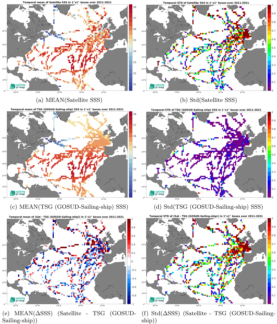
Figure 7: Temporal mean (left) and Std (right) of SSS from SMOS SSS L2Q v331 - With FLAG (CMEMS-CATDS-CPDC) (top), TSG (GOSUD-Sailing-ship) (middle), and of \Delta SSS (Satellite - TSG (GOSUD-Sailing-ship)). Only match-up pairs are used to generate these maps.
