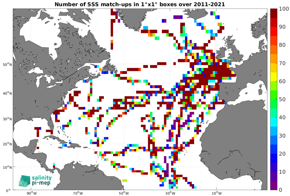
Figure 5: Number of SSS match-ups between TSG (GOSUD-Sailing-ship) SSS and the SMOS SSS L2Q v331 - With FLAG (CMEMS-CATDS-CPDC) SSS product for the North Atlantic Ocean Pi-MEP region over 1^\circ \times 1^\circ boxes and for the full satellite product period.
