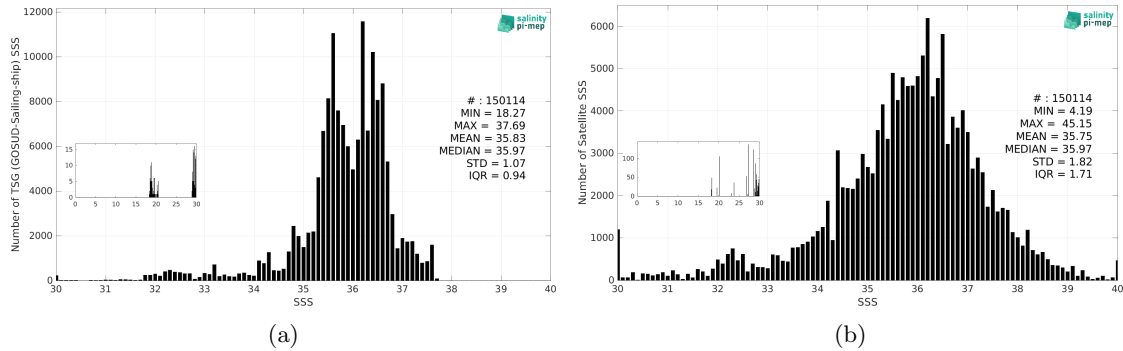
Figure 3: Histograms of SSS from TSG (GOSUD-Sailing-ship) (a) and SMOS SSS L2Q v331 - With FLAG (CMEMS-CATDS-CPDC) (b) considering all match-up pairs per bins of 0.1 over the North Atlantic Ocean Pi-MEP region and for the full satellite product period.
