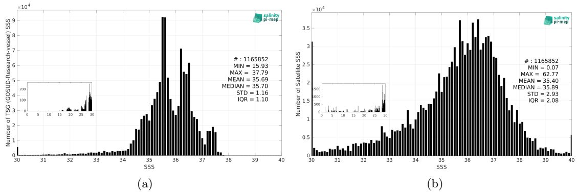
Figure 3: Histograms of SSS from TSG (GOSUD-Research-vessel) (a) and SMOS SSS L2Q v331 - With FLAG (CMEMS-CATDS-CPDC) (b) considering all match-up pairs per bins of 0.1 over the North Atlantic Ocean Pi-MEP region and for the full satellite product period.
