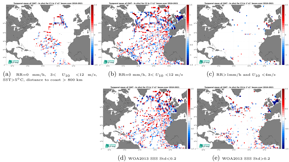
Figure 14: Temporal mean gridded over spatial boxes of size 1^\circ \times 1^\circ of \Delta\text{SSS} (SMOS SSS L2Q v331 - With FLAG (CMEMS-CATDS-CPDC) - TSG (GOSUD-Research-vessel)) for 5 different subdatasets corresponding to:RR=0 mm/h, 3 < U_{10} < 12 m/s, SST > 5°C, distance to coast > 800 km (a), RR=0 mm/h, 3 < U_{10} < 12 m/s (b), RR > 1mm/h and U_{10} < 4 m/s (c), WOA2013 SSS Std < 0.2 (d), WOA2013 SSS Std > 0.2 (e).
