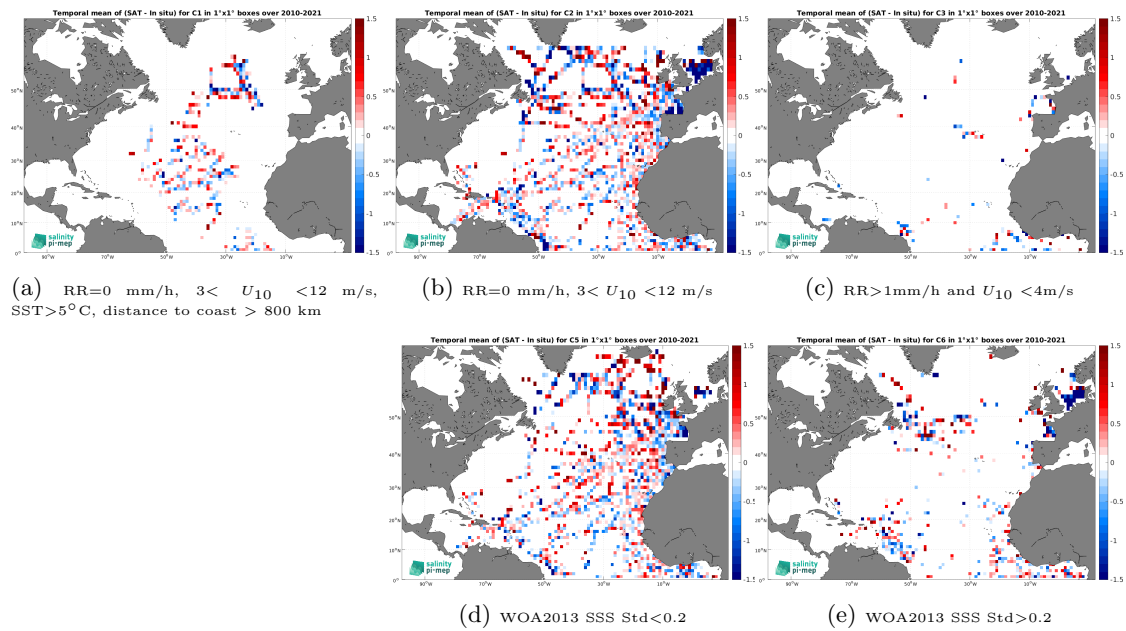
Figure 12: Temporal mean gridded over spatial boxes of size 1^\circ \times 1^\circ of \Delta\text{SSS} (SMOS SSS L2Q v331 - With FLAG (CMEMS-CATDS-CPDC) - TSG (GOSUD-Research-vessel)) for 5 different subdatasets corresponding to:RR=0 mm/h, 3 < U_{10} < 12 m/s, SST > 5°C, distance to coast > 800 km (a), RR=0 mm/h, 3 < U_{10} < 12 m/s (b), RR > 1mm/h and U_{10} < 4 m/s (c), WOA2013 SSS Std < 0.2 (d), WOA2013 SSS Std > 0.2 (e).
