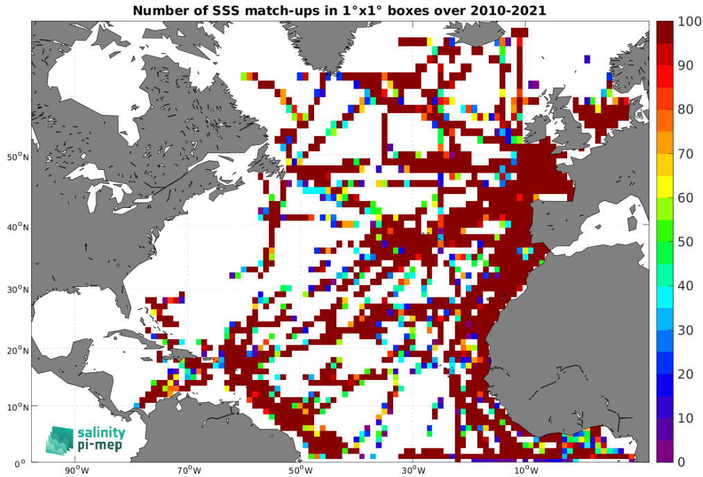
Figure 4: Number of SSS match-ups between TSG (GOSUD-Research-vessel) SSS and the SMOS SSS L2Q v331 - With FLAG (CMEMS-CATDS-CPDC) SSS product for the North Atlantic Ocean Pi-MEP region over 1^\circ \times 1^\circ boxes and for the full satellite product period.
