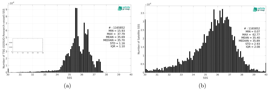
Figure 2: Histograms of SSS from TSG (GOSUD-Research-vessel) (a) and SMOS SSS L2Q v331 - With FLAG (CMEMS-CATDS-CPDC) (b) considering all match-up pairs per bins of 0.1 over the North Atlantic Ocean Pi-MEP region and for the full satellite product period.
