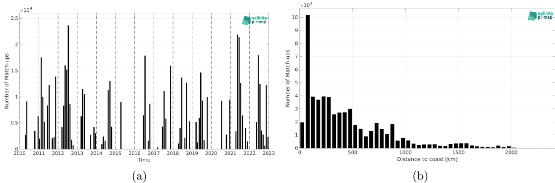
Figure 2: Number of match-ups between TSG (CSIC-UTM) and SMOS SSS L2Q v331 - With FLAG (CMEMS-CATDS-CPDC) SSS as a function of time (a) and as function of the distance to coast (b) over the North Atlantic Ocean Pi-MEP region and for the full satellite product period.
