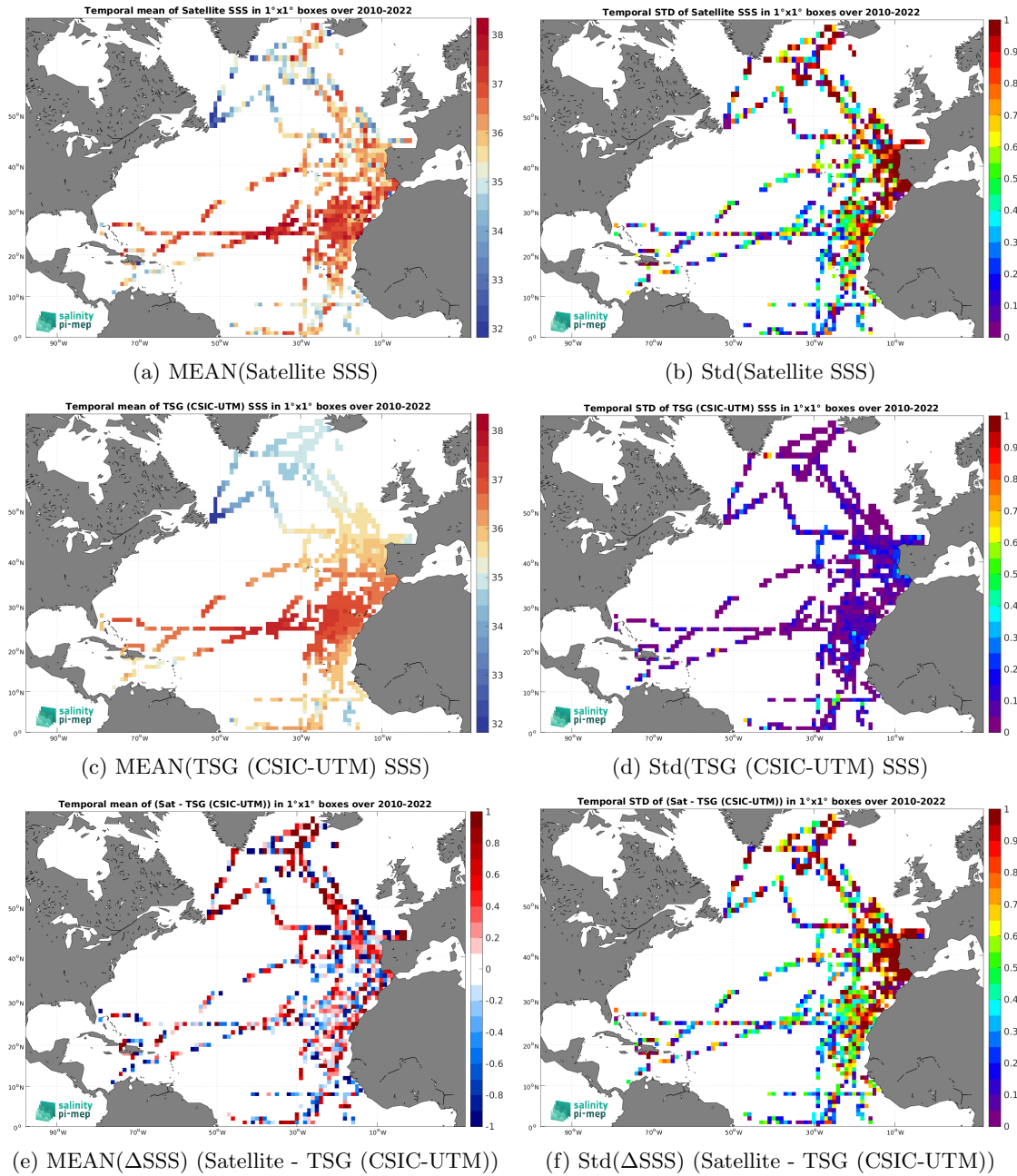
Figure 7: Temporal mean (left) and Std (right) of SSS from SMOS SSS L2Q v331 - With FLAG (CMEMS-CATDS-CPDC) (top), TSG (CSIC-UTM) (middle), and of \Delta SSS (Satellite - TSG (CSIC-UTM)). Only match-up pairs are used to generate these maps.
