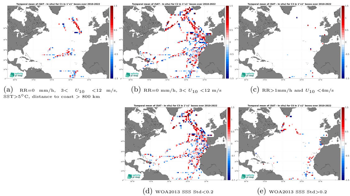
Figure 14: Temporal mean gridded over spatial boxes of size 1^\circ \times 1^\circ of \Delta\text{SSS} (SMOS SSS L2Q v331 - With FLAG (CMEMS-CATDS-CPDC) - TSG (CSIC-UTM)) for 5 different subdatasets corresponding to:RR=0 mm/h, 3 < U_{10} < 12 m/s, SST >5^\circ\text{C} , distance to coast > 800 km (a), RR=0 mm/h, 3 < U_{10} < 12 m/s (b), RR >1 mm/h and U_{10} < 4 m/s (c), WOA2013 SSS Std <0.2 (d), WOA2013 SSS Std >0.2 (e).
