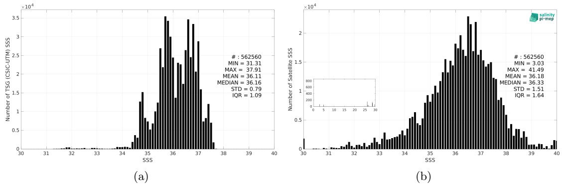
Figure 3: Histograms of SSS from TSG (CSIC-UTM) (a) and SMOS SSS L2Q v331 - With FLAG (CMEMS-CATDS-CPDC) (b) considering all match-up pairs per bins of 0.1 over the North Atlantic Ocean Pi-MEP region and for the full satellite product period.
