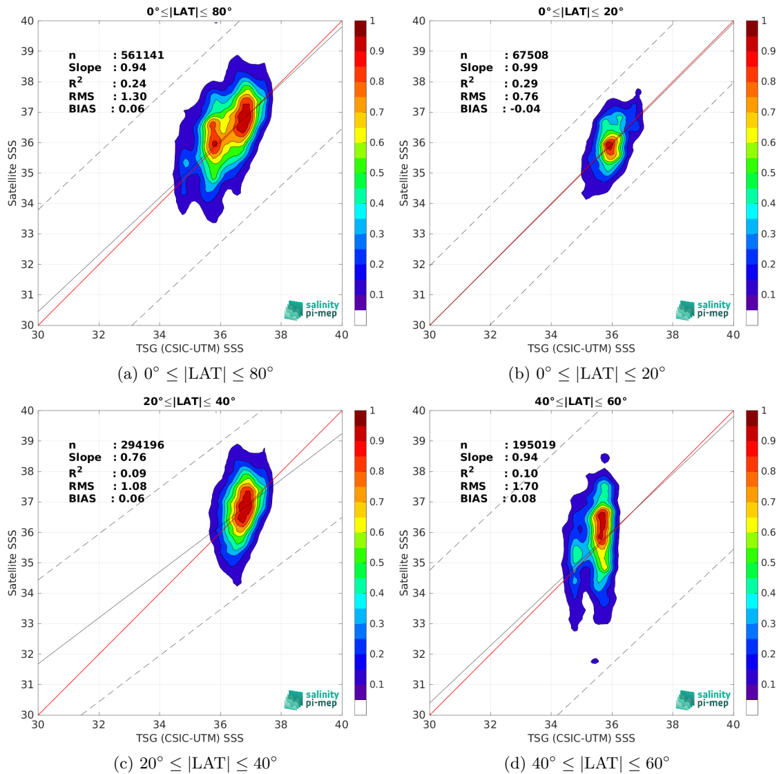
Figure 9: Contour maps of the concentration of SMOS SSS L2Q v331 - With FLAG (CMEMS-CATDS-CPDC) SSS ( y -axis) versus TSG (CSIC-UTM) SSS ( x -axis) at match-up pairs for different latitude bands. For each plot, the red line shows x=y . The black thin and dashed lines indicate a linear fit through the data cloud and the \pm 95\% confidence levels, respectively. The number match-up pairs n , the slope and R^2 coefficient of the linear fit, the root mean square (RMS) and the mean bias between satellite and in situ data are indicated for each latitude band in each plots.
