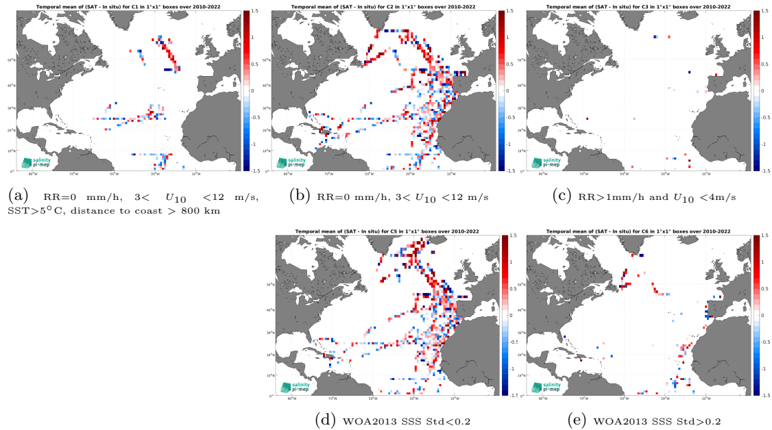
Figure 12: Temporal mean gridded over spatial boxes of size 1^\circ \times 1^\circ of \Delta\text{SSS} (SMOS SSS L2Q v331 - With FLAG (CMEMS-CATDS-CPDC) - TSG (CSIC-UTM)) for 5 different subdatasets corresponding to:RR=0 mm/h, 3 < U_{10} < 12 m/s, SST >5^\circ\text{C} , distance to coast > 800 km (a), RR=0 mm/h, 3 < U_{10} < 12 m/s (b), RR >1 mm/h and U_{10} < 4 m/s (c), WOA2013 SSS Std <0.2 (d), WOA2013 SSS Std >0.2 (e).
