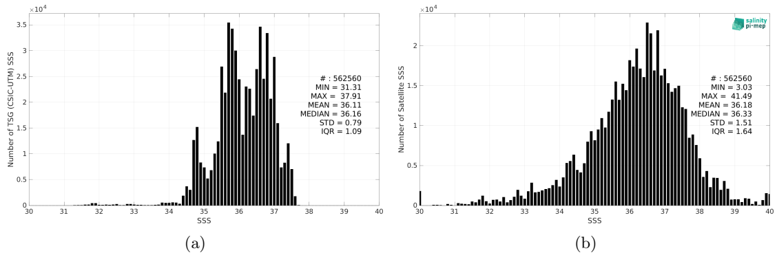
Figure 2: Histograms of SSS from TSG (CSIC-UTM) (a) and SMOS SSS L2Q v331 - With FLAG (CMEMS-CATDS-CPDC) (b) considering all match-up pairs per bins of 0.1 over the North Atlantic Ocean Pi-MEP region and for the full satellite product period.
