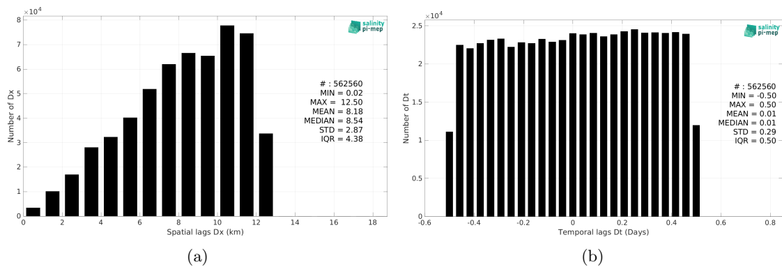
Figure 5: Histograms of the spatial (a) and temporal (b) lags between the location/time of the TSG (CSIC-UTM) measurement and the date of the corresponding SMOS SSS L2Q v331 - With FLAG (CMEMS-CATDS-CPDC) SSS pixel.
