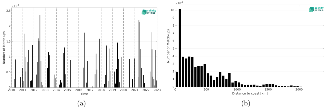
Figure 1: Number of match-ups between TSG (CSIC-UTM) and SMOS SSS L2Q v331 - With FLAG (CMEMS-CATDS-CPDC) SSS as a function of time (a) and as function of the distance to coast (b) over the North Atlantic Ocean Pi-MEP region and for the full satellite product period.
