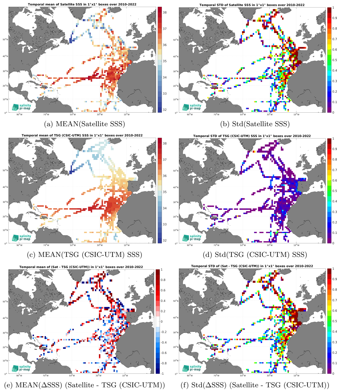
Figure 6: Temporal mean (left) and Std (right) of SSS from SMOS SSS L2Q v331 - With FLAG (CMEMS-CATDS-CPDC) (top), TSG (CSIC-UTM) (middle), and of \Delta SSS (Satellite - TSG (CSIC-UTM)). Only match-up pairs are used to generate these maps.
