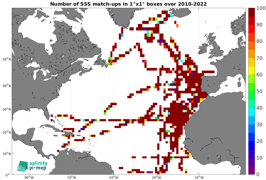
Figure 4: Number of SSS match-ups between TSG (CSIC-UTM) SSS and the SMOS SSS L2Q v331 - With FLAG (CMEMS-CATDS-CPDC) SSS product for the North Atlantic Ocean Pi-MEP region over 1^\circ \times 1^\circ boxes and for the full satellite product period.
