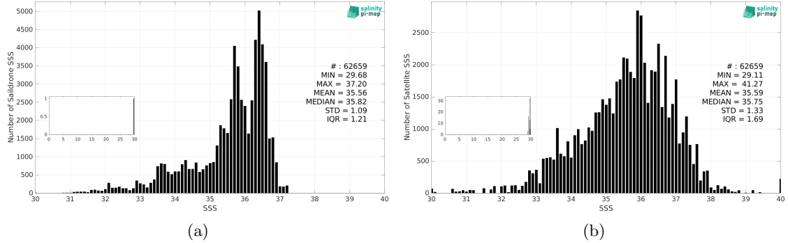
Figure 3: Histograms of SSS from Saildrone (a) and SMOS SSS L2Q v331 - With FLAG (CMEMS-CATDS-CPDC) (b) considering all match-up pairs per bins of 0.1 over the North Atlantic Ocean Pi-MEP region and for the full satellite product period.
