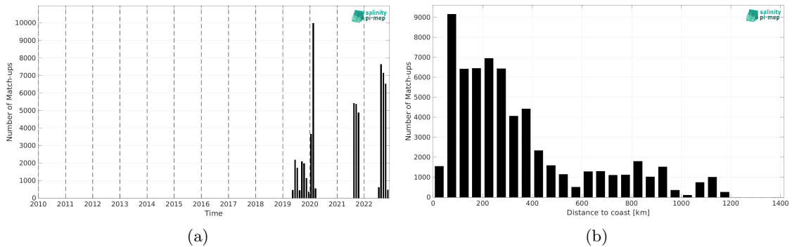
Figure 2: Number of match-ups between Saildrone and SMOS SSS L2Q v331 - With FLAG (CMEMS-CATDS-CPDC) SSS as a function of time (a) and as function of the distance to coast (b) over the North Atlantic Ocean Pi-MEP region and for the full satellite product period.
