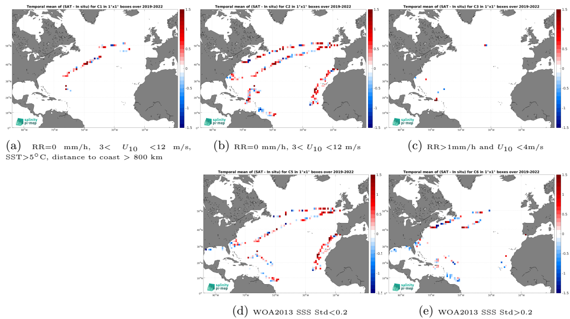
Figure 14: Temporal mean gridded over spatial boxes of size 1^\circ \times 1^\circ of \Delta\text{SSS} (SMOS SSS L2Q v331 - With FLAG (CMEMS-CATDS-CPDC) - Saildrone) for 5 different subdatasets corresponding to:RR=0 mm/h, 3 < U_{10} < 12 m/s, SST > 5°C, distance to coast > 800 km (a), RR=0 mm/h, 3 < U_{10} < 12 m/s (b), RR > 1mm/h and U_{10} < 4 m/s (c), WOA2013 SSS Std < 0.2 (d), WOA2013 SSS Std > 0.2 (e).
