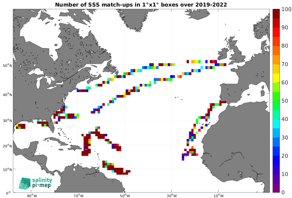
Figure 5: Number of SSS match-ups between Saildrone SSS and the SMOS SSS L2Q v331 - With FLAG (CMEMS-CATDS-CPDC) SSS product for the North Atlantic Ocean Pi-MEP region over 1^\circ \times 1^\circ boxes and for the full satellite product period.
