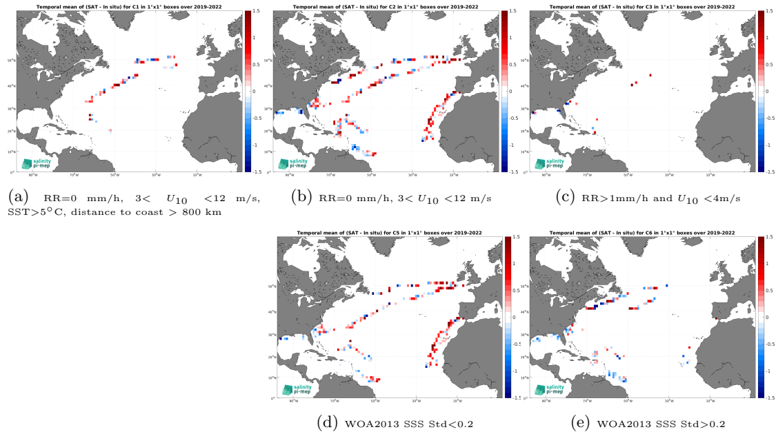
Figure 12: Temporal mean gridded over spatial boxes of size 1^\circ \times 1^\circ of \Delta\text{SSS} (SMOS SSS L2Q v331 - With FLAG (CMEMS-CATDS-CPDC) - Saildrone) for 5 different subdatasets corresponding to:RR=0 mm/h, 3 < U_{10} < 12 m/s, SST >5^\circ\text{C} , distance to coast > 800 km (a), RR=0 mm/h, 3 < U_{10} < 12 m/s (b), RR >1 mm/h and U_{10} < 4 m/s (c), WOA2013 SSS Std <0.2 (d), WOA2013 SSS Std >0.2 (e).
