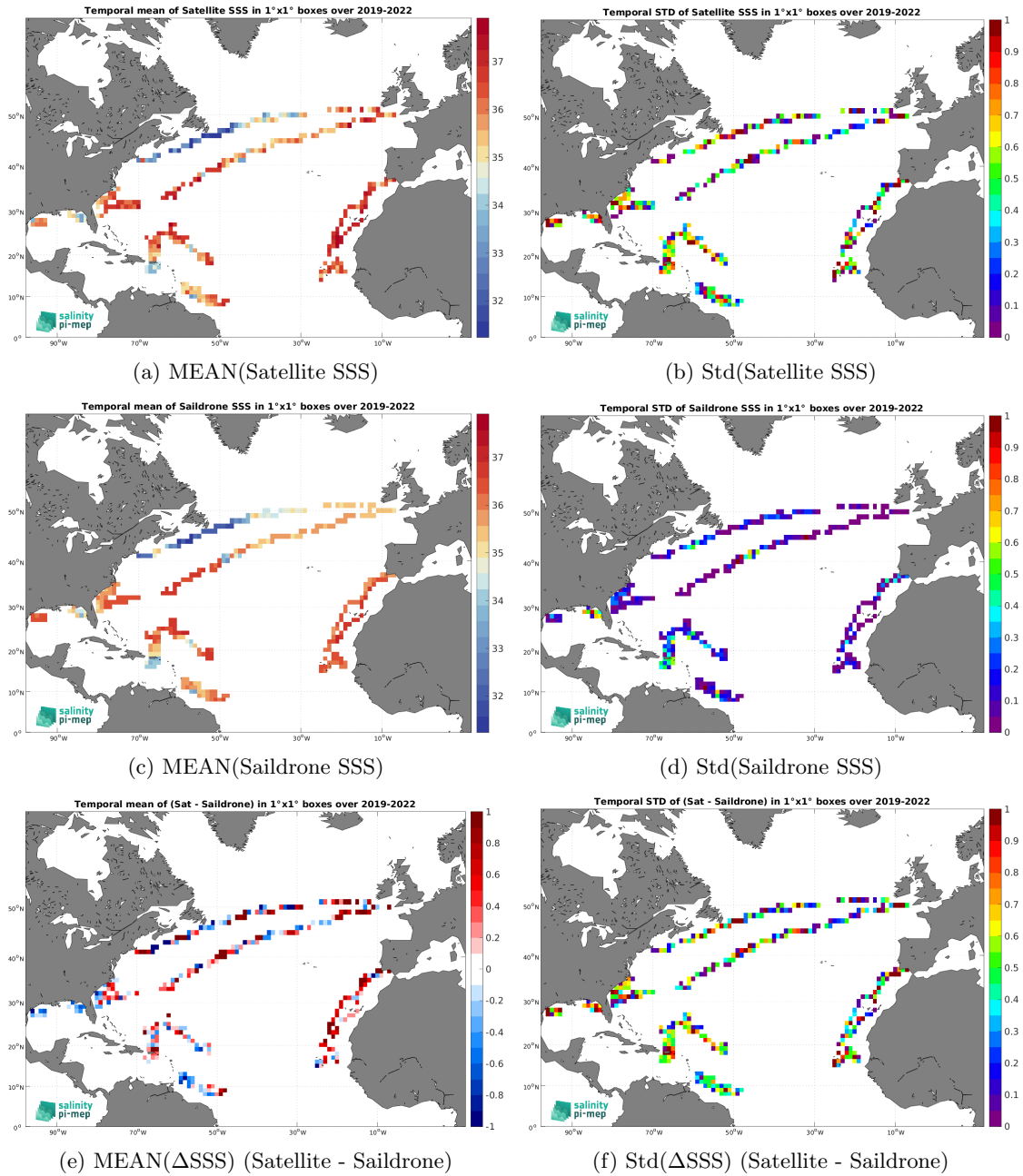
Figure 6: Temporal mean (left) and Std (right) of SSS from SMOS SSS L2Q v331 - With FLAG (CMEMS-CATDS-CPDC) (top), Saildrone (middle), and of \Delta SSS (Satellite - Saildrone). Only match-up pairs are used to generate these maps.
