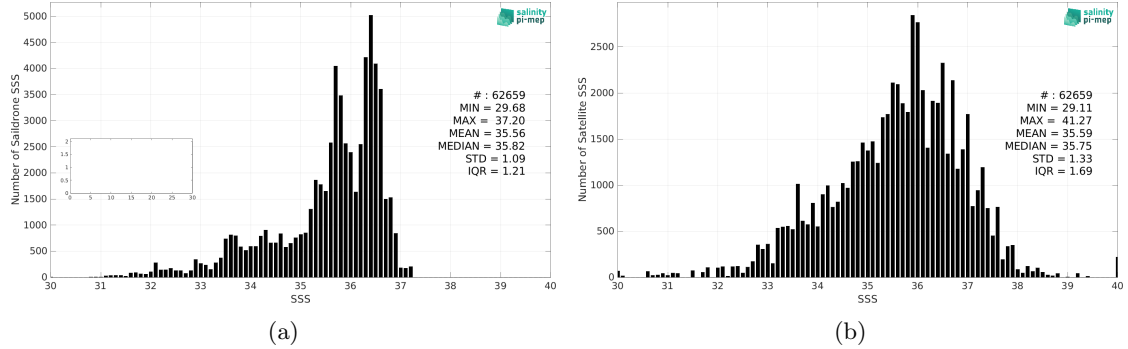
Figure 2: Histograms of SSS from Saildrone (a) and SMOS SSS L2Q v331 - With FLAG (CMEMS-CATDS-CPDC) (b) considering all match-up pairs per bins of 0.1 over the North Atlantic Ocean Pi-MEP region and for the full satellite product period.
