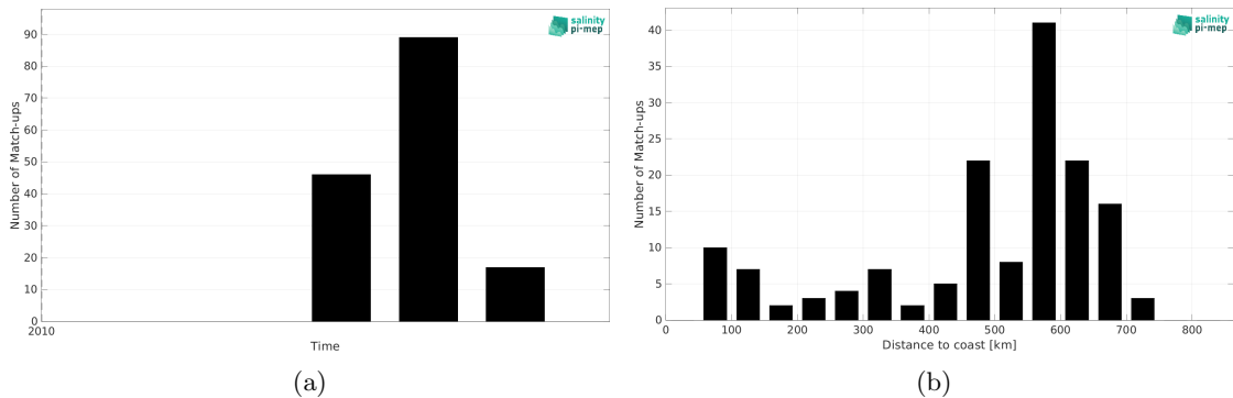
Figure 2: Number of match-ups between Marine mammals and SMOS SSS L2Q v331 - With FLAG (CMEMS-CATDS-CPDC) SSS as a function of time (a) and as function of the distance to coast (b) over the North Atlantic Ocean Pi-MEP region and for the full satellite product period.
