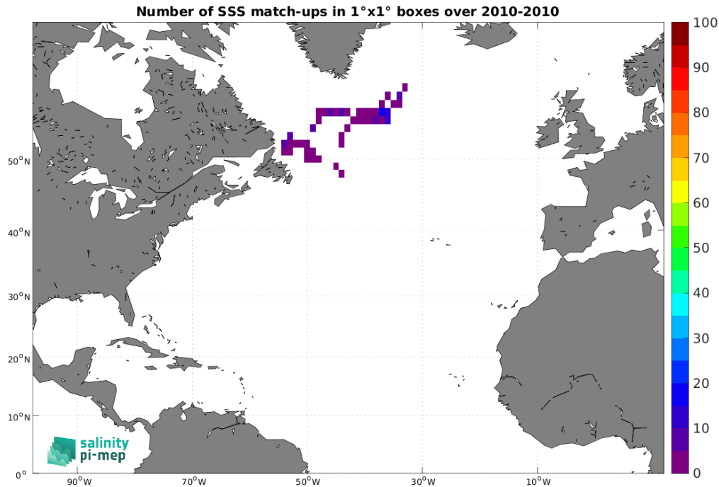
Figure 5: Number of SSS match-ups between Marine mammals SSS and the SMOS SSS L2Q v331 - With FLAG (CMEMS-CATDS-CPDC) SSS product for the North Atlantic Ocean Pi-MEP region over 1^\circ \times 1^\circ boxes and for the full satellite product period.
