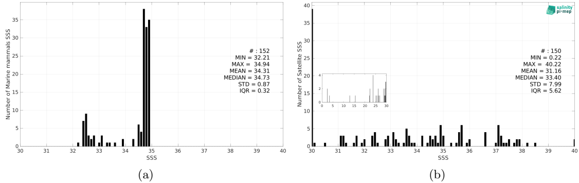
Figure 3: Histograms of SSS from Marine mammals (a) and SMOS SSS L2Q v331 - With FLAG (CMEMS-CATDS-CPDC) (b) considering all match-up pairs per bins of 0.1 over the North Atlantic Ocean Pi-MEP region and for the full satellite product period.
