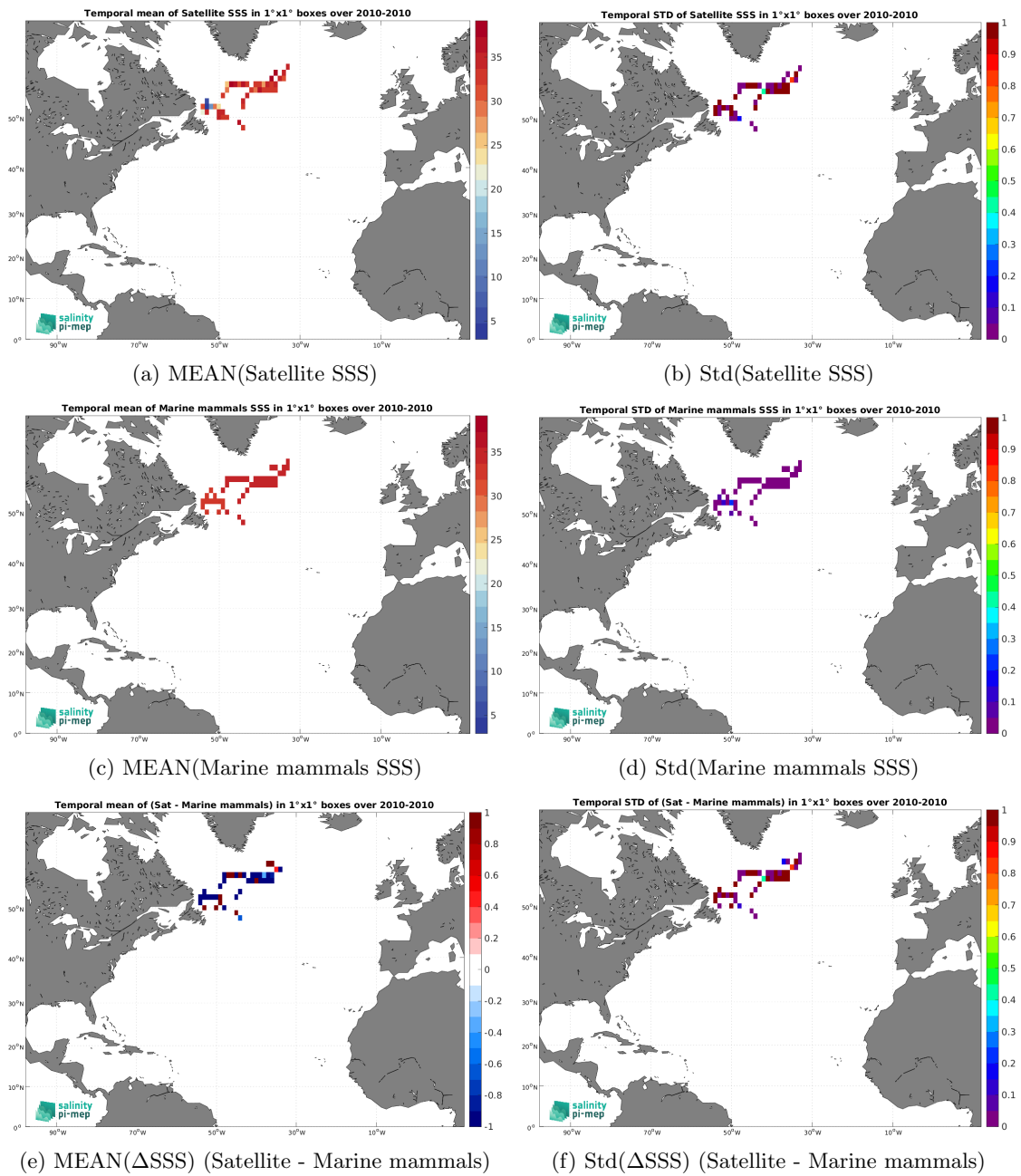
Figure 7: Temporal mean (left) and Std (right) of SSS from SMOS SSS L2Q v331 - With FLAG (CMEMS-CATDS-CPDC) (top), Marine mammals (middle), and of \Delta SSS (Satellite - Marine mammals). Only match-up pairs are used to generate these maps.
