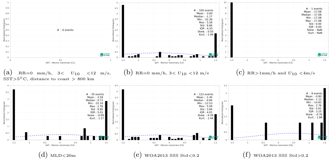
Figure 15: Normalized histogram of \Delta SSS (SMOS SSS L2Q v331 - With FLAG (CMEMS-CATDS-CPDC) - Marine mammals) for 6 different subdatasets corresponding to: RR=0 mm/h, 3 < U_{10} < 12 m/s, SST > 5°C, distance to coast > 800 km (a), RR=0 mm/h, 3 < U_{10} < 12 m/s (b), RR > 1mm/h and U_{10} < 4 m/s (c), MLD < 20m (d), WOA2013 SSS Std < 0.2 (e), WOA2013 SSS Std > 0.2 (f).
