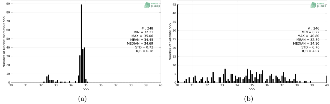
Figure 2: Histograms of SSS from Marine mammals (a) and SMOS SSS L2Q v331 - With FLAG (CMEMS-CATDS-CPDC) (b) considering all match-up pairs per bins of 0.1 over the North Atlantic Ocean Pi-MEP region and for the full satellite product period.
