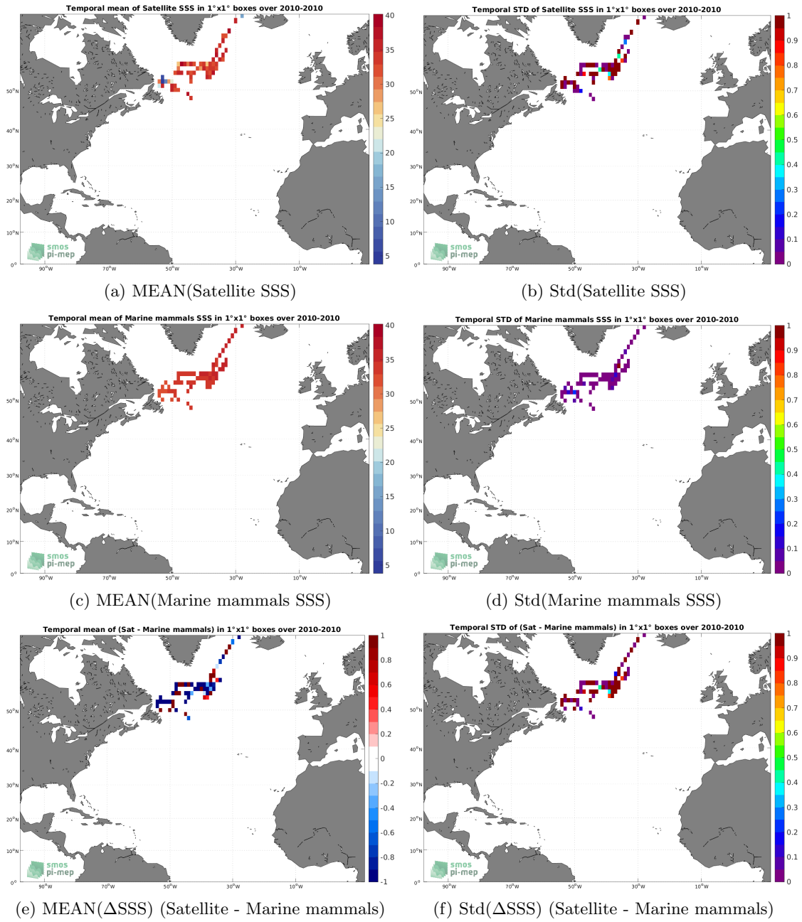
Figure 6: Temporal mean (left) and Std (right) of SSS from SMOS SSS L2Q v331 - With FLAG (CMEMS-CATDS-CPDC) (top), Marine mammals (middle), and of \Delta SSS (Satellite - Marine mammals). Only match-up pairs are used to generate these maps.
