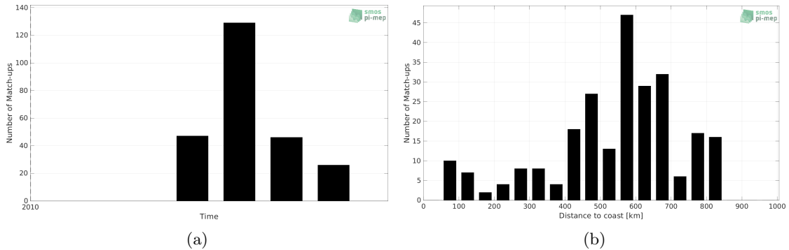
Figure 1: Number of match-ups between Marine mammals and SMOS SSS L2Q v331 - With FLAG (CMEMS-CATDS-CPDC) SSS as a function of time (a) and as function of the distance to coast (b) over the North Atlantic Ocean Pi-MEP region and for the full satellite product period.
