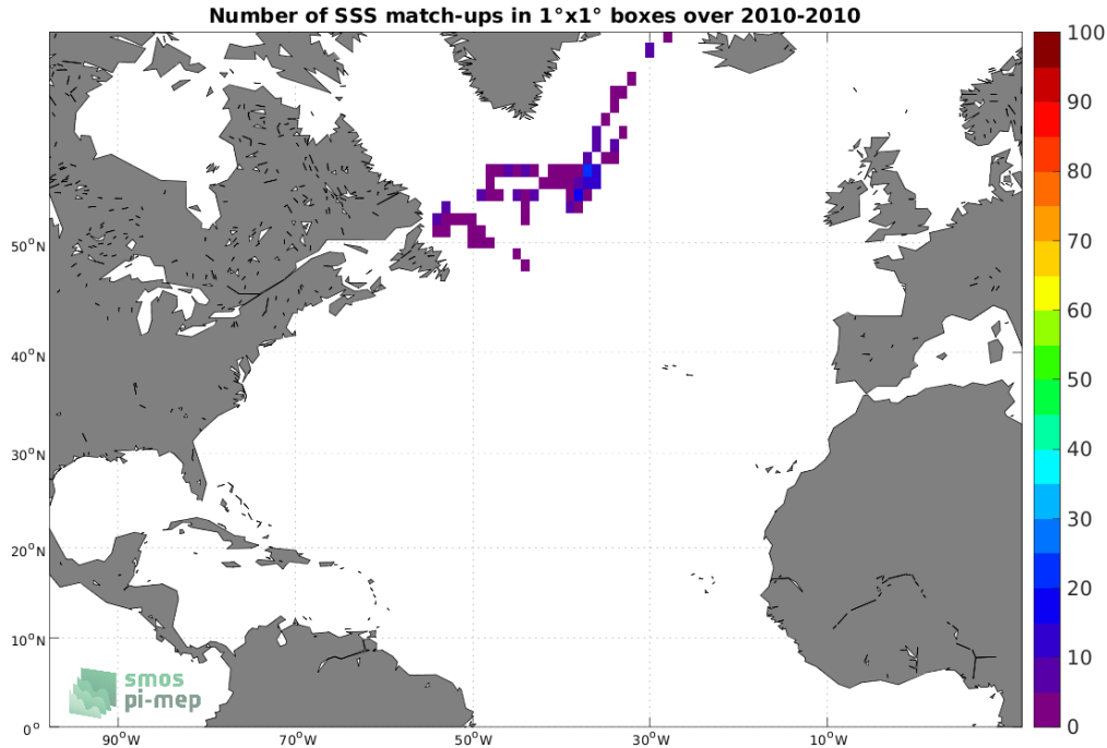
Figure 4: Number of SSS match-ups between Marine mammals SSS and the SMOS SSS L2Q v331 - With FLAG (CMEMS-CATDS-CPDC) SSS product for the North Atlantic Ocean Pi-MEP region over 1^\circ \times 1^\circ boxes and for the full satellite product period.
