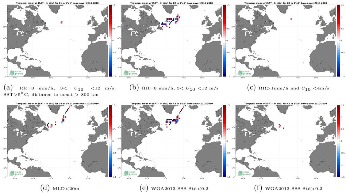
Figure 12: Temporal mean gridded over spatial boxes of size 1^{\circ}\times 1^{\circ} of \Delta\text{SSS} (SMOS SSS L2Q v331 - With FLAG (CMEMS-CATDS-CPDC) - Marine mammals) for 6 different subdatasets corresponding to:RR=0 mm/h, 3 < U_{10} < 12 m/s, SST >5^{\circ}\text{C} , distance to coast > 800 km (a), RR=0 mm/h, 3 < U_{10} < 12 m/s (b), RR >1\text{mm/h} and U_{10} < 4\text{m/s} (c),MLD <20\text{m} (d),WOA2013 SSS Std <0.2 (e),WOA2013 SSS Std >0.2 (f).
