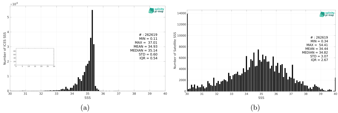
Figure 2: Histograms of SSS from ICES (a) and SMOS SSS L2Q v331 - With FLAG (CMEMS-CATDS-CPDC) (b) considering all match-up pairs per bins of 0.1 over the North Atlantic Ocean Pi-MEP region and for the full satellite product period.
