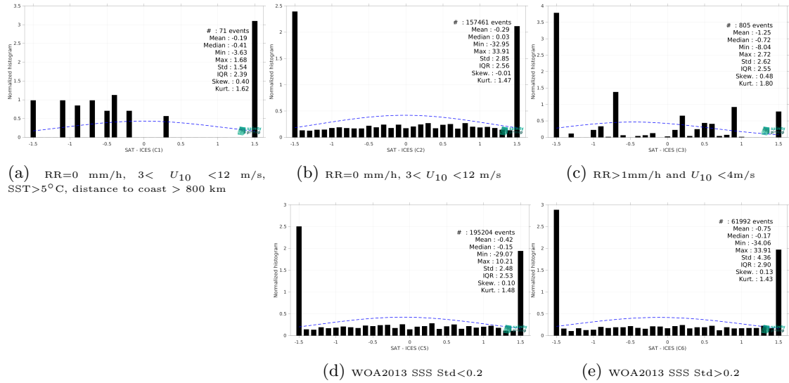
Figure 13: Normalized histogram of \Delta SSS (SMOS SSS L2Q v331 - With FLAG (CMEMS-CATDS-CPDC) - ICES) for 5 different subdatasets corresponding to: RR=0 mm/h, 3 < U_{10} < 12 m/s, SST>5°C, distance to coast > 800 km (a), RR=0 mm/h, 3 < U_{10} < 12 m/s (b), RR>1mm/h and U_{10} < 4 m/s (c), WOA2013 SSS Std<0.2 (d), WOA2013 SSS Std>0.2 (e).
