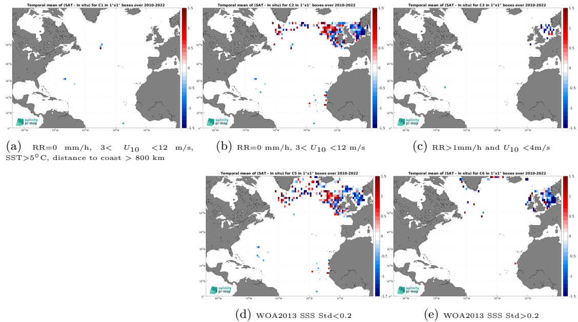
Figure 12: Temporal mean gridded over spatial boxes of size 1^\circ \times 1^\circ of \Delta\text{SSS} (SMOS SSS L2Q v331 - With FLAG (CMEMS-CATDS-CPDC) - ICES) for 5 different subdatasets corresponding to:RR=0 mm/h, 3 < U_{10} < 12 m/s, SST >5^\circ\text{C} , distance to coast > 800 km (a), RR=0 mm/h, 3 < U_{10} < 12 m/s (b), RR >1 mm/h and U_{10} < 4 m/s (c), WOA2013 SSS Std <0.2 (d), WOA2013 SSS Std >0.2 (e).
