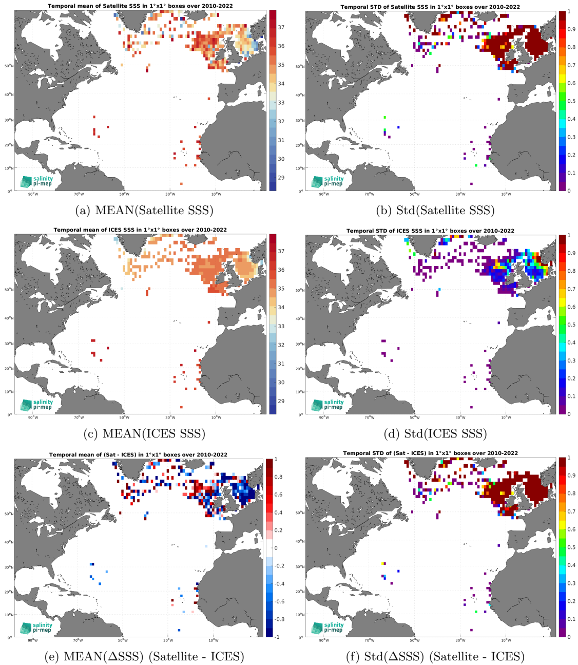
Figure 6: Temporal mean (left) and Std (right) of SSS from SMOS SSS L2Q v331 - With FLAG (CMEMS-CATDS-CPDC) (top), ICES (middle), and of \Delta SSS (Satellite - ICES). Only match-up pairs are used to generate these maps.
