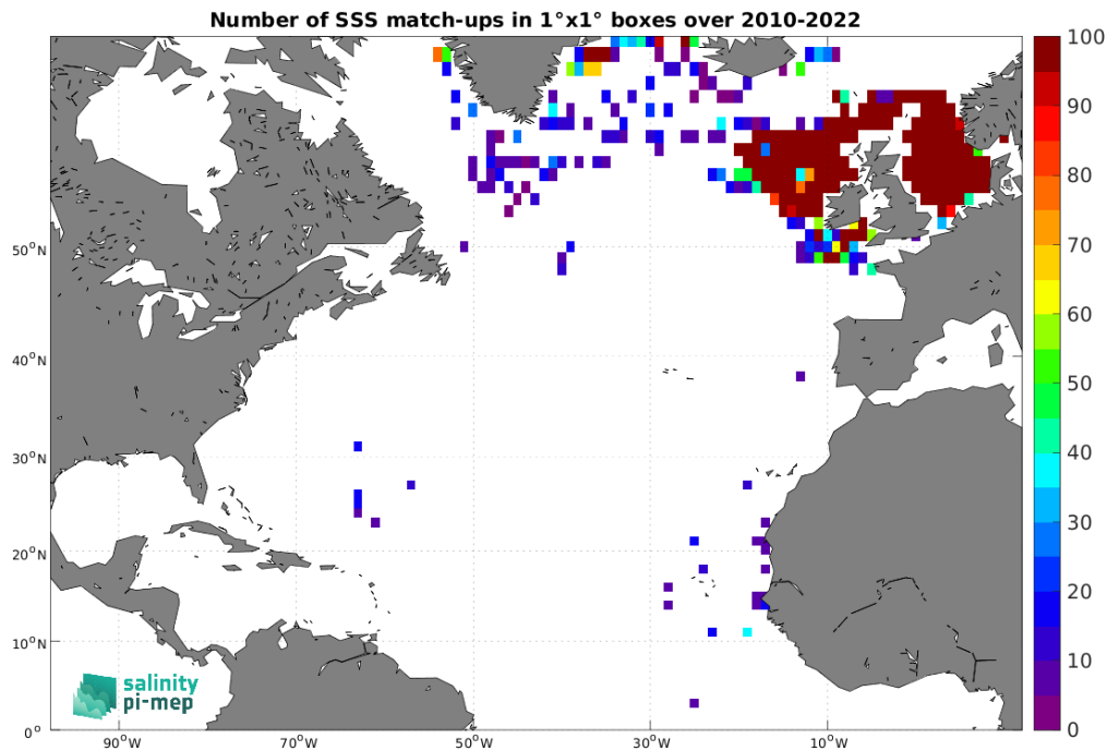
Figure 4: Number of SSS match-ups between ICES SSS and the SMOS SSS L2Q v331 - With FLAG (CMEMS-CATDS-CPDC) SSS product for the North Atlantic Ocean Pi-MEP region over 1^\circ \times 1^\circ boxes and for the full satellite product period.
