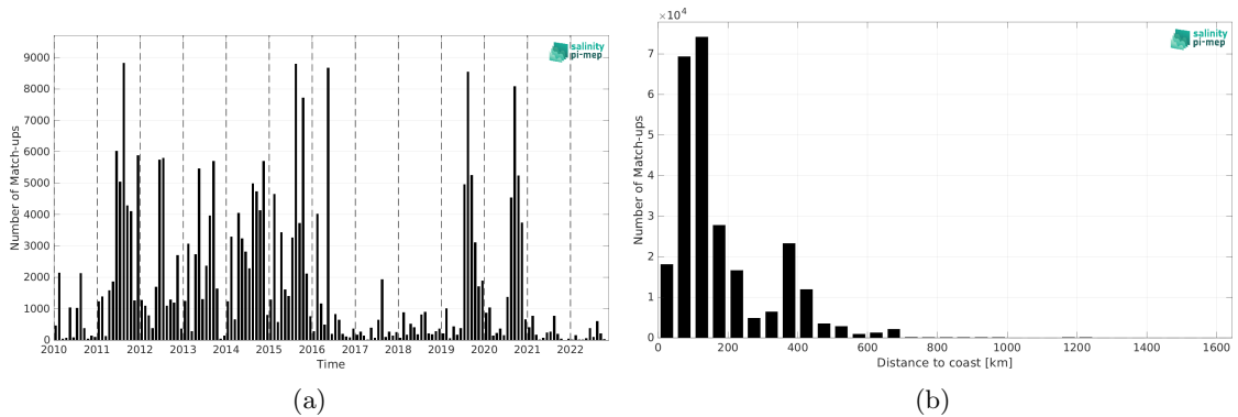
Figure 1: Number of match-ups between ICES and SMOS SSS L2Q v331 - With FLAG (CMEMS-CATDS-CPDC) SSS as a function of time (a) and as function of the distance to coast (b) over the North Atlantic Ocean Pi-MEP region and for the full satellite product period.
