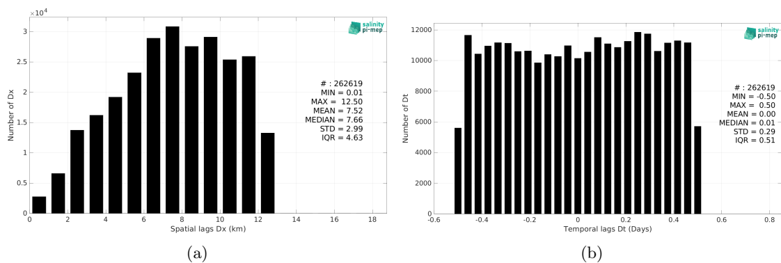
Figure 5: Histograms of the spatial (a) and temporal (b) lags between the location/time of the ICES measurement and the date of the corresponding SMOS SSS L2Q v331 - With FLAG (CMEMS-CATDS-CPDC) SSS pixel.
