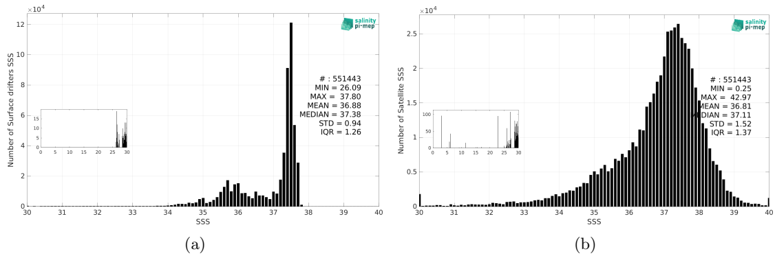
Figure 3: Histograms of SSS from Surface drifters (a) and SMOS SSS L2Q v331 - With FLAG (CMEMS-CATDS-CPDC) (b) considering all match-up pairs per bins of 0.1 over the North Atlantic Ocean Pi-MEP region and for the full satellite product period.
