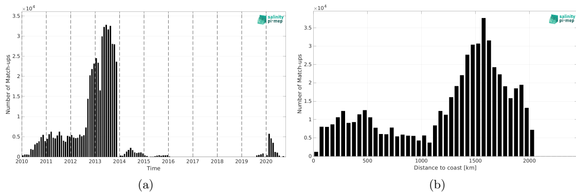
Figure 2: Number of match-ups between Surface drifters and SMOS SSS L2Q v331 - With FLAG (CMEMS-CATDS-CPDC) SSS as a function of time (a) and as function of the distance to coast (b) over the North Atlantic Ocean Pi-MEP region and for the full satellite product period.
