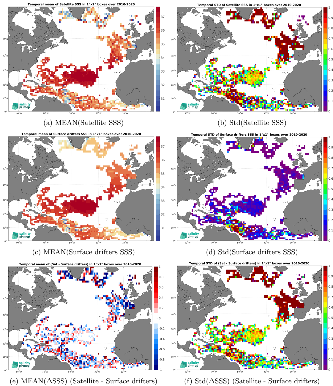
Figure 6: Temporal mean (left) and Std (right) of SSS from SMOS SSS L2Q v331 - With FLAG (CMEMS-CATDS-CPDC) (top), Surface drifters (middle), and of \Delta SSS (Satellite - Surface drifters). Only match-up pairs are used to generate these maps.
