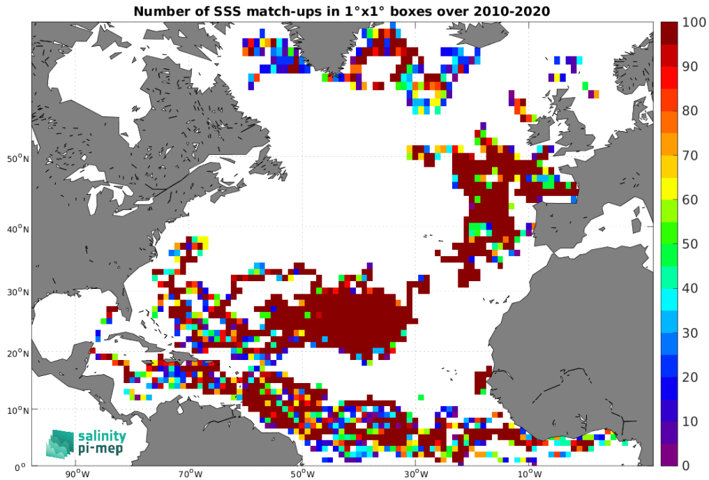
Figure 4: Number of SSS match-ups between Surface drifters SSS and the SMOS SSS L2Q v331 - With FLAG (CMEMS-CATDS-CPDC) SSS product for the North Atlantic Ocean Pi-MEP region over 1^\circ \times 1^\circ boxes and for the full satellite product period.
