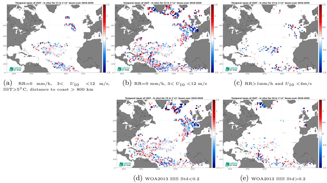
Figure 13: Temporal mean gridded over spatial boxes of size 1^\circ \times 1^\circ of \Delta\text{SSS} (SMOS SSS L2Q v331 - With FLAG (CMEMS-CATDS-CPDC) - Surface drifters) for 5 different subdatasets corresponding to:RR=0 mm/h, 3 < U_{10} < 12 m/s, SST >5^\circ\text{C} , distance to coast > 800 km (a), RR=0 mm/h, 3 < U_{10} < 12 m/s (b), RR >1 mm/h and U_{10} < 4 m/s (c), WOA2013 SSS Std <0.2 (d), WOA2013 SSS Std >0.2 (e).
