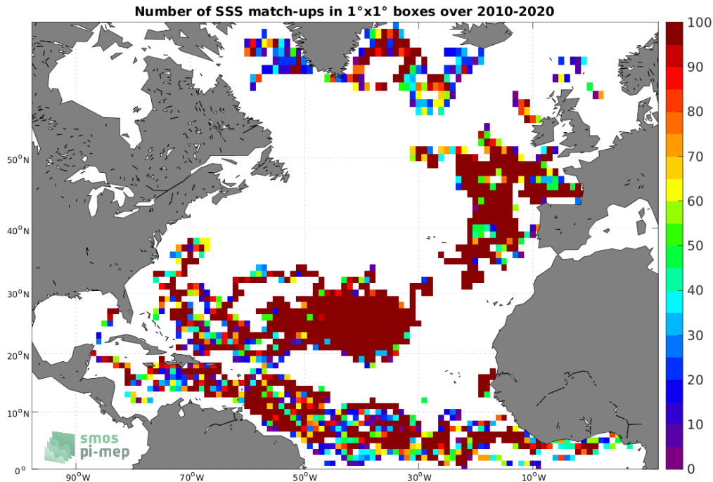
Figure 3: Number of SSS match-ups between Surface drifters SSS and the SMOS SSS L2Q v331 - With FLAG (CMEMS-CATDS-CPDC) SSS product for the North Atlantic Ocean Pi-MEP region over 1^\circ \times 1^\circ boxes and for the full satellite product period.
