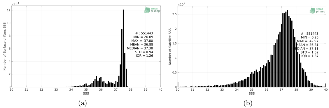
Figure 2: Histograms of SSS from Surface drifters (a) and SMOS SSS L2Q v331 - With FLAG (CMEMS-CATDS-CPDC) (b) considering all match-up pairs per bins of 0.1 over the North Atlantic Ocean Pi-MEP region and for the full satellite product period.
