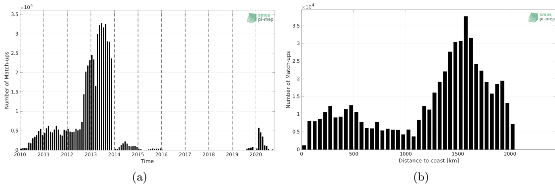
Figure 1: Number of match-ups between Surface drifters and SMOS SSS L2Q v331 - With FLAG (CMEMS-CATDS-CPDC) SSS as a function of time (a) and as function of the distance to coast (b) over the North Atlantic Ocean Pi-MEP region and for the full satellite product period.
