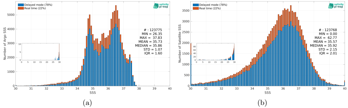
Figure 3: Histograms of SSS from Argo (a) and SMOS SSS L2Q v331 - With FLAG (CMEMS-CATDS-CPDC) (b) considering all match-up pairs per bins of 0.1 over the North Atlantic Ocean Pi-MEP region and for the full satellite product period.
