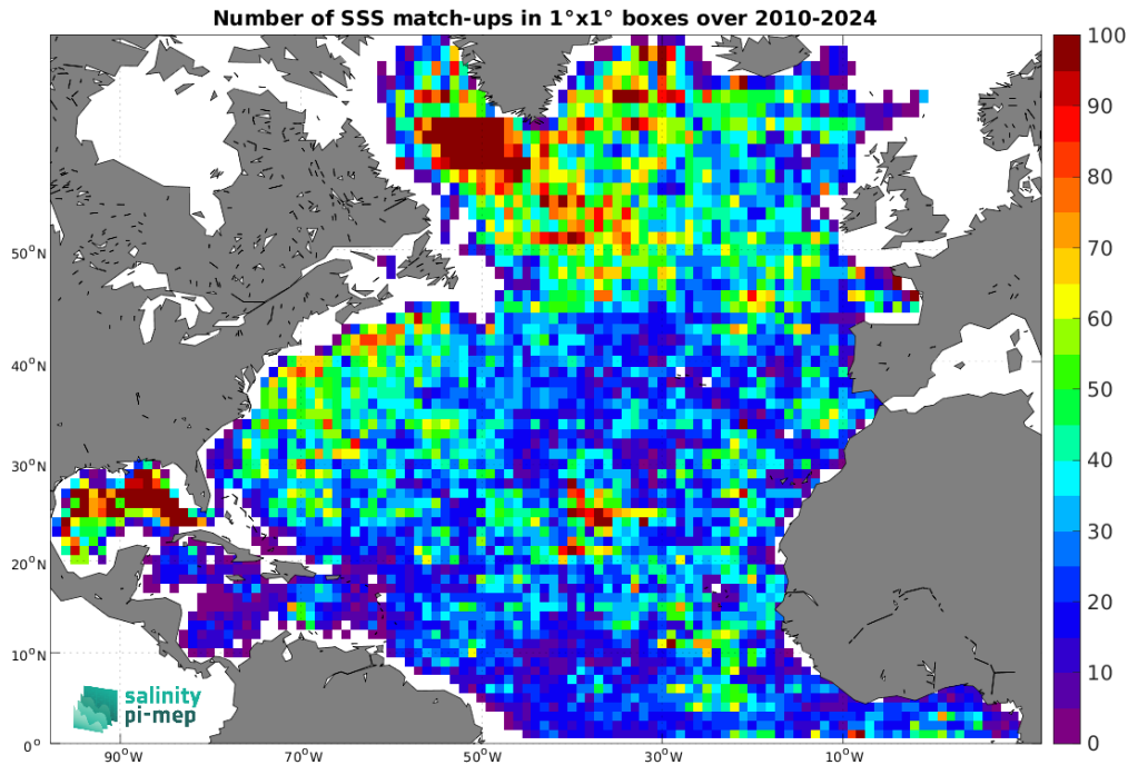
Figure 5: Number of SSS match-ups between Argo SSS and the SMOS SSS L2Q v331 - With FLAG (CMEMS-CATDS-CPDC) SSS product for the North Atlantic Ocean Pi-MEP region over 1^\circ \times 1^\circ boxes and for the full satellite product period.
