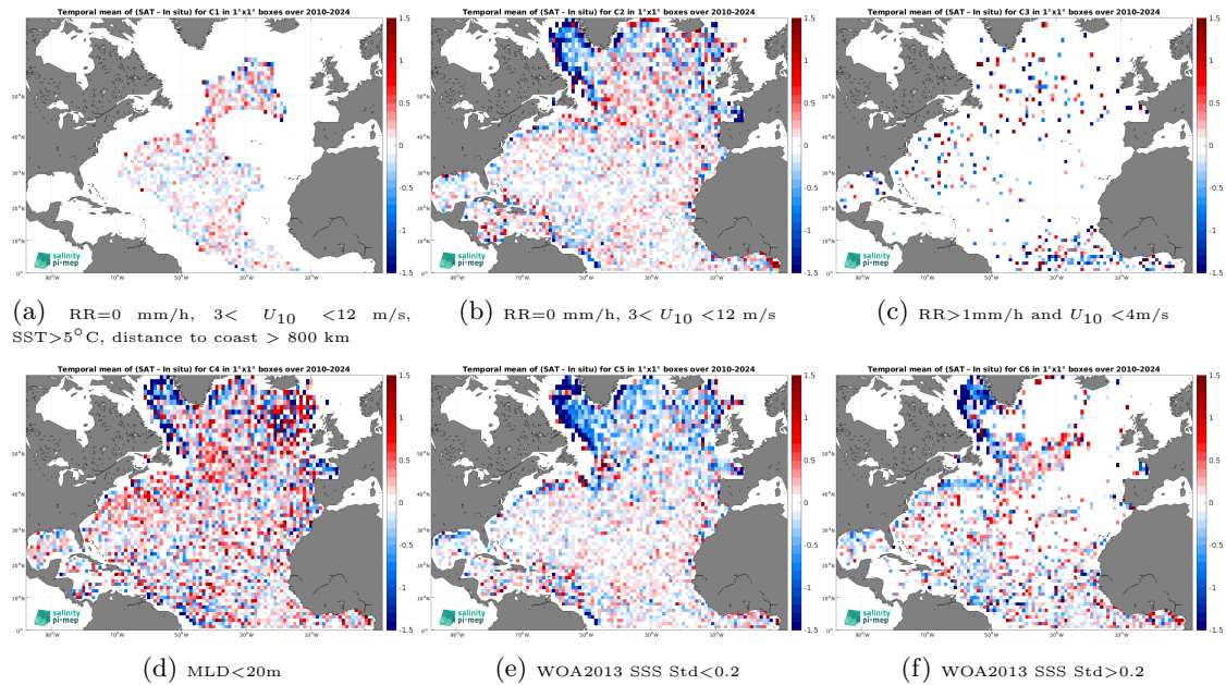
Figure 14: Temporal mean gridded over spatial boxes of size 1^\circ \times 1^\circ of \Delta SSS (SMOS SSS L2Q v331 - With FLAG (CMEMS-CATDS-CPDC) - Argo) for 6 different subdatasets corresponding to:RR=0 mm/h, 3 < U_{10} < 12 m/s, SST > 5^\circ\text{C} , distance to coast > 800 km (a), RR=0 mm/h, 3 < U_{10} < 12 m/s (b), RR > 1 mm/h and U_{10} < 4 m/s (c),MLD < 20 m (d),WOA2013 SSS Std < 0.2 (e),WOA2013 SSS Std > 0.2 (f).
