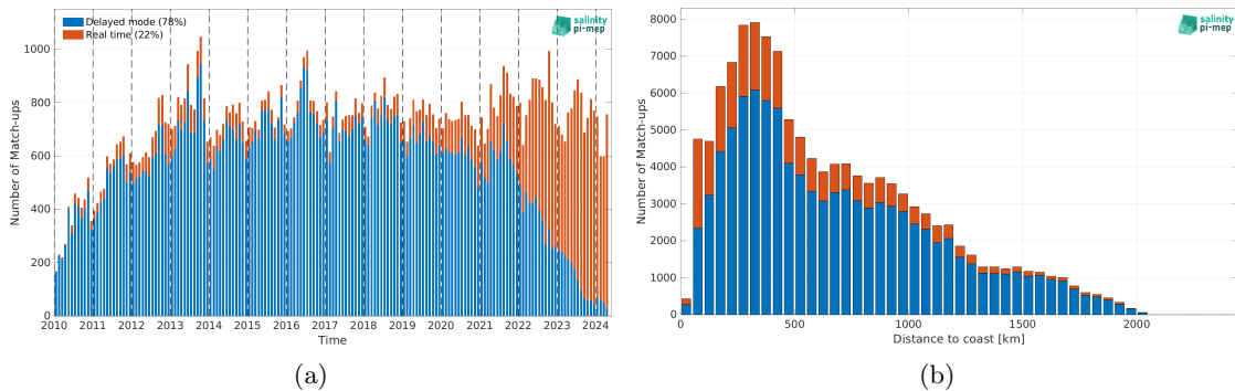
Figure 2: Number of match-ups between Argo and SMOS SSS L2Q v331 - With FLAG (CMEMS-CATDS-CPDC) SSS as a function of time (a) and as function of the distance to coast (b) over the North Atlantic Ocean Pi-MEP region and for the full satellite product period.
