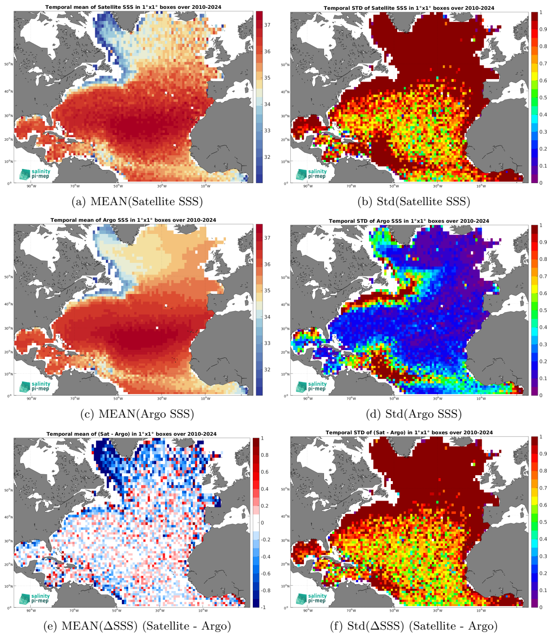
Figure 7: Temporal mean (left) and Std (right) of SSS from SMOS SSS L2Q v331 - With FLAG (CMEMS-CATDS-CPDC) (top), Argo (middle), and of \Delta SSS (Satellite - Argo). Only match-up pairs are used to generate these maps.
