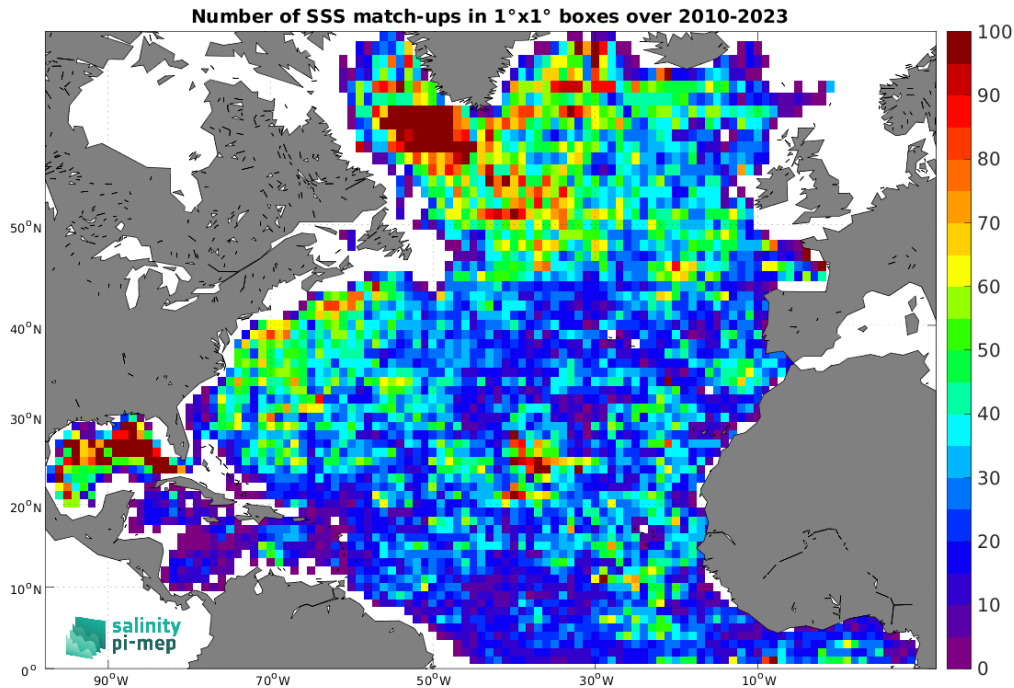
Figure 4: Number of SSS match-ups between Argo SSS and the SMOS SSS L2Q v331 - With FLAG (CMEMS-CATDS-CPDC) SSS product for the North Atlantic Ocean Pi-MEP region over 1^\circ \times 1^\circ boxes and for the full satellite product period.
