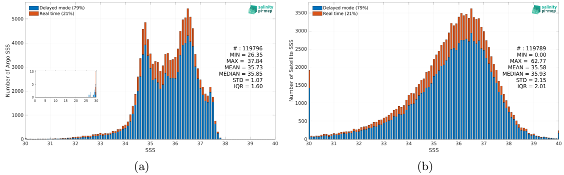
Figure 2: Histograms of SSS from Argo (a) and SMOS SSS L2Q v331 - With FLAG (CMEMS-CATDS-CPDC) (b) considering all match-up pairs per bins of 0.1 over the North Atlantic Ocean Pi-MEP region and for the full satellite product period.
