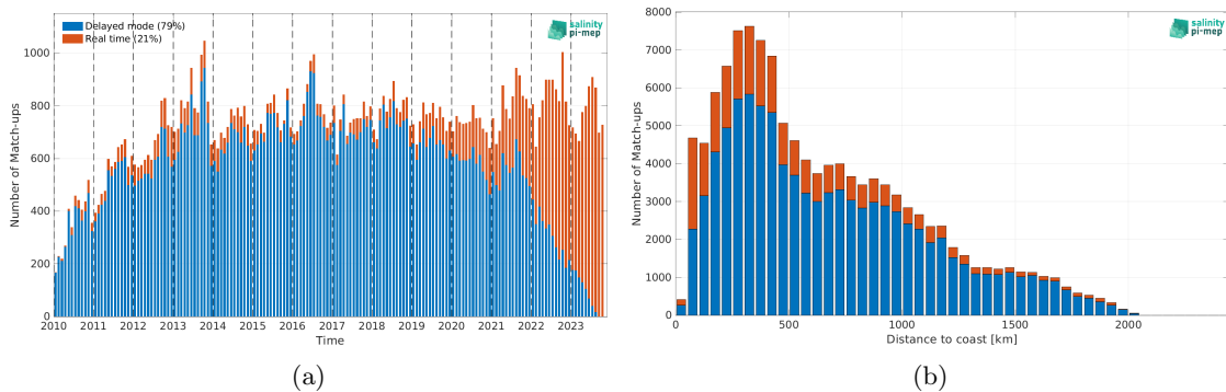
Figure 1: Number of match-ups between Argo and SMOS SSS L2Q v331 - With FLAG (CMEMS-CATDS-CPDC) SSS as a function of time (a) and as function of the distance to coast (b) over the North Atlantic Ocean Pi-MEP region and for the full satellite product period.
